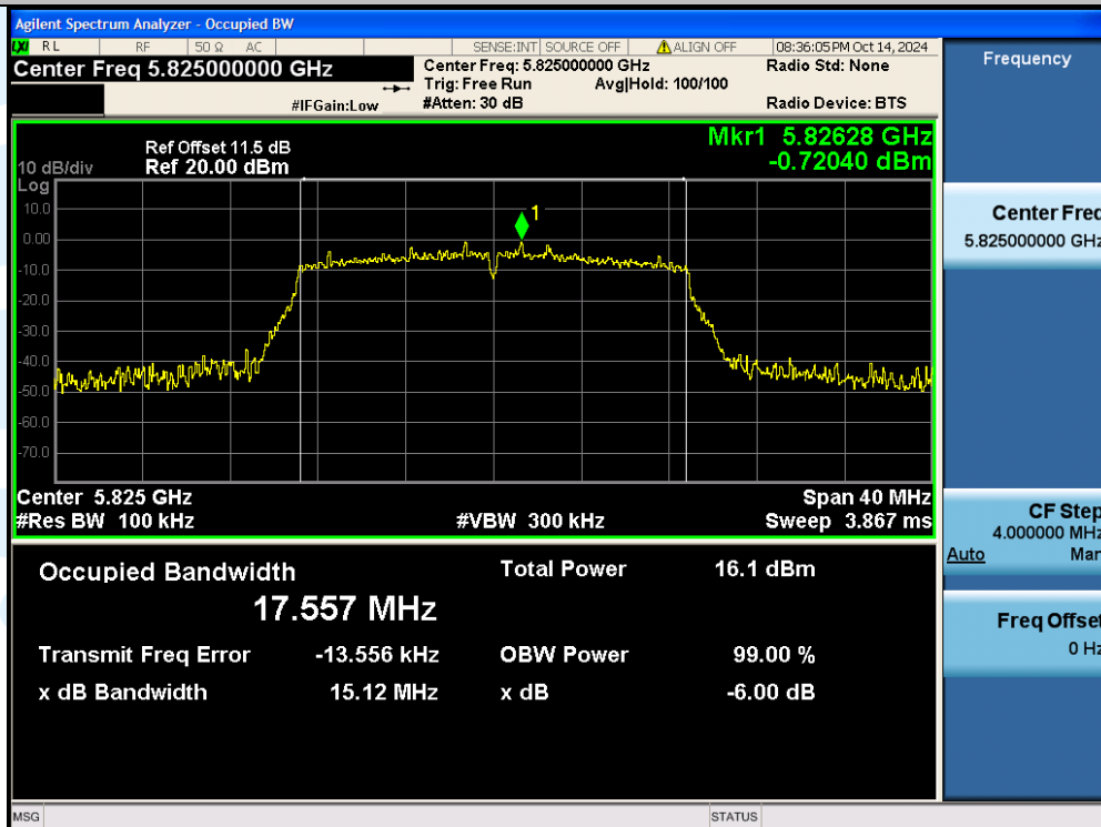
11AC20SISO-Ant1-5825-PASS
