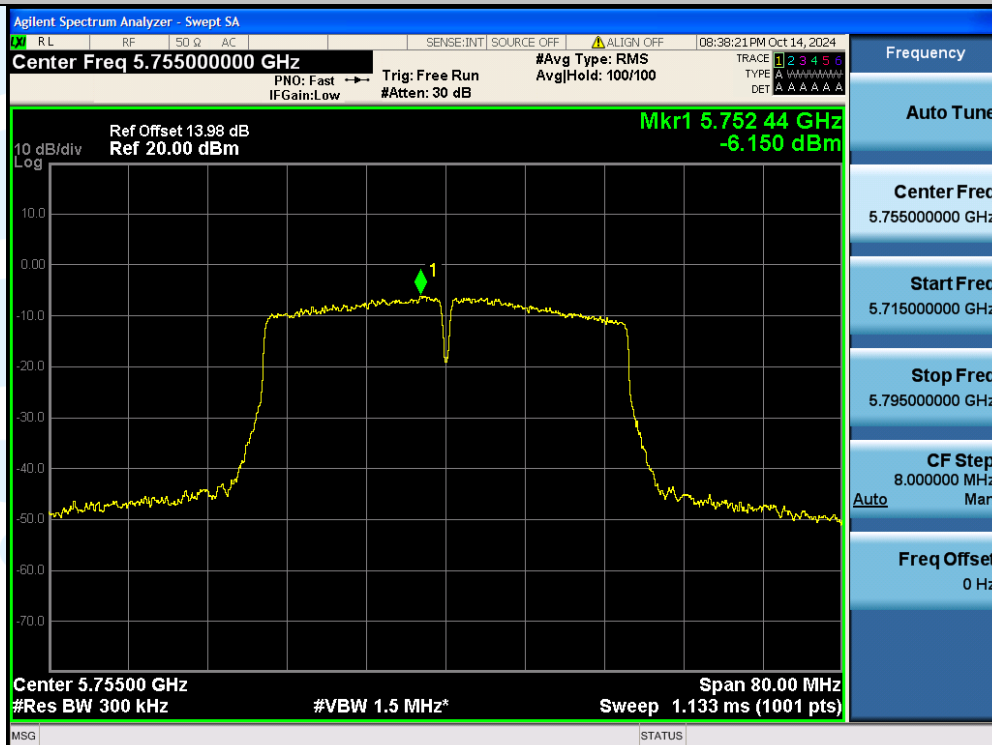
11AC40SISO-Ant1-5755-PASS
