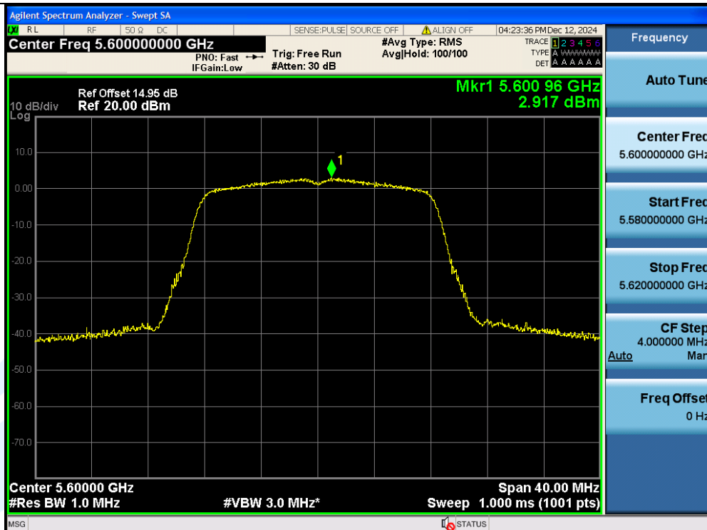
11A-Ant1-5600-PASS
