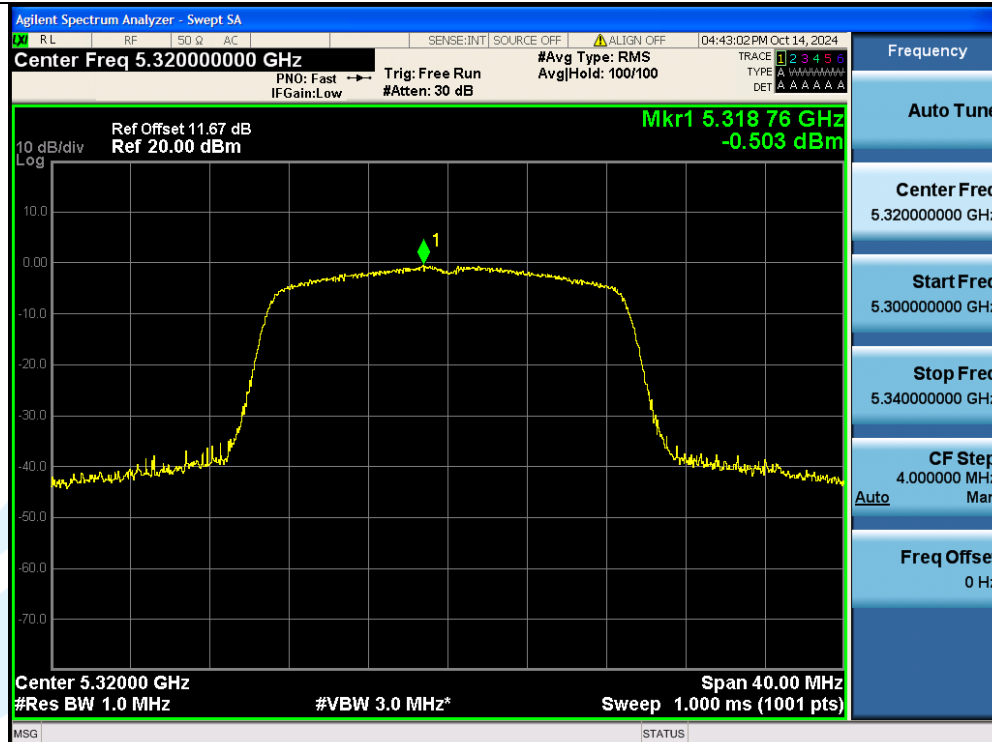
11N20SISO-Ant1-5320-PASS
