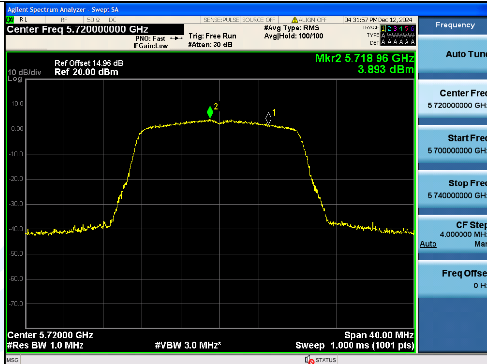
11A-Ant1-5720 UNII-2C-PASS
