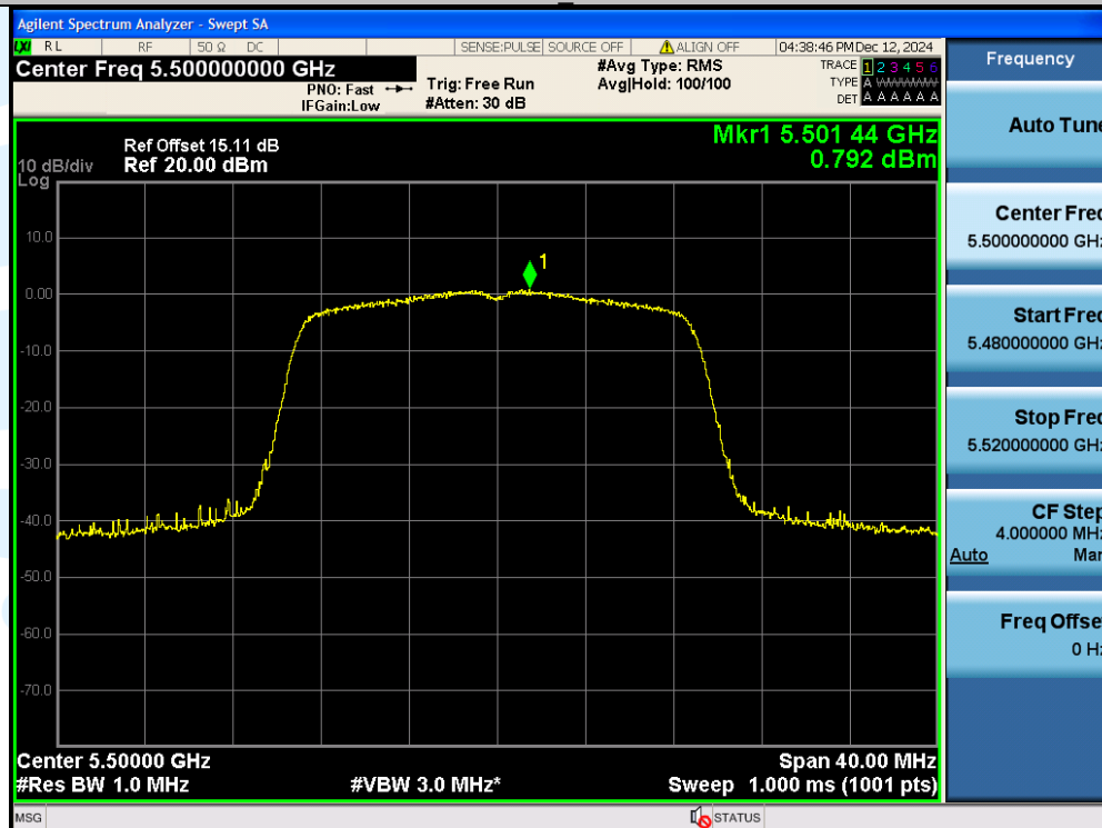
11N20SISO-Ant1-5500-PASS
