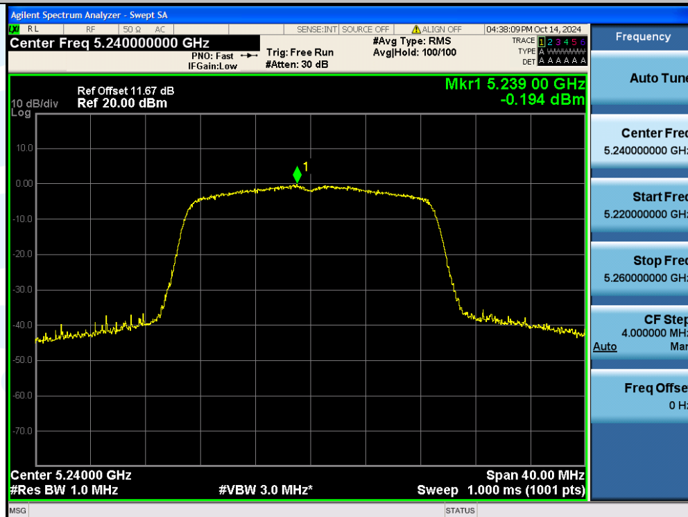
11N20SISO-Ant1-5240-PASS
