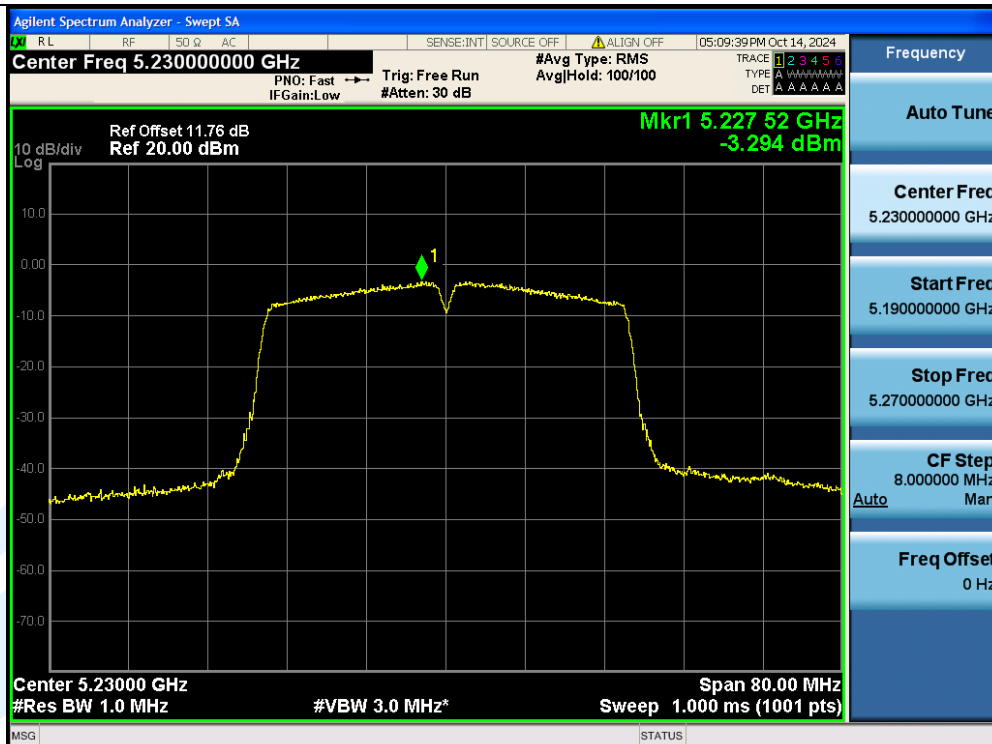
11AC40SISO-Ant1-5230-PASS
