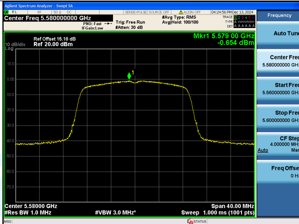
11AC20SISO-Ant1-5580-PASS
