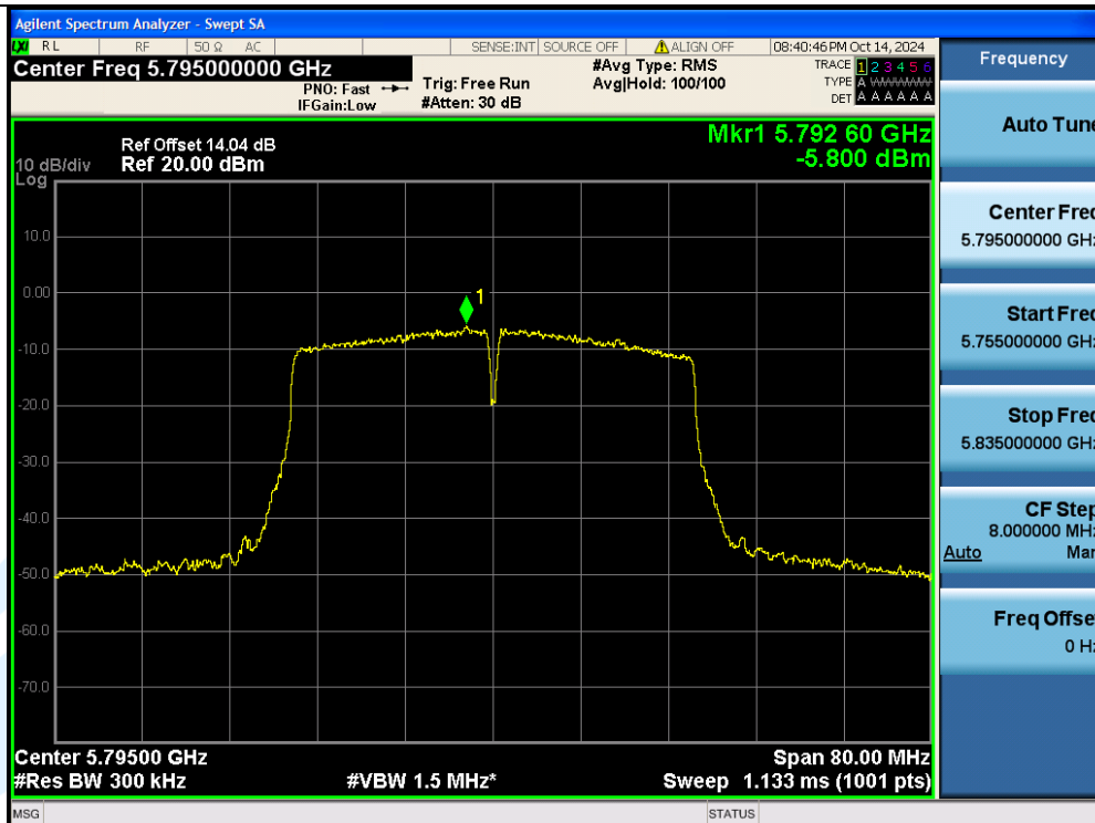
11AC40SISO-Ant1-5795-PASS
