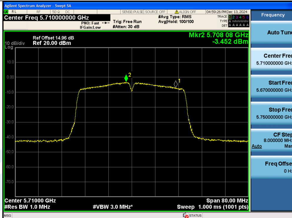
11AC40SISO-Ant1-5710_UNII-2C-PASS
