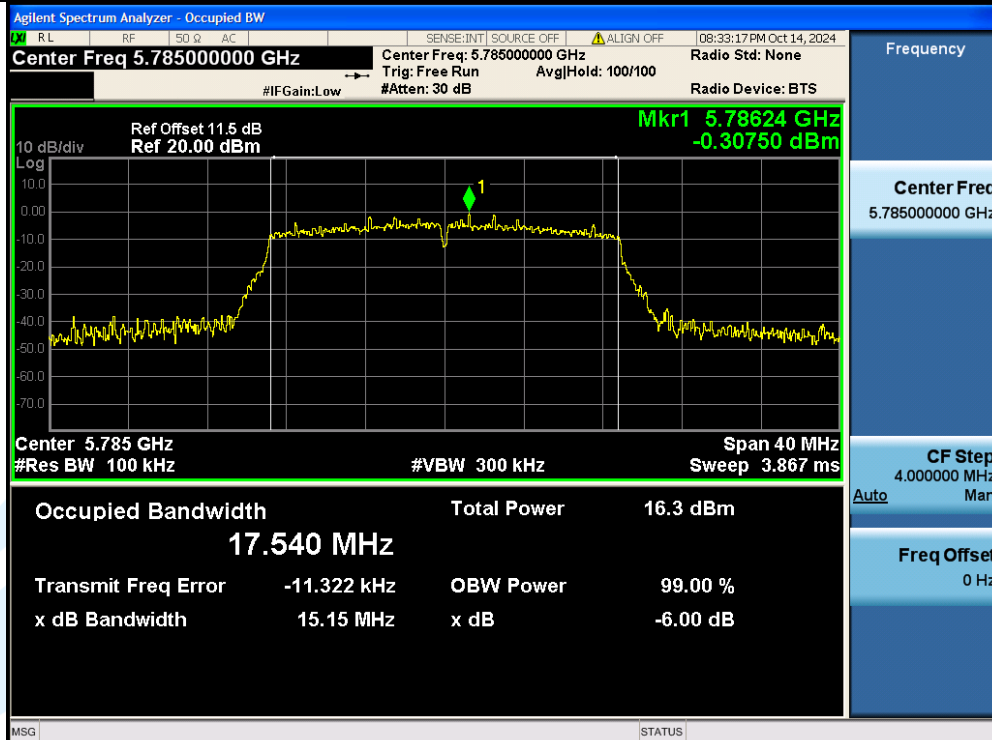
11AC20SISO-Ant1-5785-PASS
