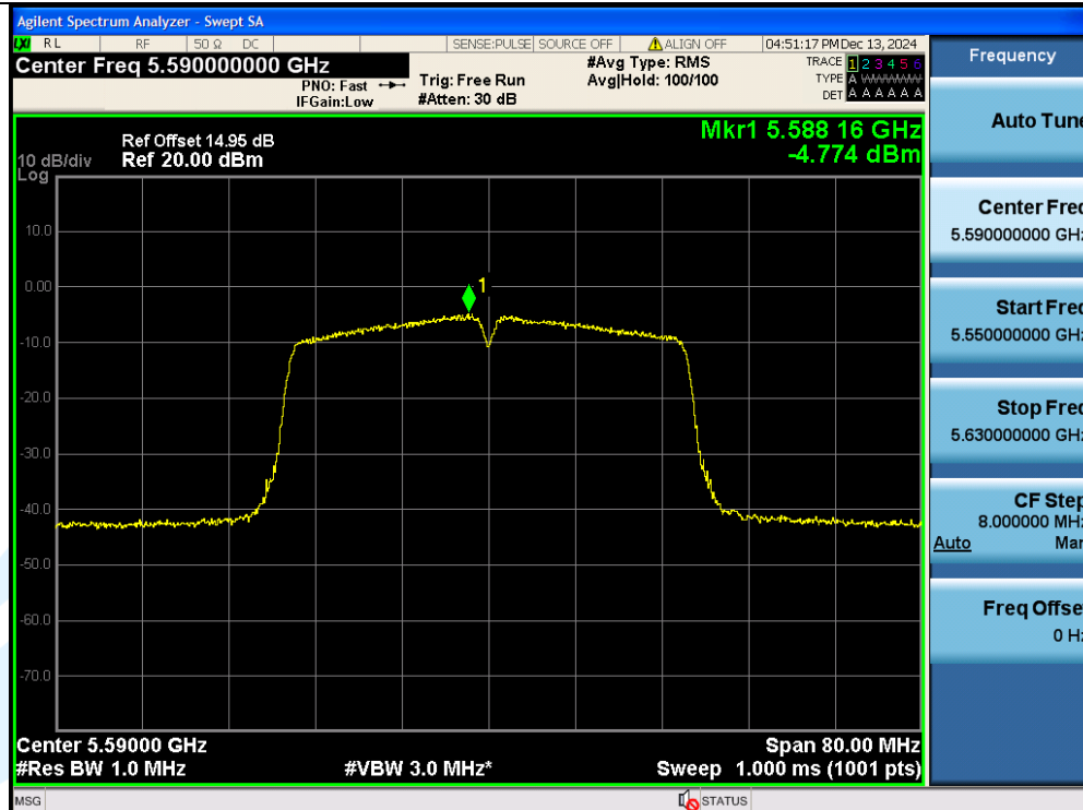
11AC40SISO-Ant1-5590-PASS
