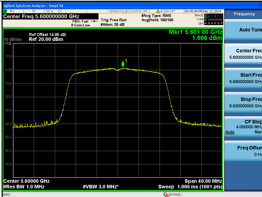
11N20SISO-Ant1-5600-PASS
