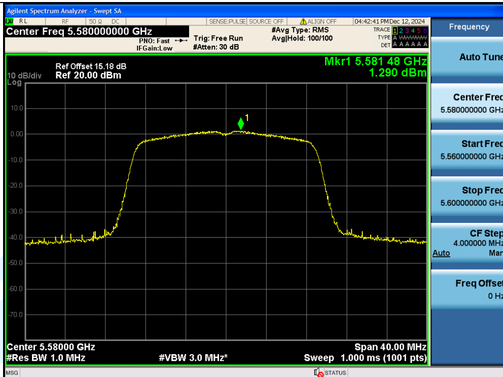
11N20SISO-Ant1-5580-PASS
