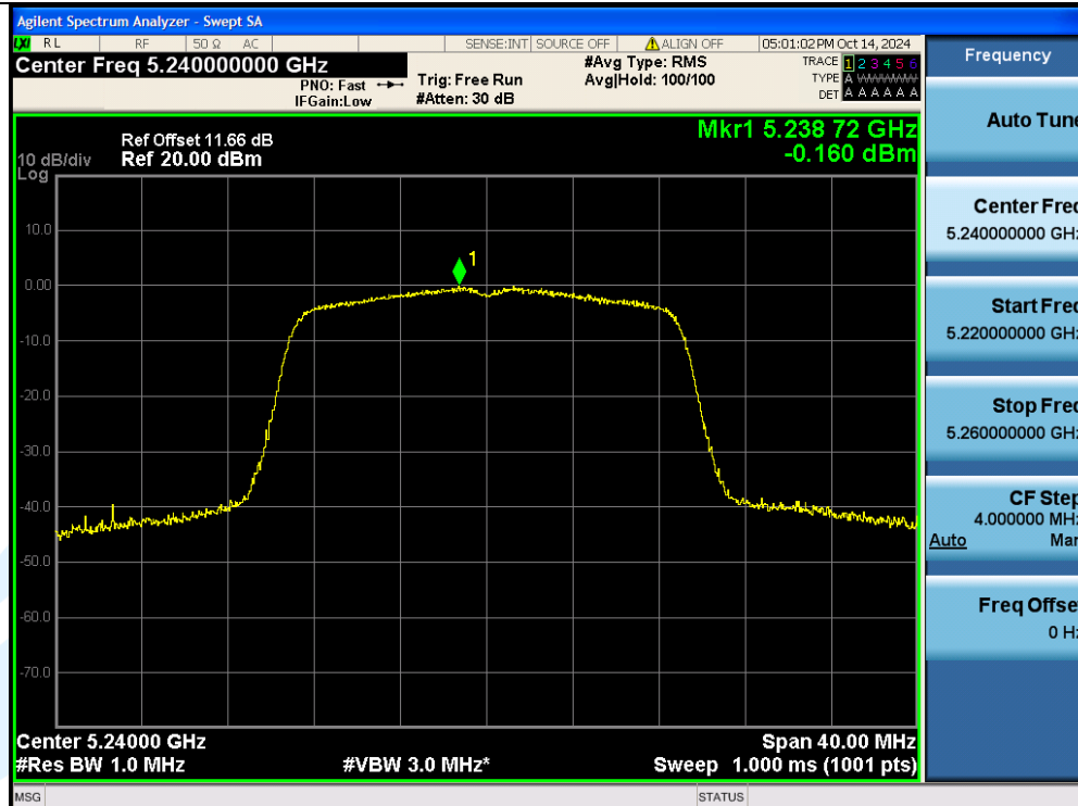
11AC20SISO-Ant1-5240-PASS
