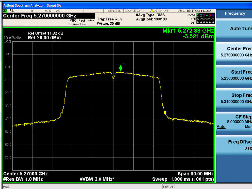
11AC40SISO-Ant1-5270-PASS
