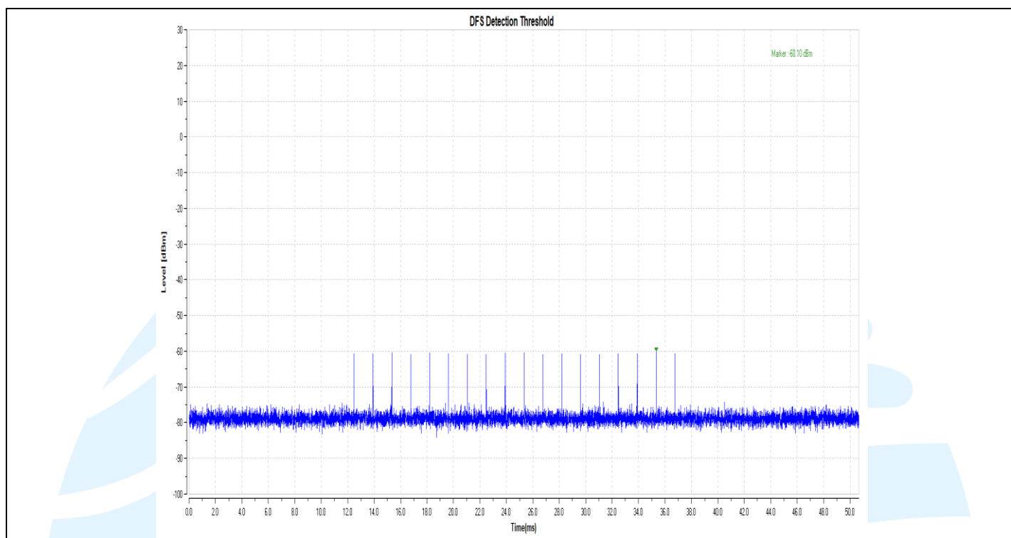
11AC20SISO-5300-Type0-PASS
