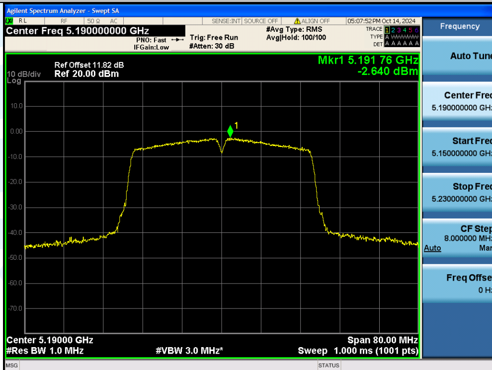
11AC40SISO-Ant1-5190-PASS
