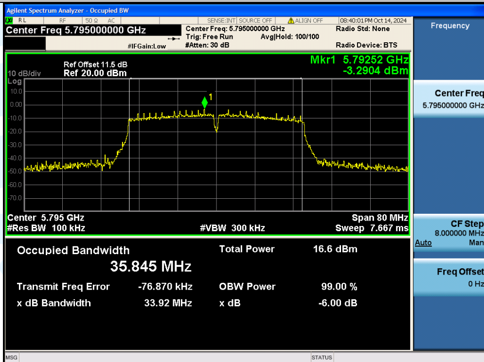
11AC40SISO-Ant1-5795-PASS
