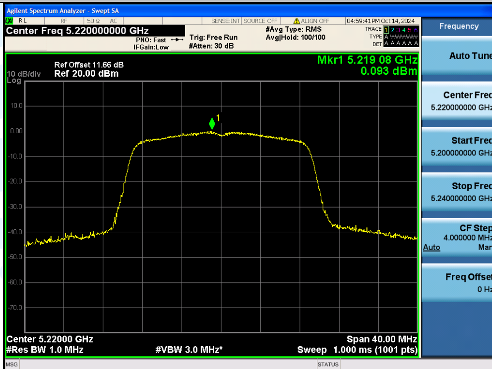
11AC20SISO-Ant1-5220-PASS
