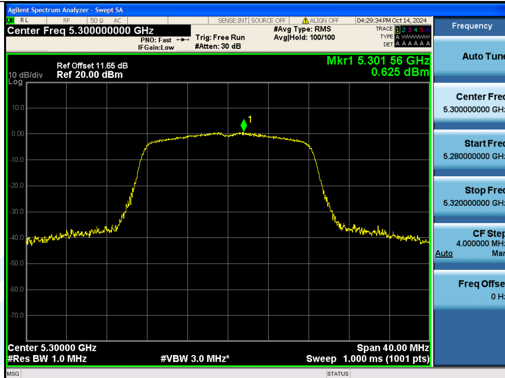
11A-Ant1-5300-PASS
