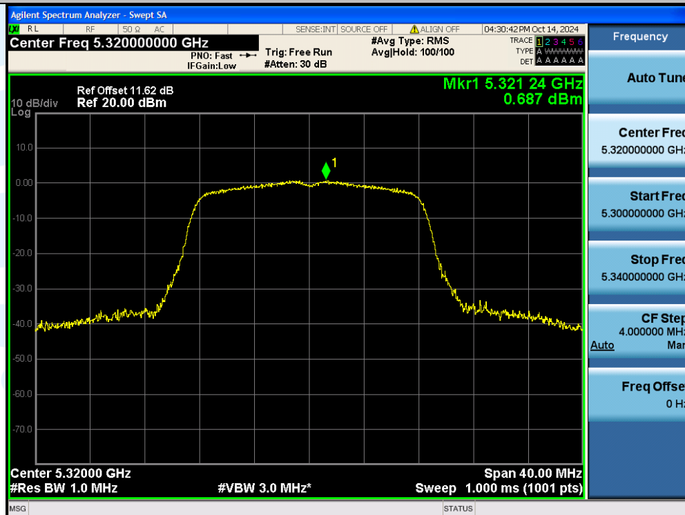
11A-Ant1-5320-PASS
