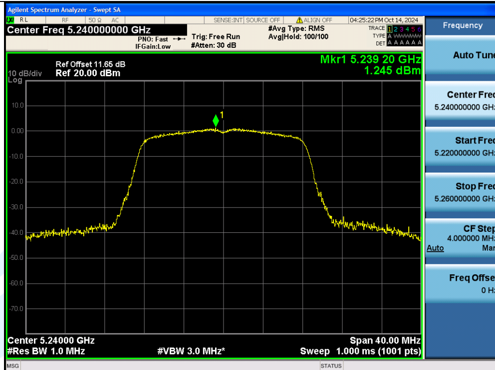
11A-Ant1-5240-PASS
