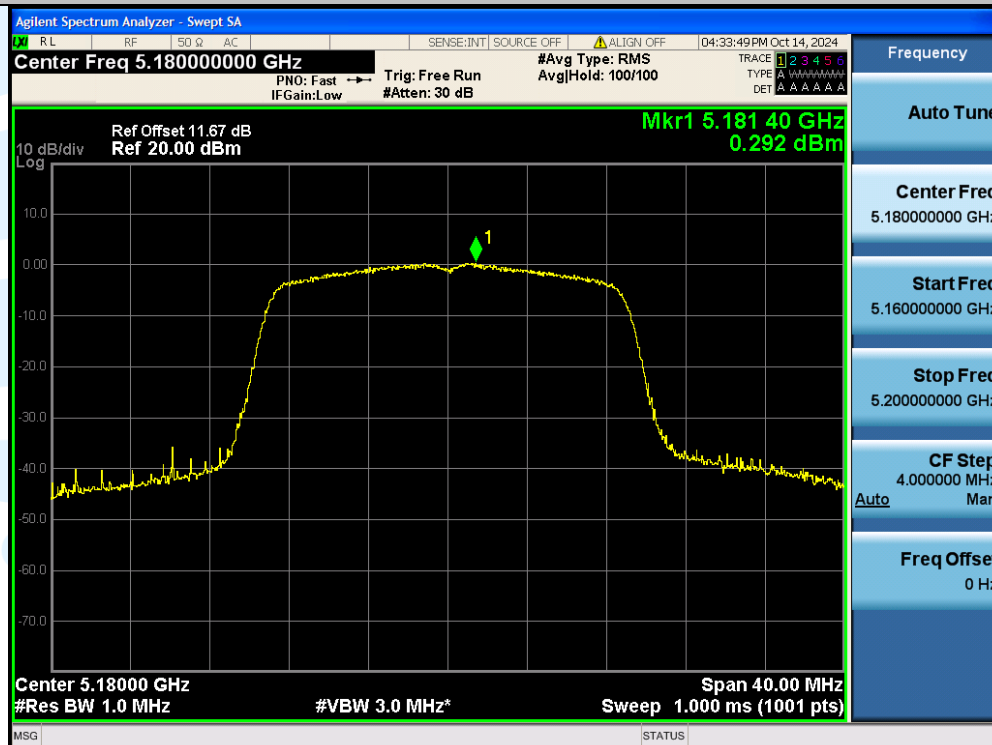
11N20SISO-Ant1-5180-PASS
