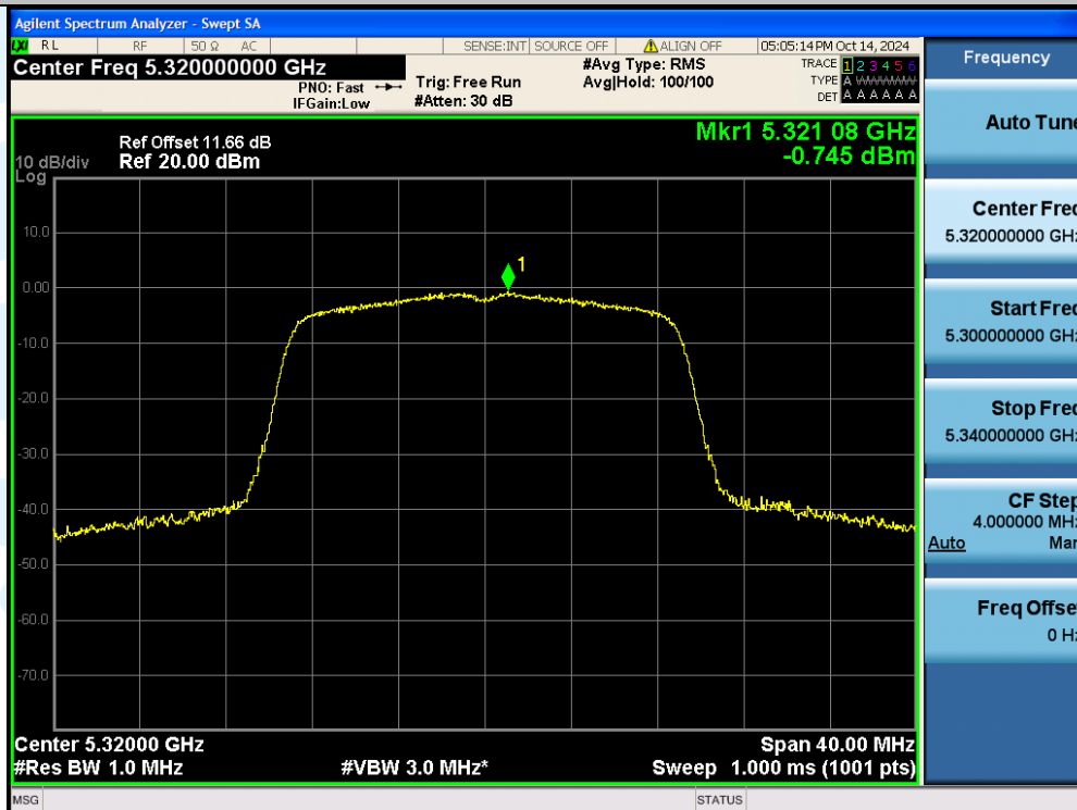
11AC20SISO-Ant1-5320-PASS
