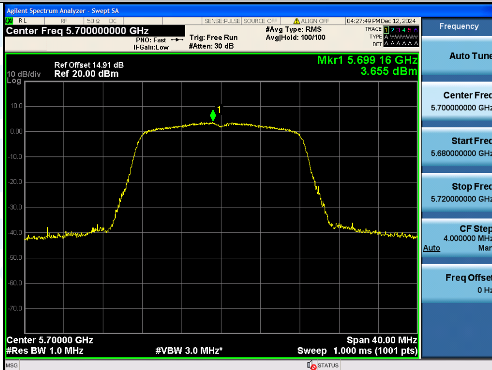
11A-Ant1-5700-PASS
