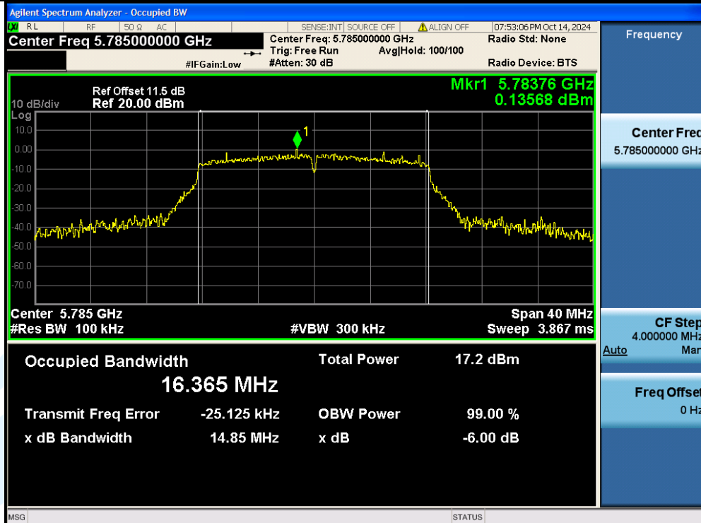
11A-Ant1-5785-PASS
