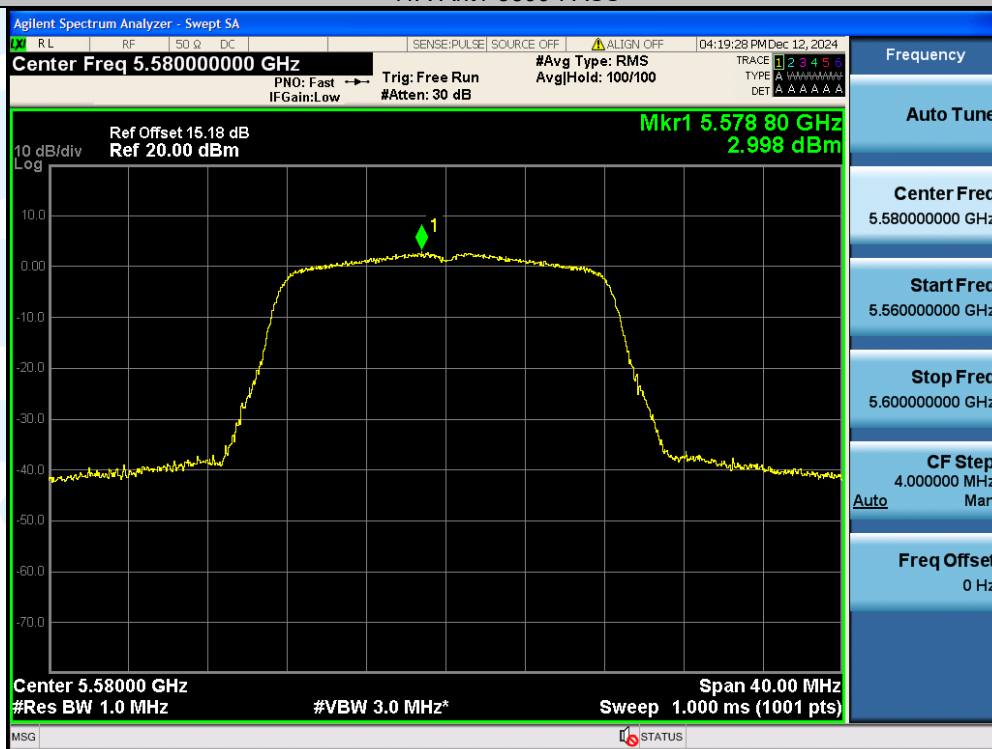
11A-Ant1-5580-PASS
