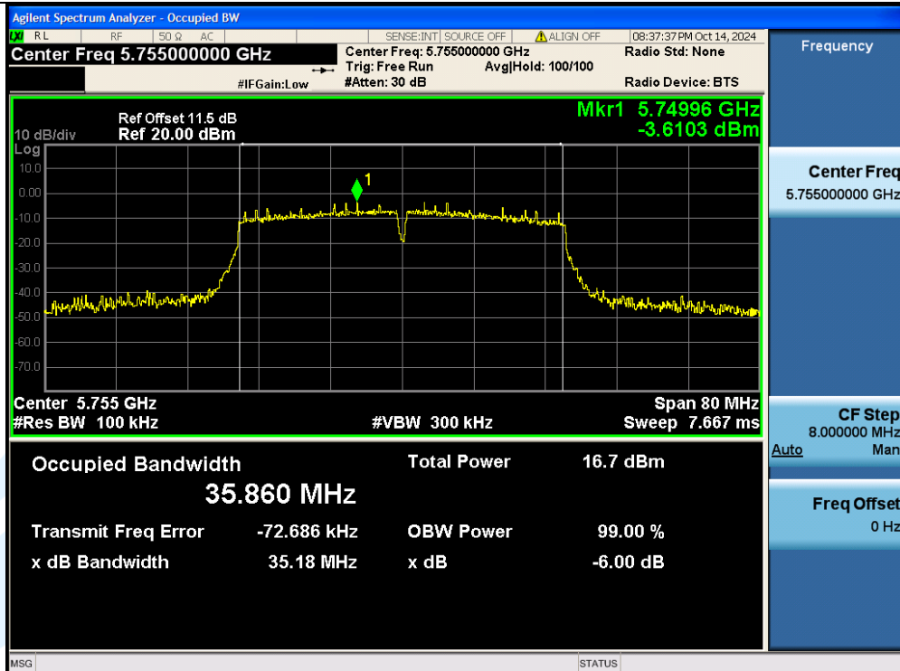
11AC40SISO-Ant1-5755-PASS
