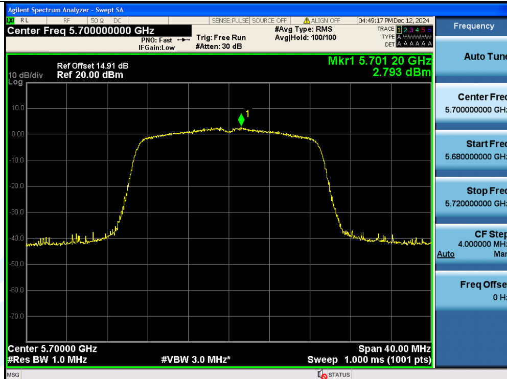
11N20SISO-Ant1-5700-PASS
