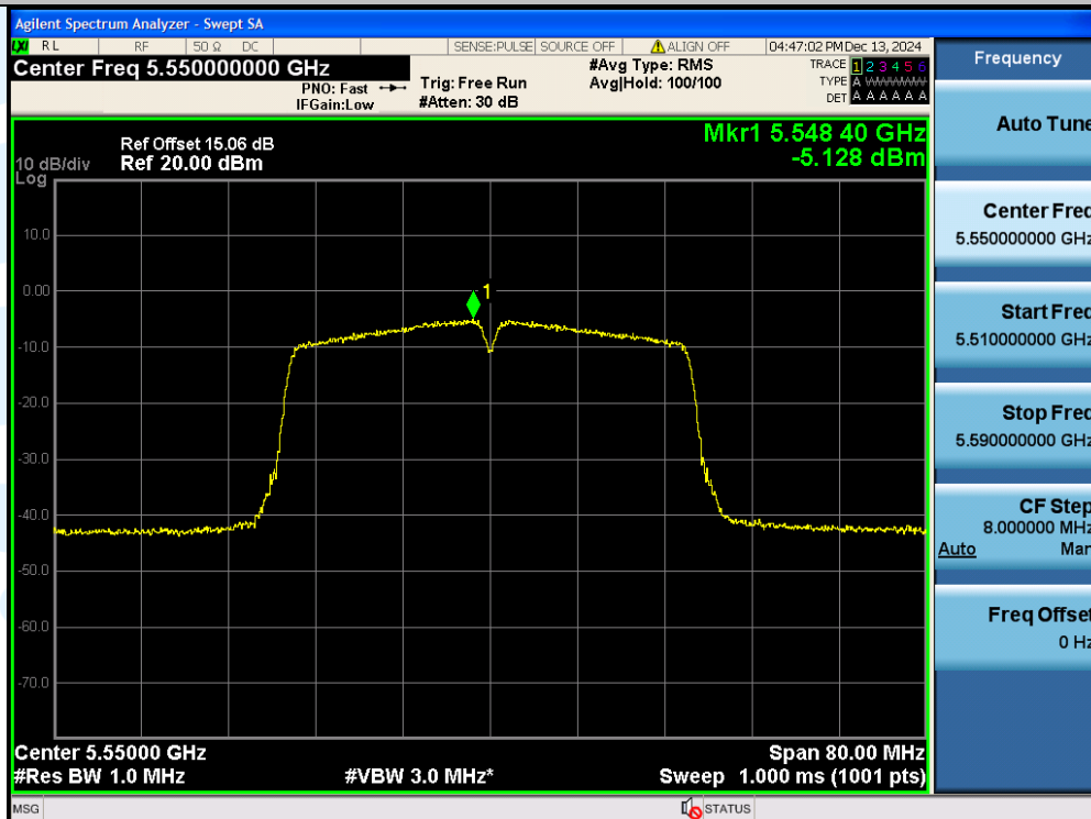
11AC40SISO-Ant1-5550-PASS
