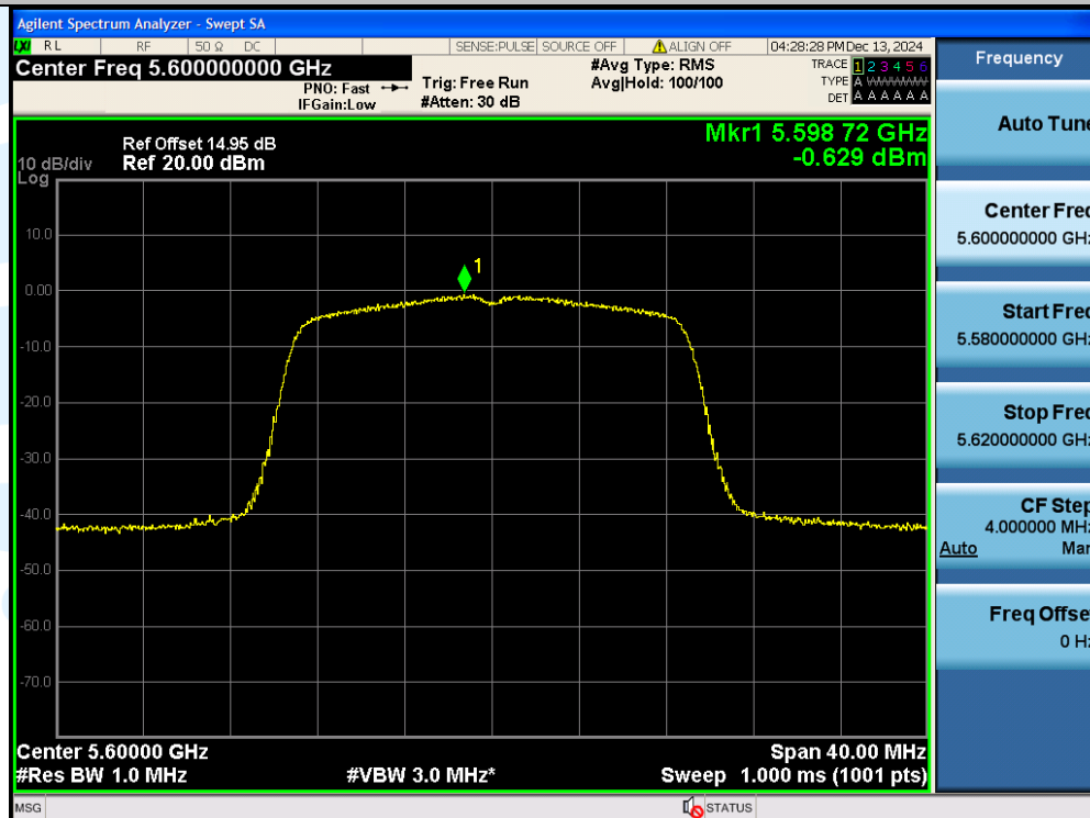
11AC20SISO-Ant1-5600-PASS
