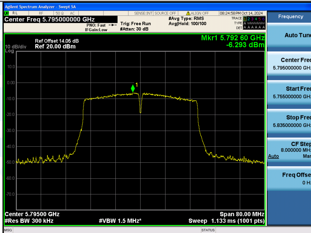
11N40SISO-Ant1-5795-PASS
