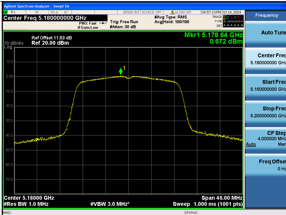
11AC20SISO-Ant1-5180-PASS
