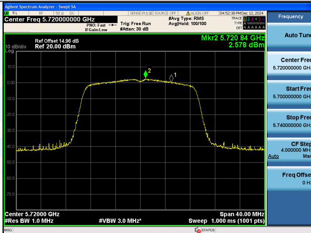
11N20SISO-Ant1-5720_UNII-2C-PASS
