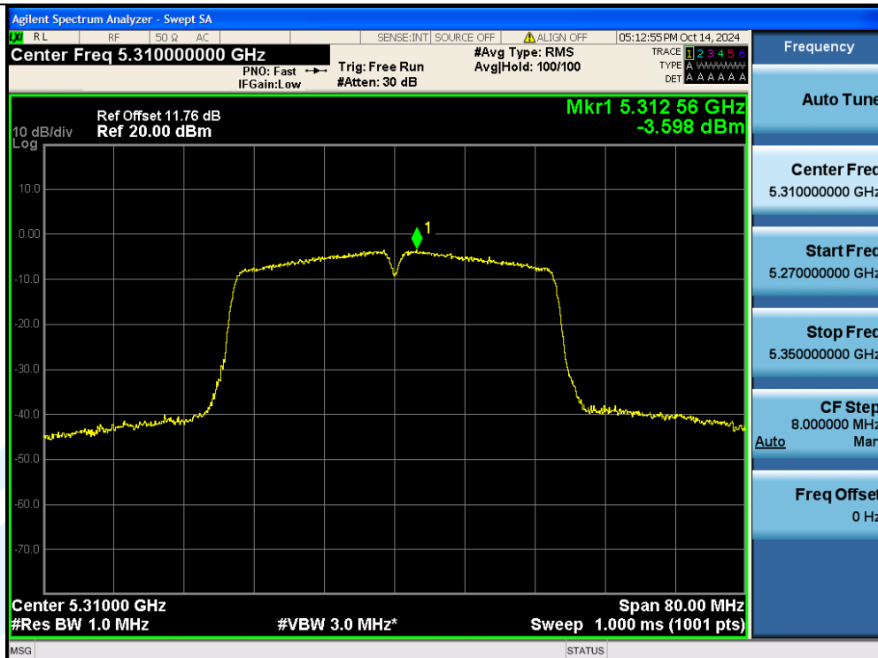
11AC40SISO-Ant1-5310-PASS
