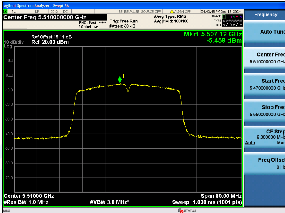
11AC40SISO-Ant1-5510-PASS
