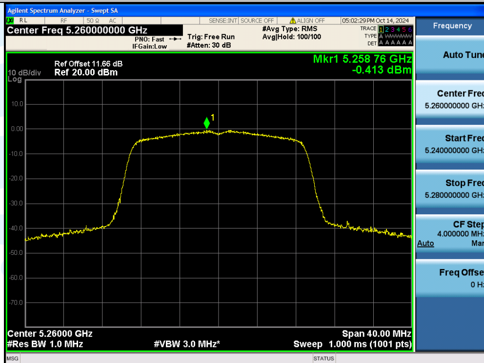
11AC20SISO-Ant1-5260-PASS
