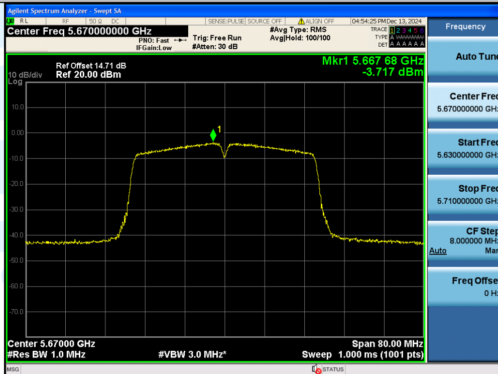
11AC40SISO-Ant1-5670-PASS
