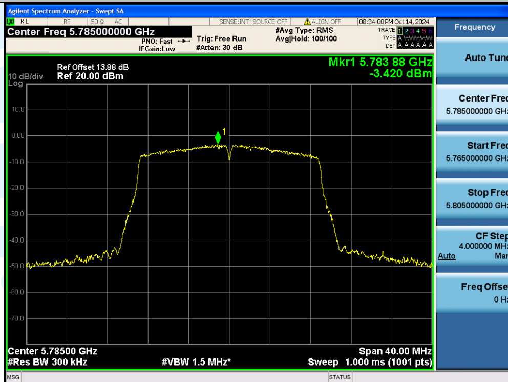
11AC20SISO-Ant1-5785-PASS
