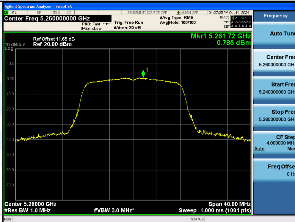
11A-Ant1-5260-PASS
