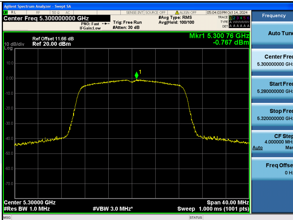
11AC20SISO-Ant1-5300-PASS
