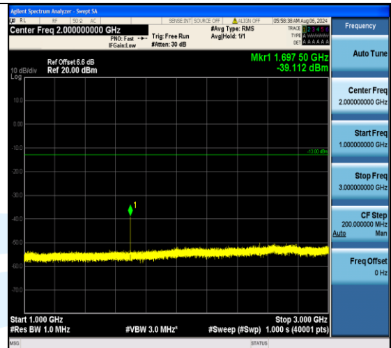
Band5_1.4MHz_16QAM_20643_1RB#5_1000~3000_1000~3000
