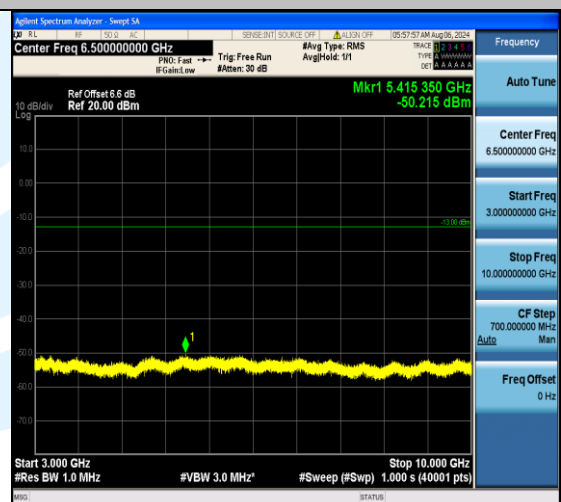
Band5_1.4MHz_16QAM_20643_1RB#0_3000~10000_3000~10000
