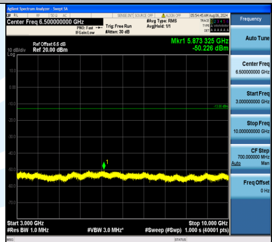
Band5_1.4MHz_16QAM_20407_6RB#0_3000~10000_3000~10000
