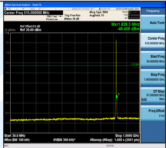
Band5_1.4MHz_16QAM_20407_6RB#0_30~1000_30~1000
