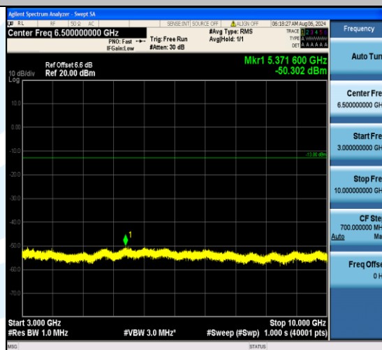
Band5_3MHz_QPSK_20525_1RB#0_3000~10000_3000~10000
