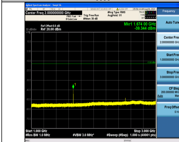
Band5_1.4MHz_16QAM_20525_1RB#5_1000~3000_1000~3000
