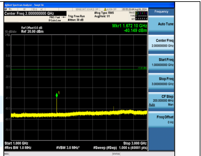
Band5_1.4MHz_16QAM_20525_1RB#0_1000~3000_1000~3000
