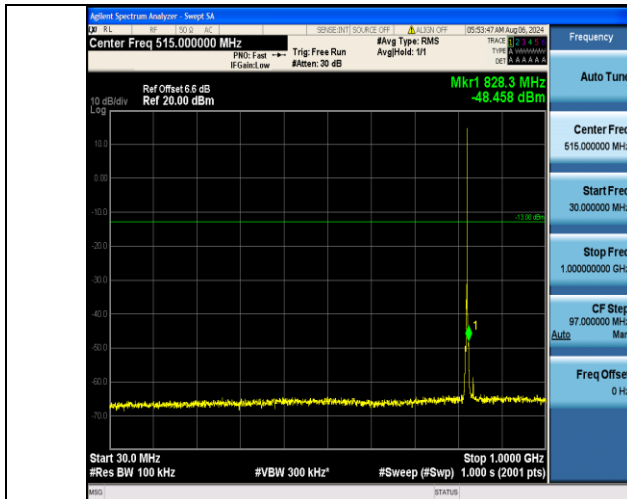
Band5_1.4MHz_16QAM_20407_1RB#5_30~1000_30~1000
