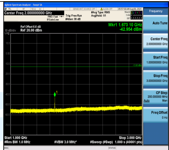
Band5_1.4MHz_16QAM_20525_6RB#0_1000~3000_1000~3000
