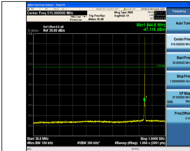
Band5_1.4MHz_16QAM_20643_1RB#5_30~1000_30~1000
