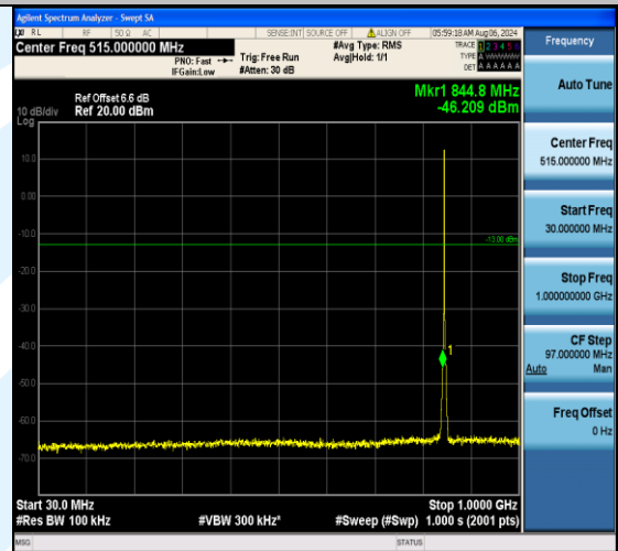
Band5_1.4MHz_16QAM_20643_6RB#0_30~1000_30~1000
