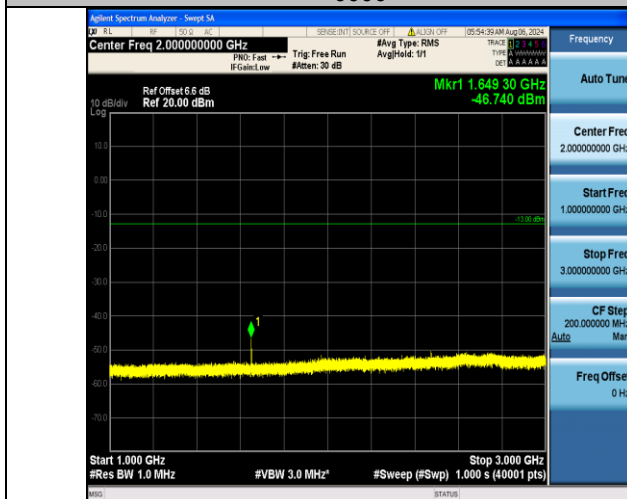
Band5_1.4MHz_16QAM_20407_6RB#0_1000~3000_1000~3000
