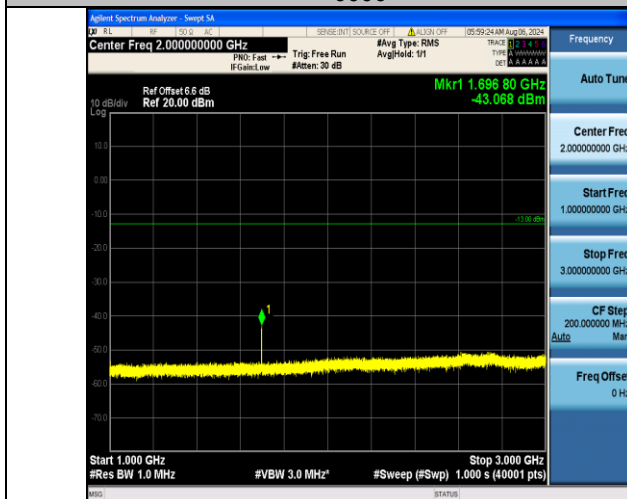
Band5_1.4MHz_16QAM_20643_6RB#0_1000~3000_1000~3000
