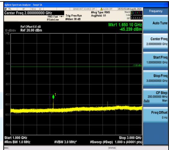
Band5_1.4MHz_16QAM_20407_1RB#5_1000~3000_1000~3000
