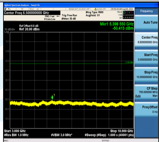
Band5_1.4MHz_16QAM_20643_6RB#0_3000~10000_3000~10000
