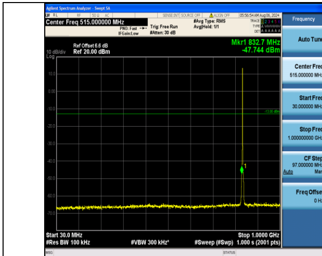
Band5_1.4MHz_16QAM_20525_6RB#0_30~1000_30~1000
