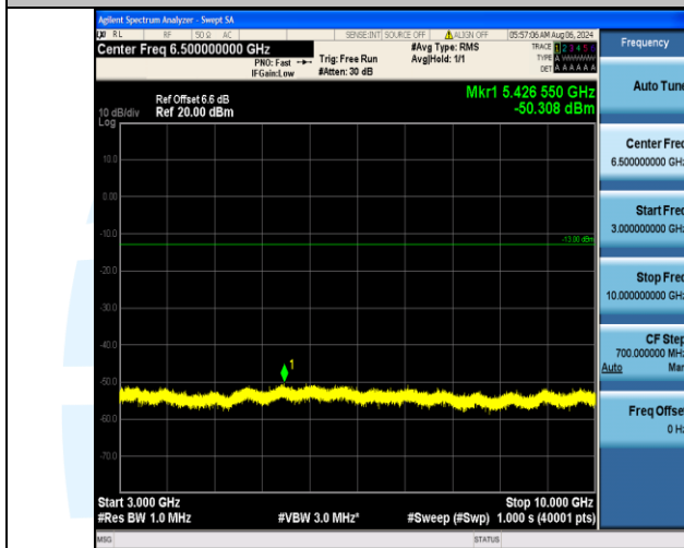
Band5_1.4MHz_16QAM_20525_6RB#0_3000~10000_3000~10000
