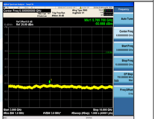
Band5_1.4MHz_16QAM_20525_1RB#5_3000~10000_3000~10000
