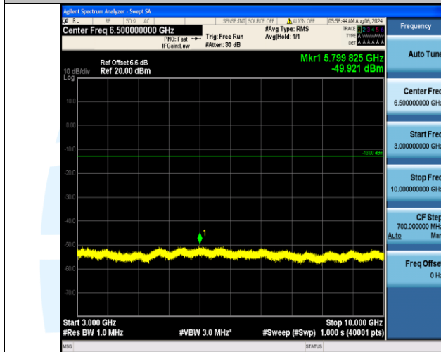
Band5_1.4MHz_16QAM_20643_1RB#5_3000~10000_3000~10000
