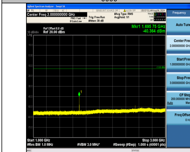
Band5_1.4MHz_16QAM_20643_1RB#0_1000~3000_1000~3000
