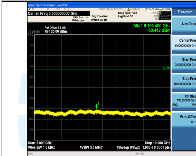
Band5_1.4MHz_16QAM_20407_1RB#5_3000~10000_3000~10000
