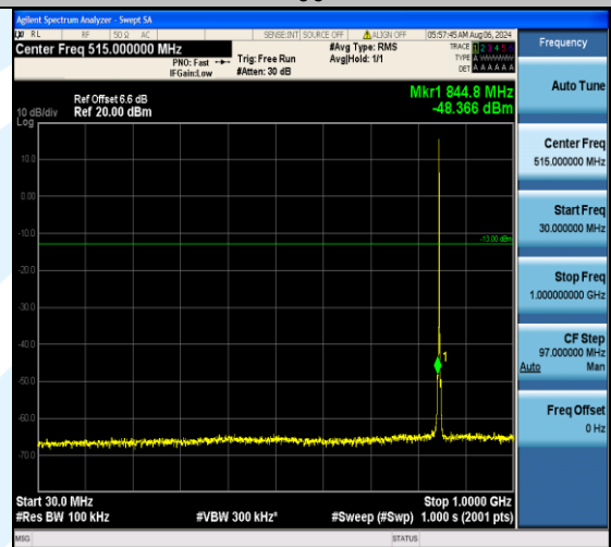
Band5_1.4MHz_16QAM_20643_1RB#0_30~1000_30~1000
