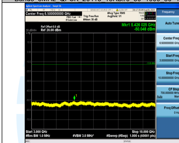
Band5_3MHz_QPSK_20415_15RB#0_3000~10000_3000~10000
