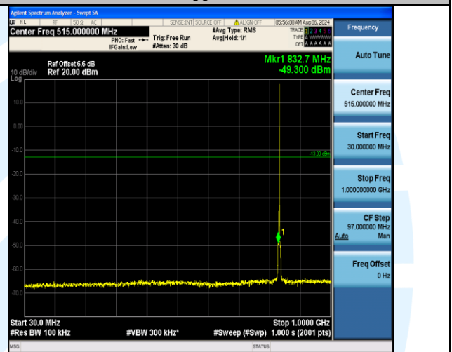
Band5_1.4MHz_16QAM_20525_1RB#5_30~1000_30~1000
