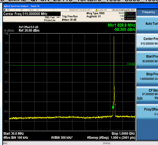
Band5_3MHz_QPSK_20525_1RB#0_30~1000_30~1000
