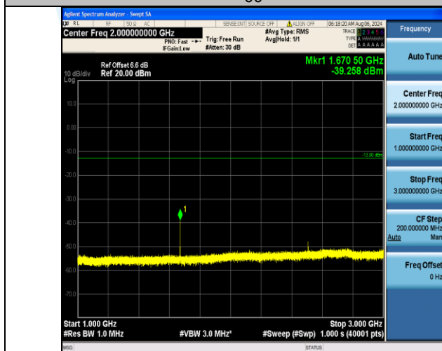
Band5_3MHz_QPSK_20525_1RB#0_1000~3000_1000~3000
