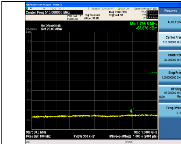
Band4_15MHz_16QAM_20325_1RB#74_30~1000_30~1000
