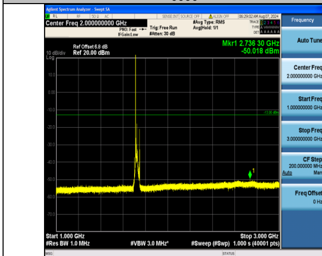
Band4_20MHz_16QAM_20050_1RB#0_1000~3000_1000~3000
