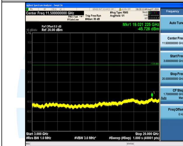
Band4_20MHz_QPSK_20050_100RB#0_3000~20000_3000~20000
