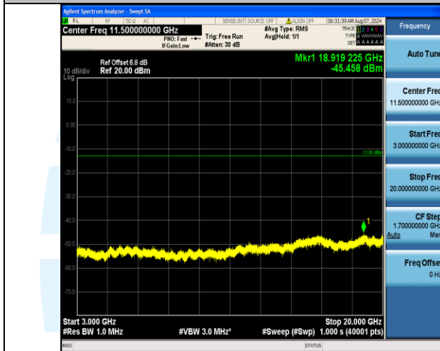
Band4_20MHz_QPSK_20175_1RB#99_3000~20000_3000~20000
