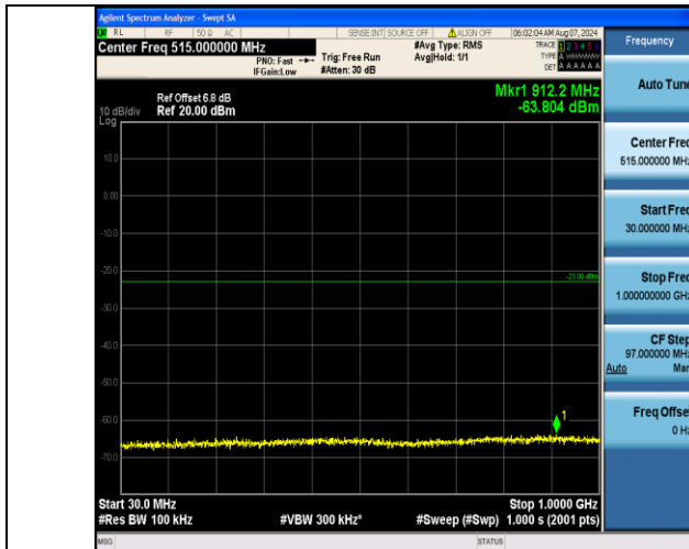
Band4_15MHz_16QAM_20175_75RB#0_30~1000_30~1000
