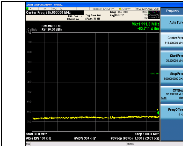
Band4_20MHz_QPSK_20050_100RB#0_30~1000_30~1000
