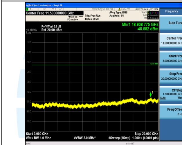
Band4_15MHz_16QAM_20175_75RB#0_3000~20000_3000~20000
