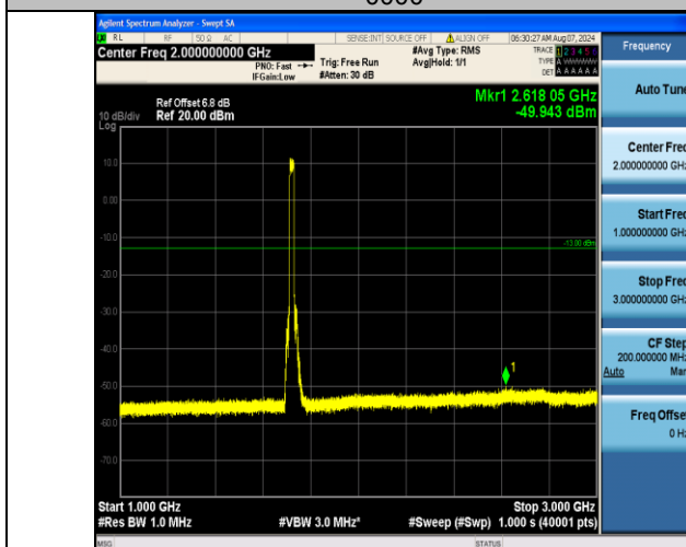
Band4_20MHz_16QAM_20050_100RB#0_1000~3000_1000~3000
