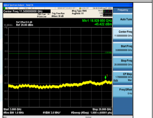
Band4_20MHz_16QAM_20050_100RB#0_3000~20000_3000~20000
