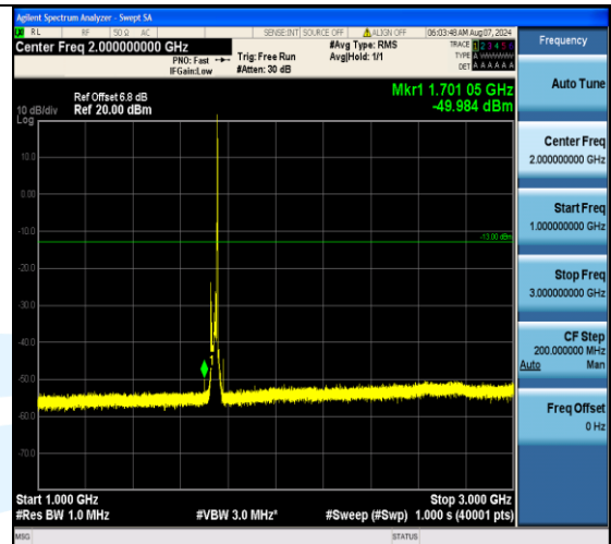
Band4_15MHz_16QAM_20325_1RB#74_1000~3000_1000~3000
