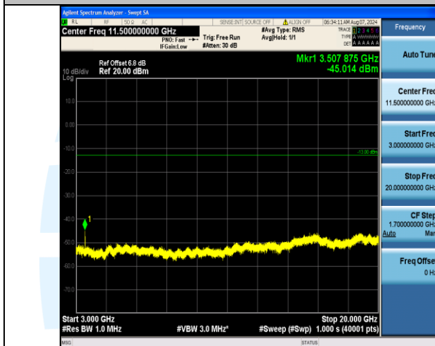
Band4_20MHz_16QAM_20300_1RB#99_3000~20000_3000~20000
