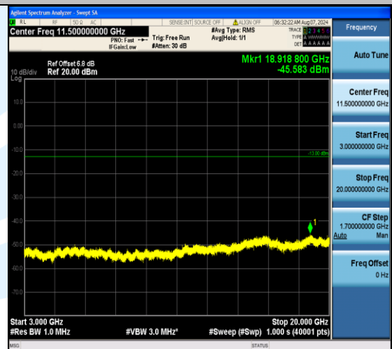
Band4_20MHz_QPSK_20175_100RB#0_3000~20000_3000~20000
