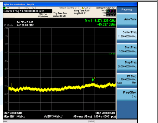
Band4_20MHz_QPSK_20175_1RB#0_3000~20000_3000~20000
