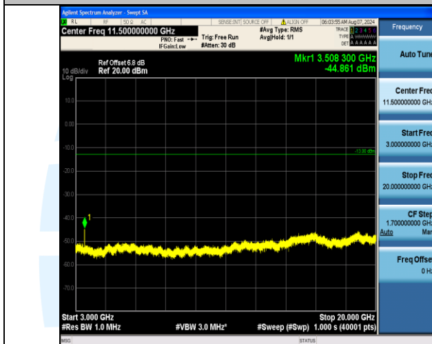
Band4_15MHz_16QAM_20325_1RB#74_3000~20000_3000~20000
