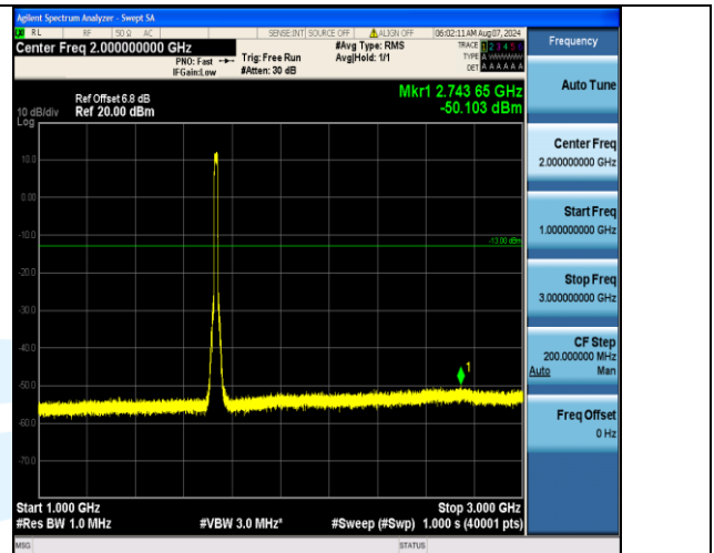
Band4_15MHz_16QAM_20175_75RB#0_1000~3000_1000~3000
