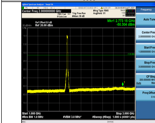
Band4_20MHz_16QAM_20300_100RB#0_1000~3000_1000~3000
