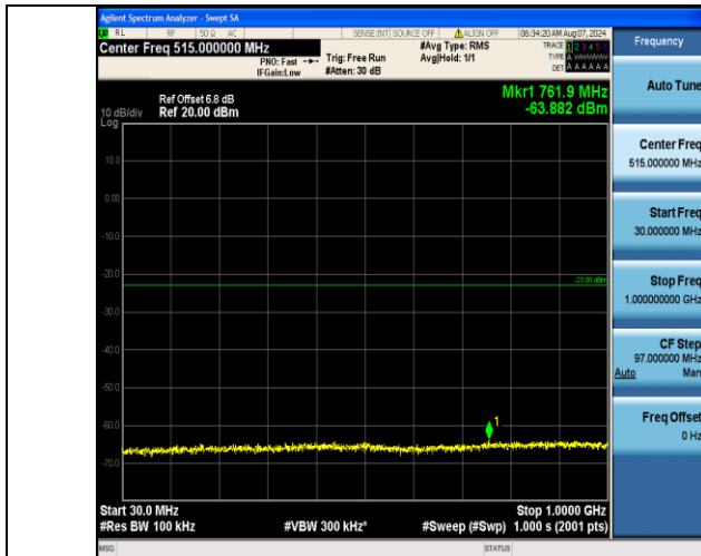
Band4_20MHz_QPSK_20300_100RB#0_30~1000_30~1000
