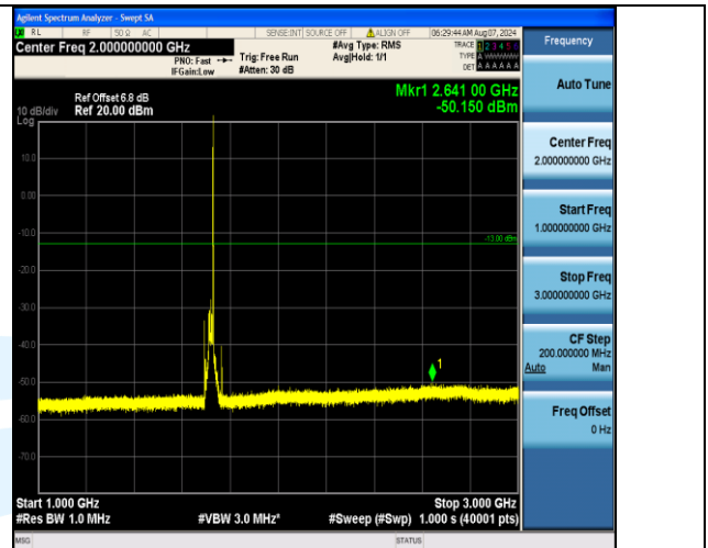
Band4_20MHz_16QAM_20050_1RB#99_1000~3000_1000~3000
