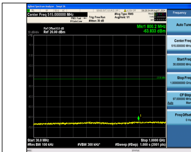
Band4 20MHz QPSK 20050 1RB#0 30~1000 30~1000
