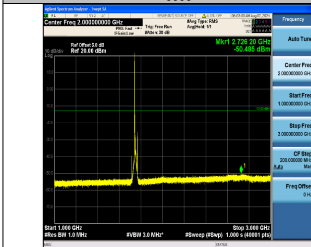
Band4_15MHz_16QAM_20325_1RB#0_1000~3000_1000~3000
