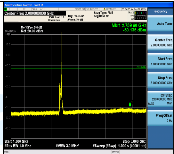
Band4_20MHz_16QAM_20300_1RB#99_1000~3000_1000~3000
