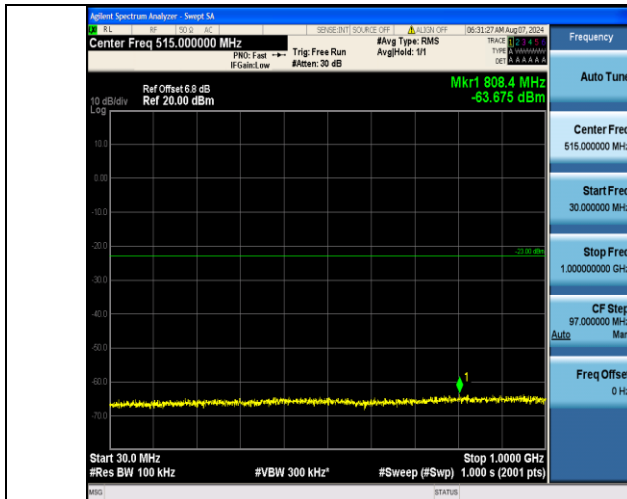
Band4_20MHz_QPSK_20175_1RB#99_30~1000_30~1000
