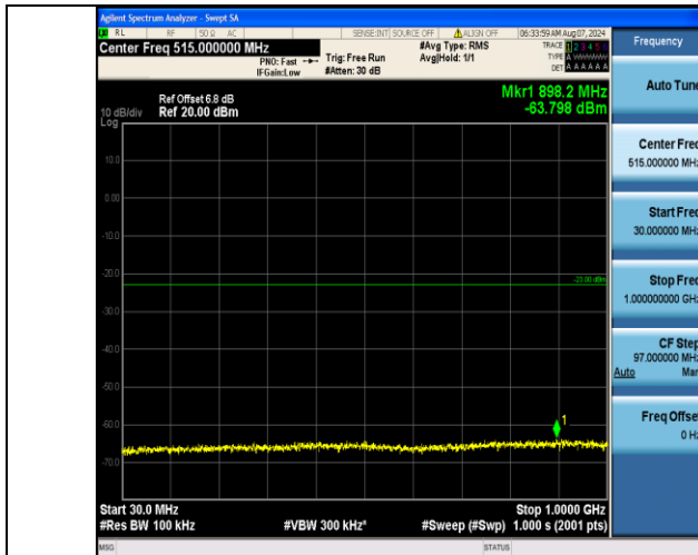
Band4_20MHz_16QAM_20300_1RB#99_30~1000_30~1000
