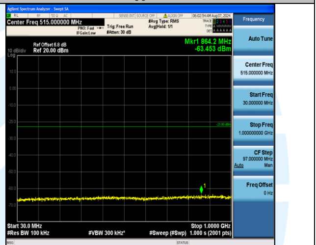
Band4_15MHz_16QAM_20325_1RB#0_30~1000_30~1000
