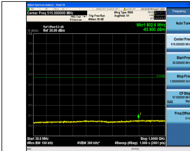
Band4_20MHz_16QAM_20050_1RB#99_30~1000_30~1000
