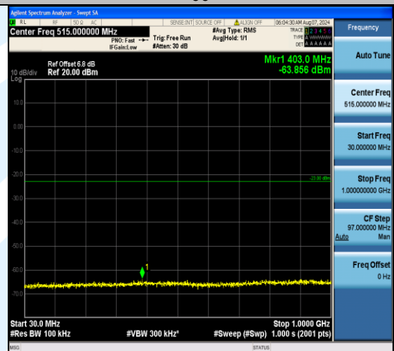
Band4_15MHz_16QAM_20325_75RB#0_30~1000_30~1000
