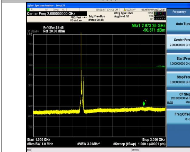
Band4_20MHz_QPSK_20175_1RB#0_1000~3000_1000~3000
