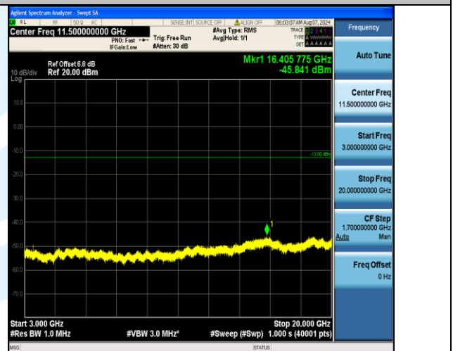
Band4_15MHz_16QAM_20325_1RB#0_3000~20000_3000~20000
