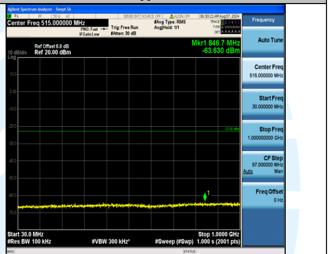
Band4_20MHz_16QAM_20050_100RB#0_30~1000_30~1000
