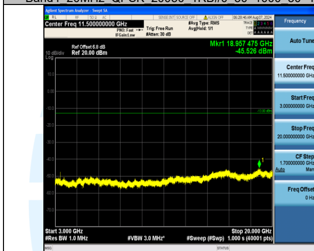
Band4_20MHz_QPSK_20050_1RB#0_3000~20000_3000~20000
