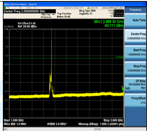
Band4_20MHz_QPSK_20175_1RB#99_1000~3000_1000~3000
