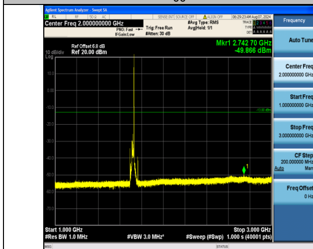
Band4_20MHz_QPSK_20050_1RB#99_1000~3000_1000~3000
