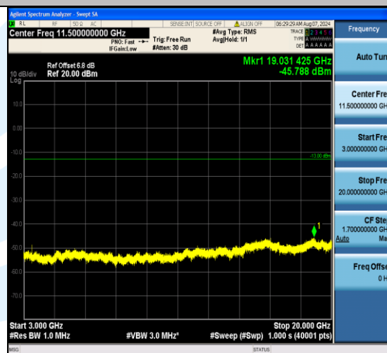
Band4_20MHz_QPSK_20050_1RB#99_3000~20000_3000~20000
