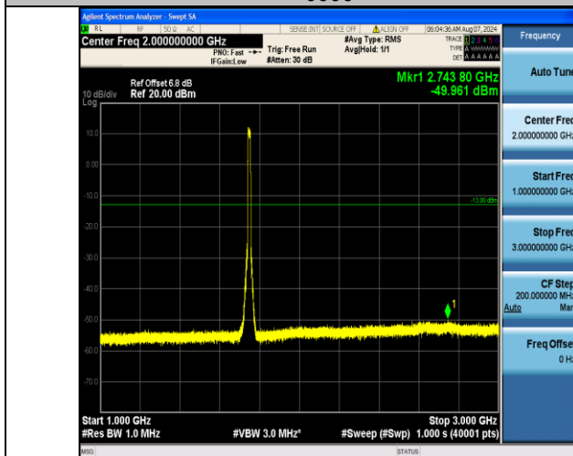
Band4_15MHz_16QAM_20325_75RB#0_1000~3000_1000~3000
