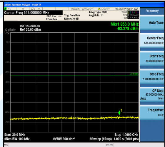
Band4_20MHz_QPSK_20175_100RB#0_30~1000_30~1000
