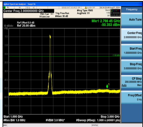
Band4_20MHz_QPSK_20300_100RB#0_1000~3000_1000~3000
