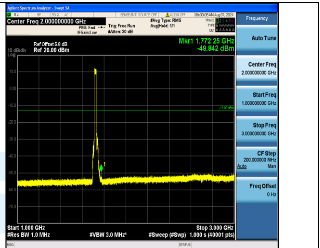
Band4_20MHz_QPSK_20050_100RB#0_1000~3000_1000~3000
