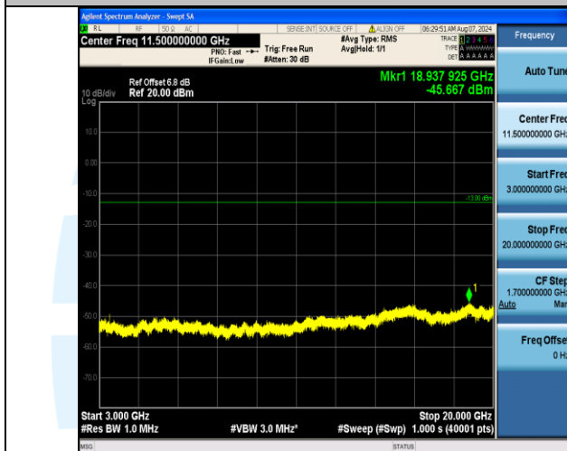
Band4_20MHz_16QAM_20050_1RB#99_3000~20000_3000~20000
