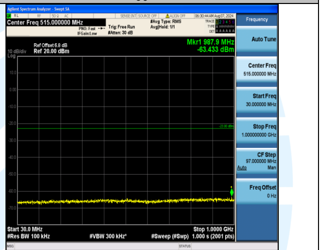
Band4_20MHz_QPSK_20175_1RB#0_30~1000_30~1000
