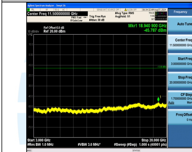
Band4_20MHz_QPSK_20300_100RB#0_3000~20000_3000~20000
