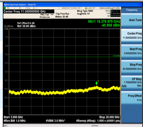
Band4_15MHz_16QAM_20325_75RB#0_3000~20000_3000~20000
