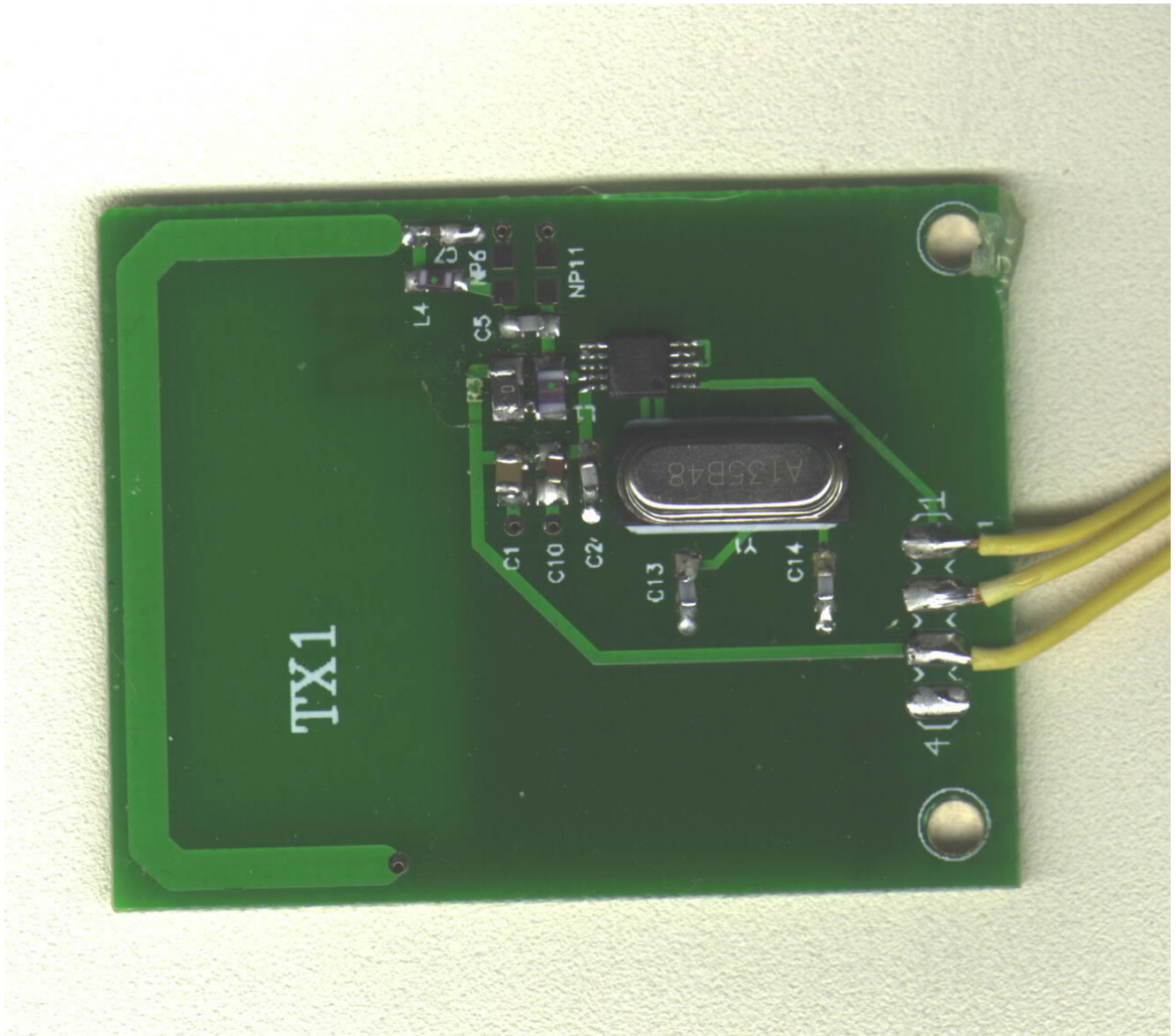
TOP OF TRANSMITTER BOARD
