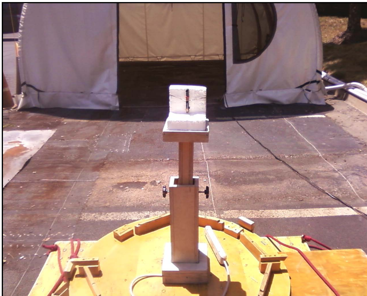
Photograph 3: Radiated Emissions – Front View
