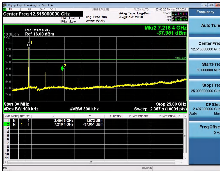
2_Spurious_Emissions_NVNT_ANT1_2.4G_2405_00
