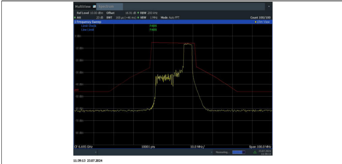
11AX20SISO_Ant2_6695_106Tone_RU54
