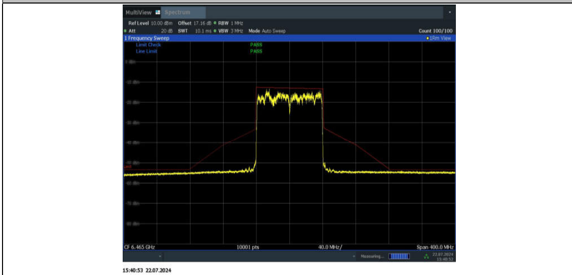
11AX80SISO_Ant2_6465
