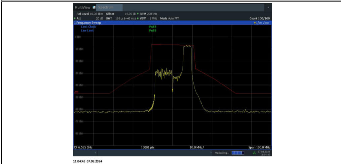
11AX20SISO_Ant2_6535_52Tone_RU40
