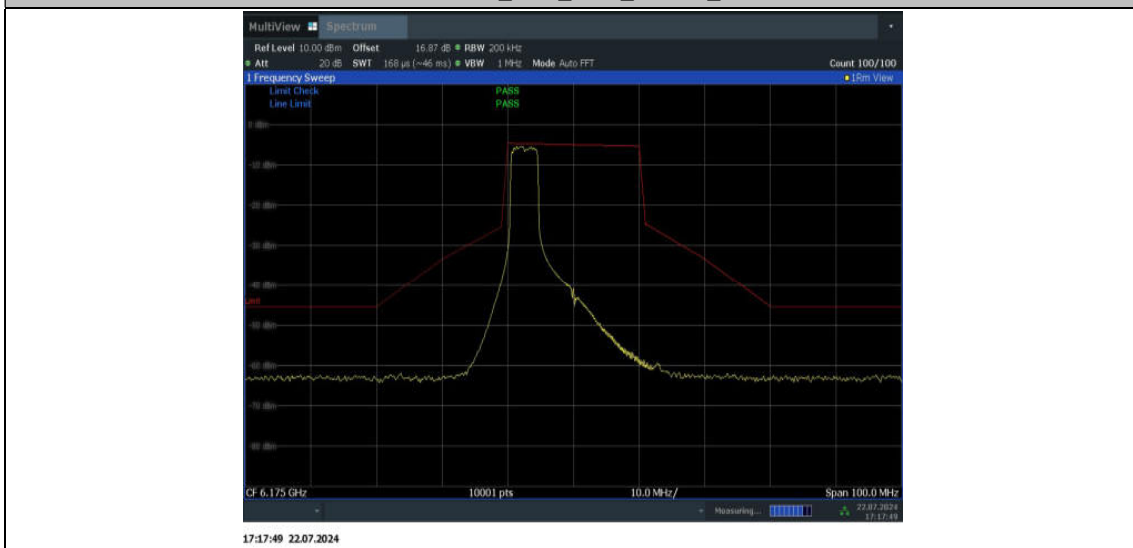
11AX20SISO_Ant2_6175_52Tone_RU37
