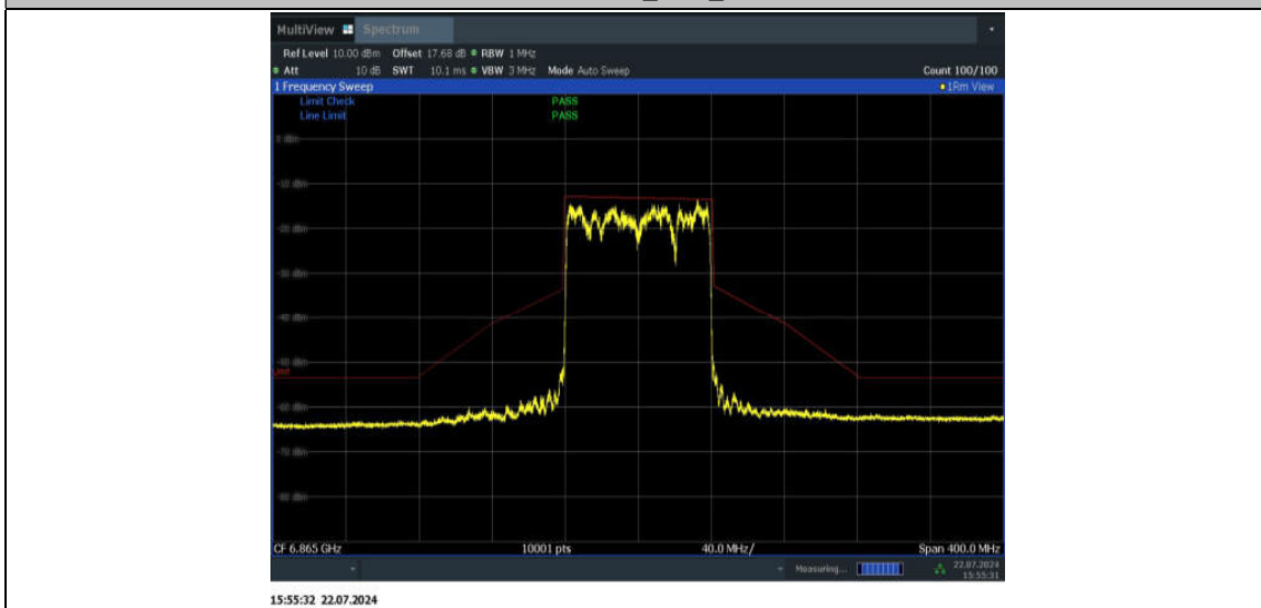
11AX80SISO_Ant2_6865
