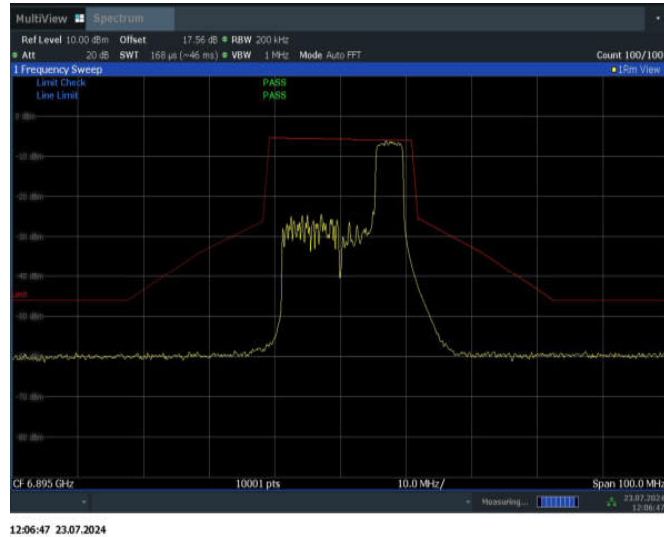
11AX20SISO_Ant2_6895_106Tone_RU54
