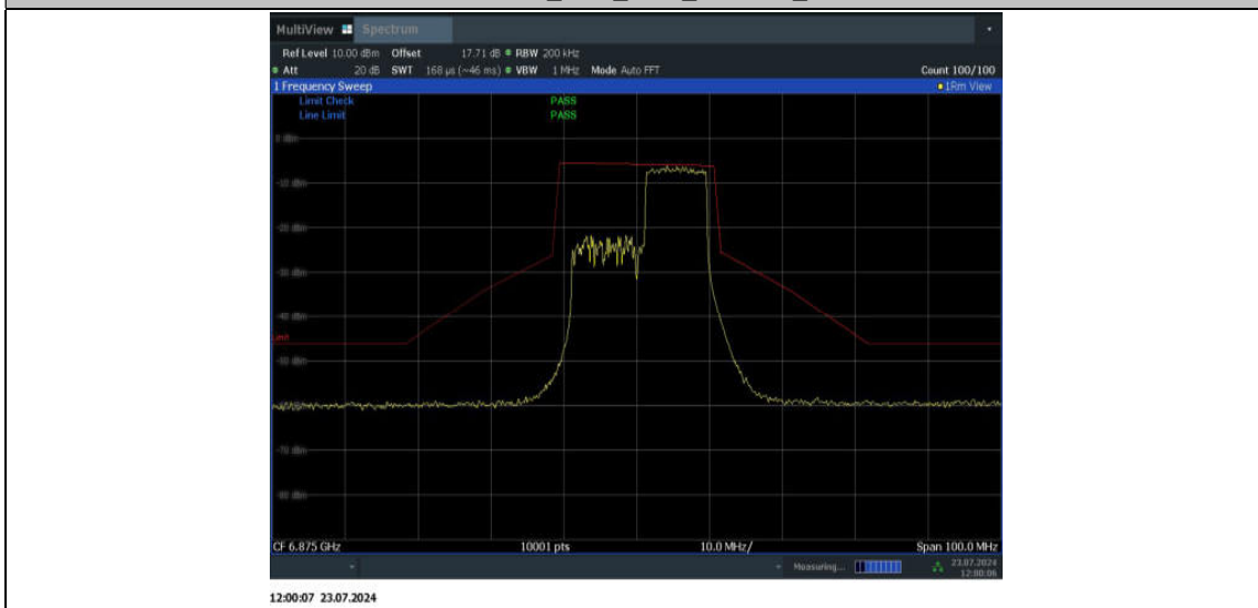
11AX20SISO_Ant2_6875_106Tone_RU54
