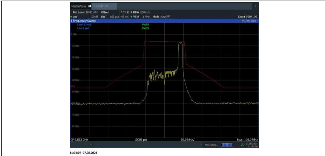
11AX20SISO_Ant2_6875_52Tone_RU40
