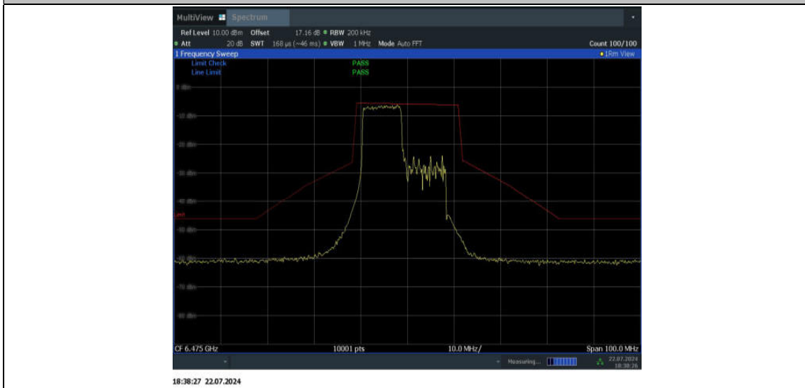
11AX20SISO_Ant2_6475_106Tone_RU53
