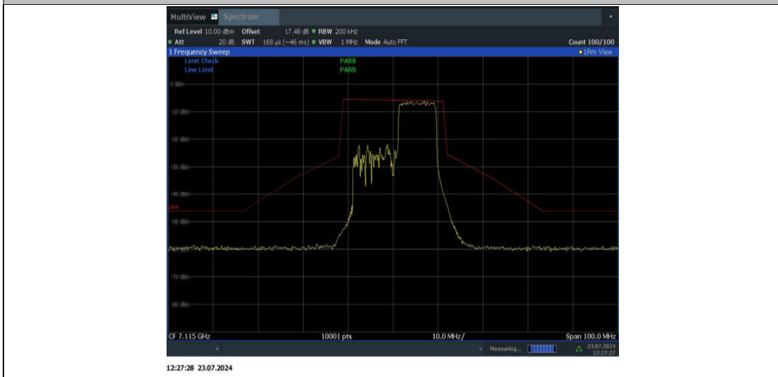
11AX20SISO_Ant2_7115_106Tone_RU54
