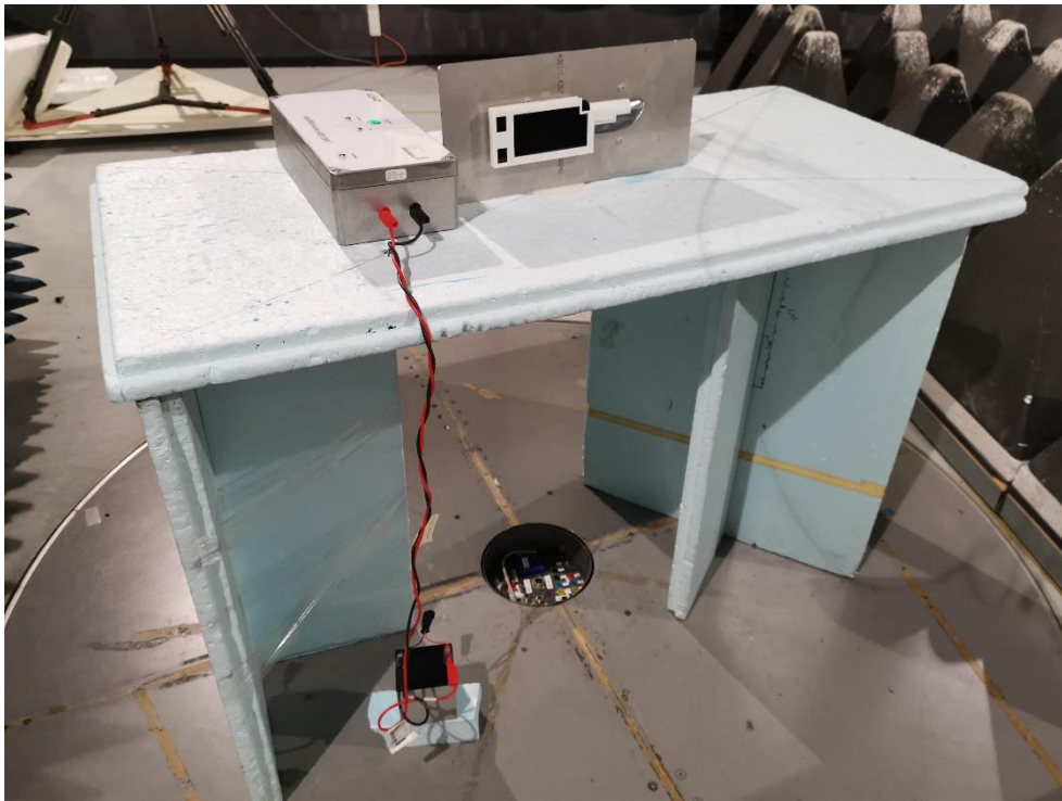
Photograph 2: Close view of the test setup in the semi-anechoic chamber. EUT stands.
