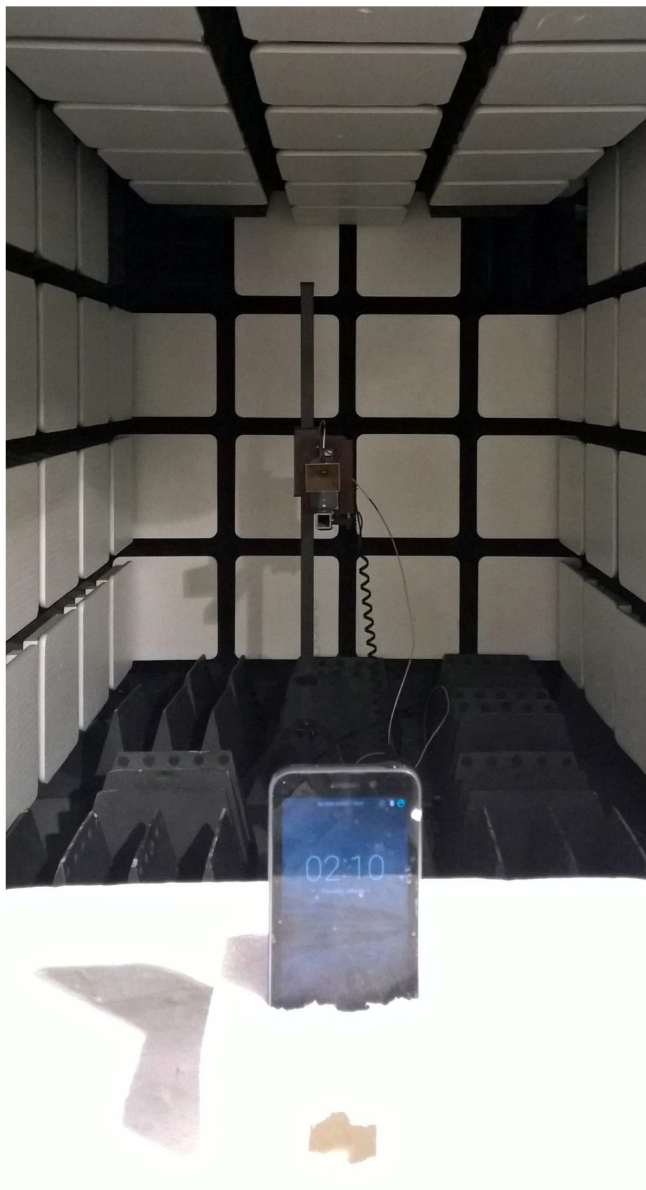
Radiated test setup 18 – 20 GHz, EUT vertical
