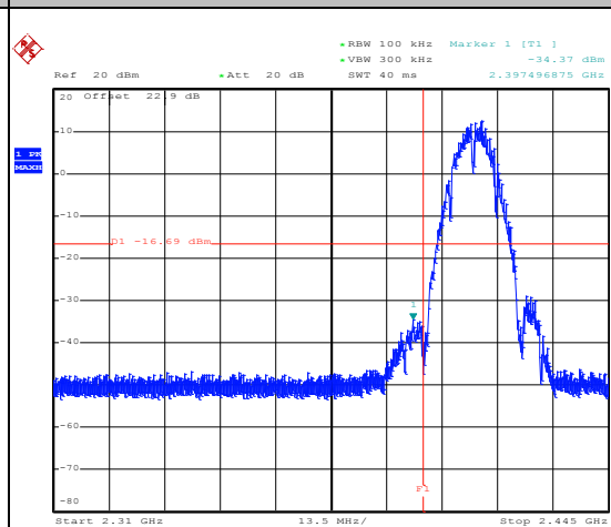
Channel Plot
