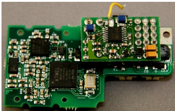
Figure 12: Gyro Board stacked with COTS Command Receiver
