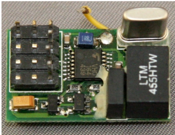
Figure 8: Command Receiver (COTS Product, Top)
