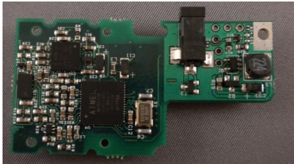
Figure 11: Gyro Board (Bottom)
