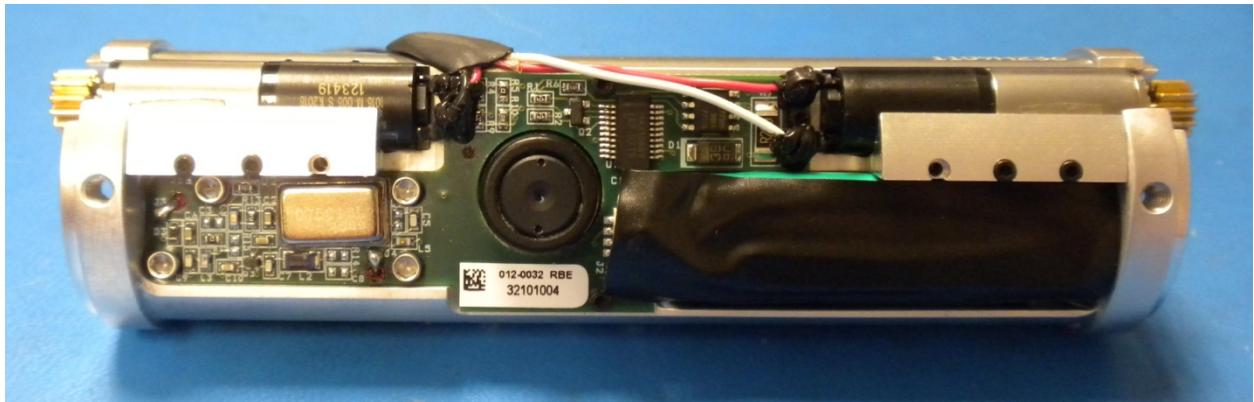
Figure 2: Chassis Front
