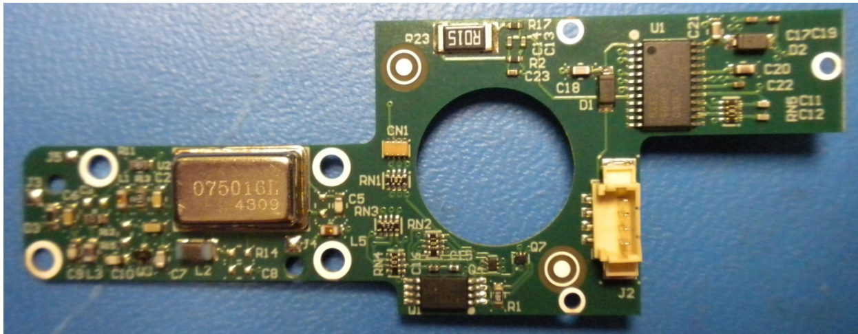
Figure 6: FrontBoard (Top)
