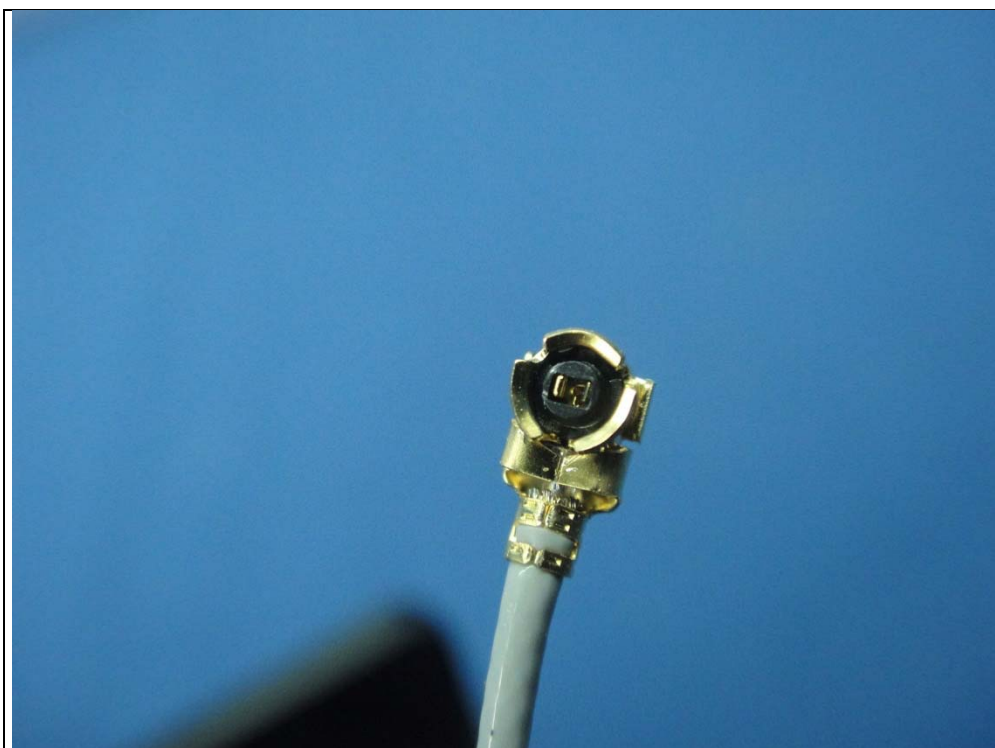
WIFI Antenna 1 (Model No.: RFA-25-G170-70B-154)
