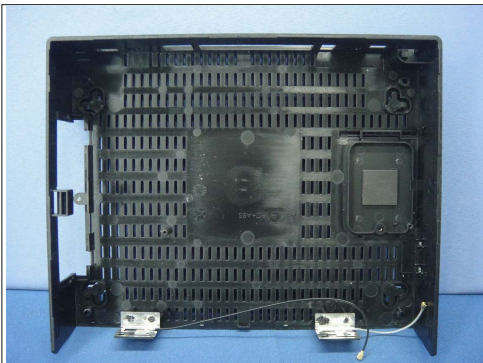
WIFI Antenna 1 (Model No.: RFA-25-G170-70-64)
