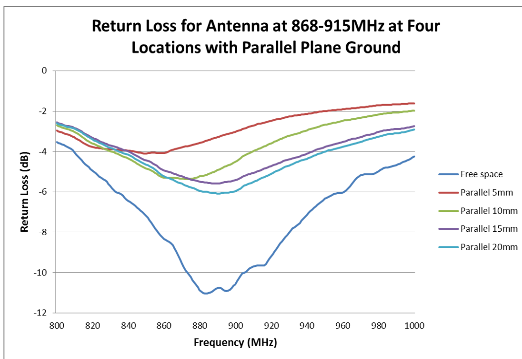
FIGURE 7.3.2 RETURN LOSS OF ANTENNA AT 868/915MHZ AT FOUR LOCATIONS WITH PARALLEL PLANE GROUND
