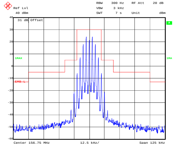
156.750MHz- Low Power Level
