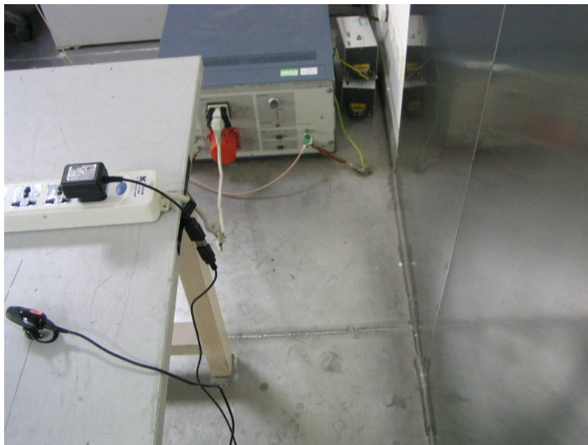
Charging Mode: Conducted Emission - Side View
