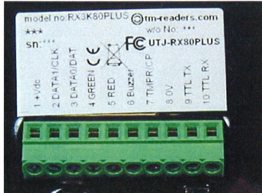
PRODUCT LABEL (artwork) (FCC UTJ-RX80PLUS)
