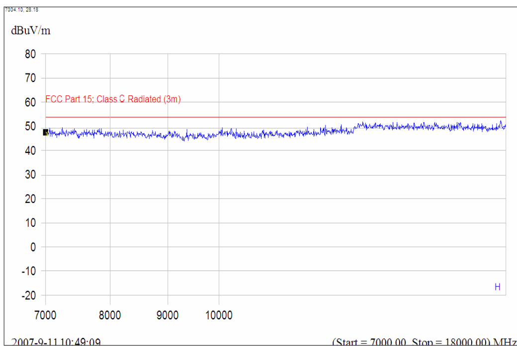
(Plot B.4: Antenna Horizontal, 7GHz to 18GHz)
