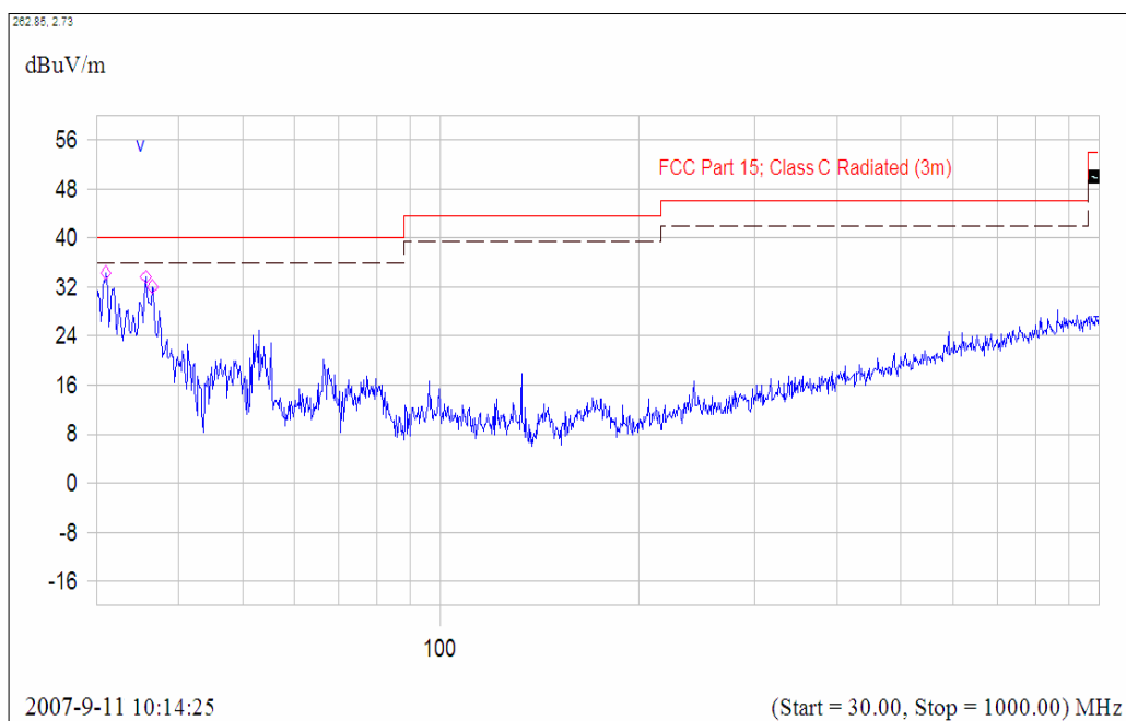
(Plot A.6: Antenna Vertical, 30MHz to 1GHz)
