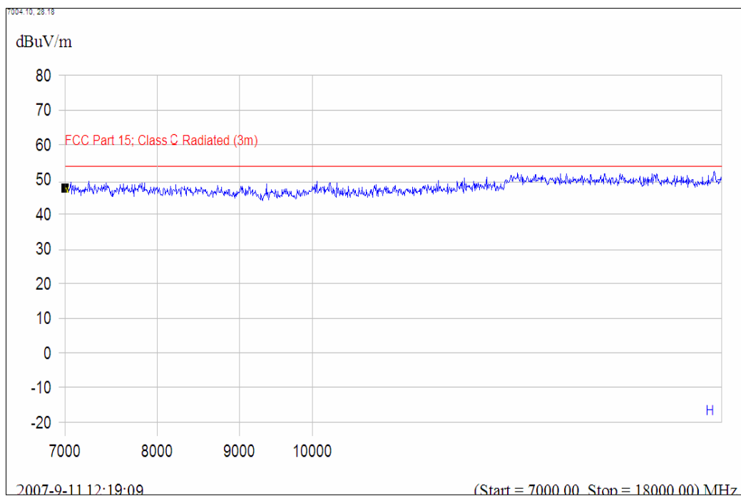
(Plot A.4: Antenna Horizontal, 7GHz to 18GHz)
