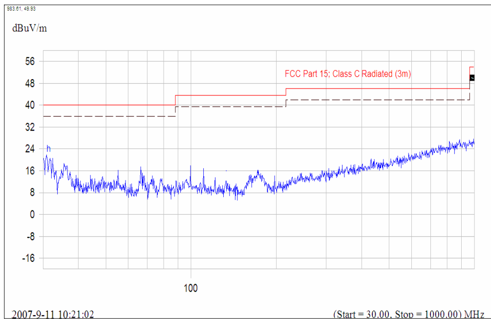
(Plot B.2: Antenna Horizontal, 30MHz to 1GHz)
