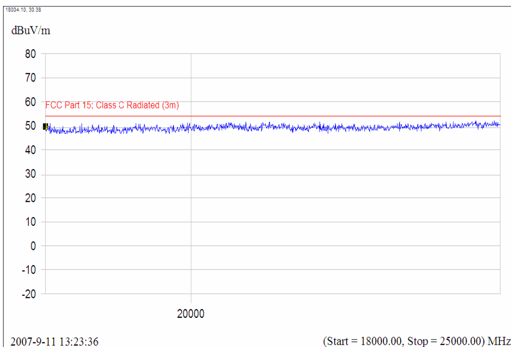
(Plot C.5: Antenna Horizontal, 18GHz to 25GHz)
