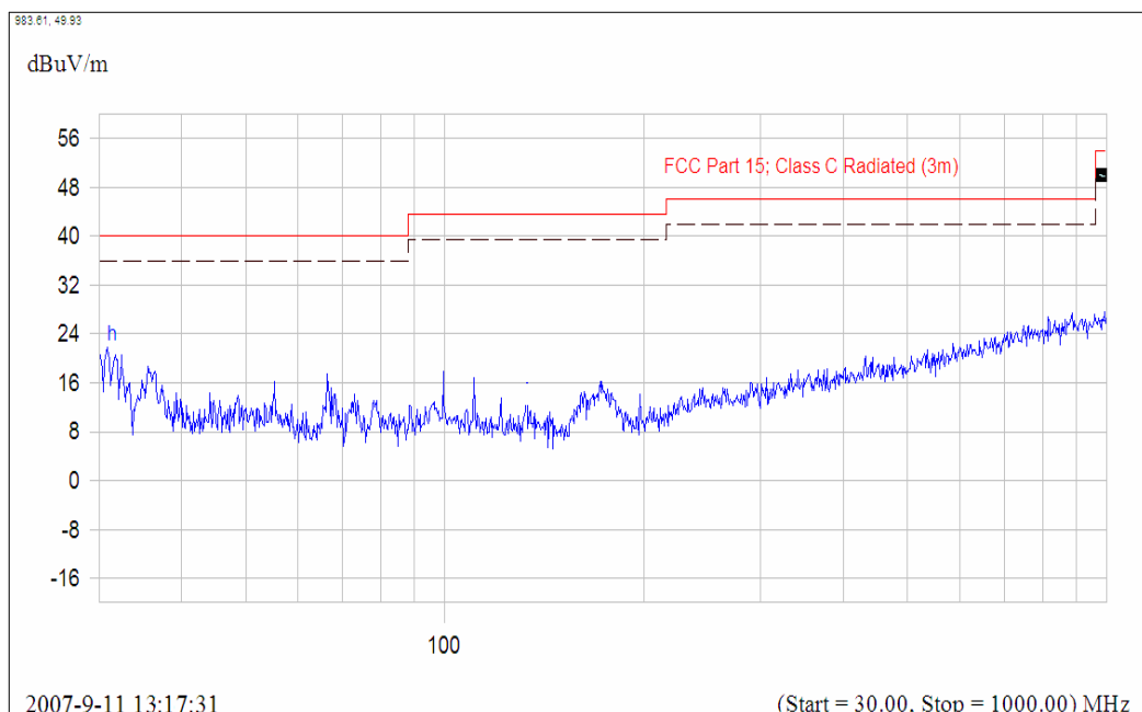
(Plot C.2: Antenna Horizontal, 30MHz to 1GHz)
