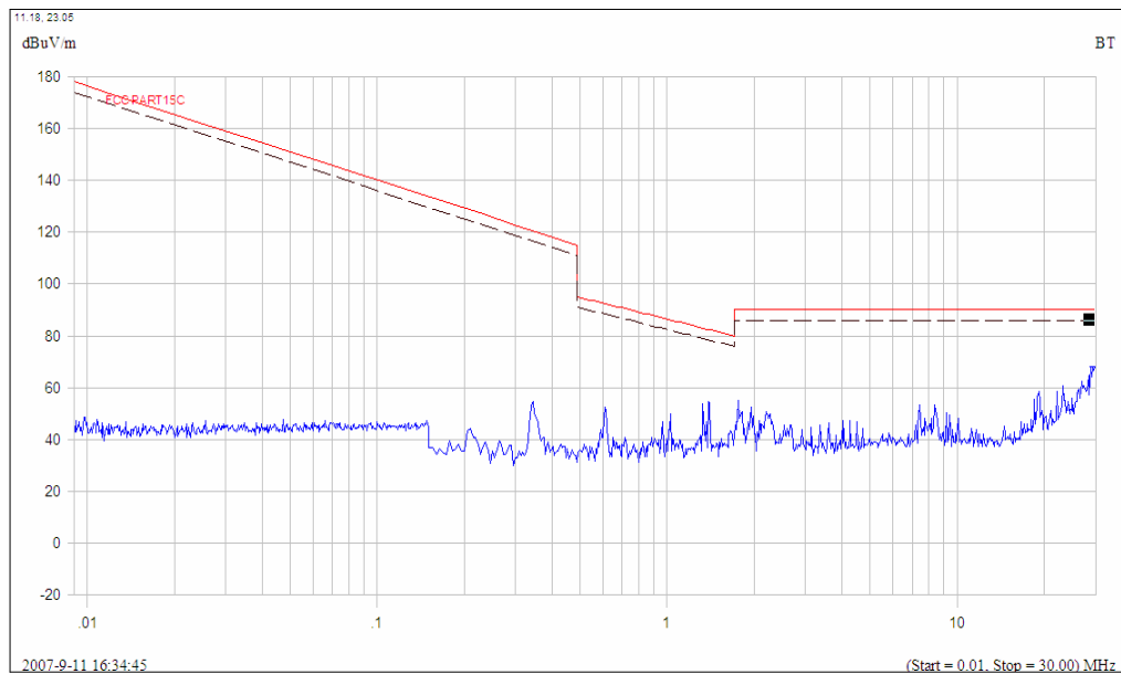
(Plot A.1: 9kHz to 30MHz)
