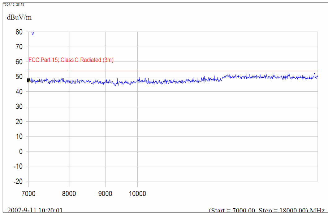
(Plot A.8: Antenna Vertical, 7GHz to 18GHz)
