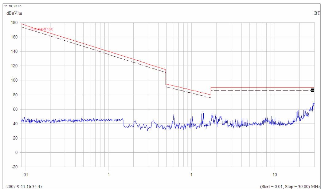
(Plot C.1: 9kHz to 30MHz)
