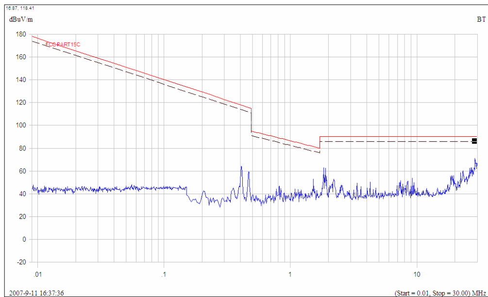
(Plot B.1: 9kHz to 30MHz)
