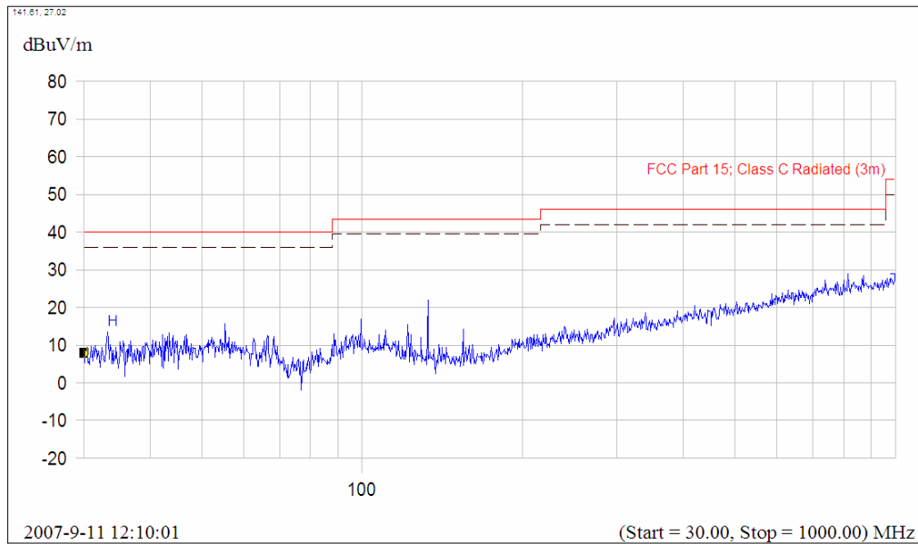
(Plot A.2: Antenna Horizontal, 30MHz to 1GHz)
