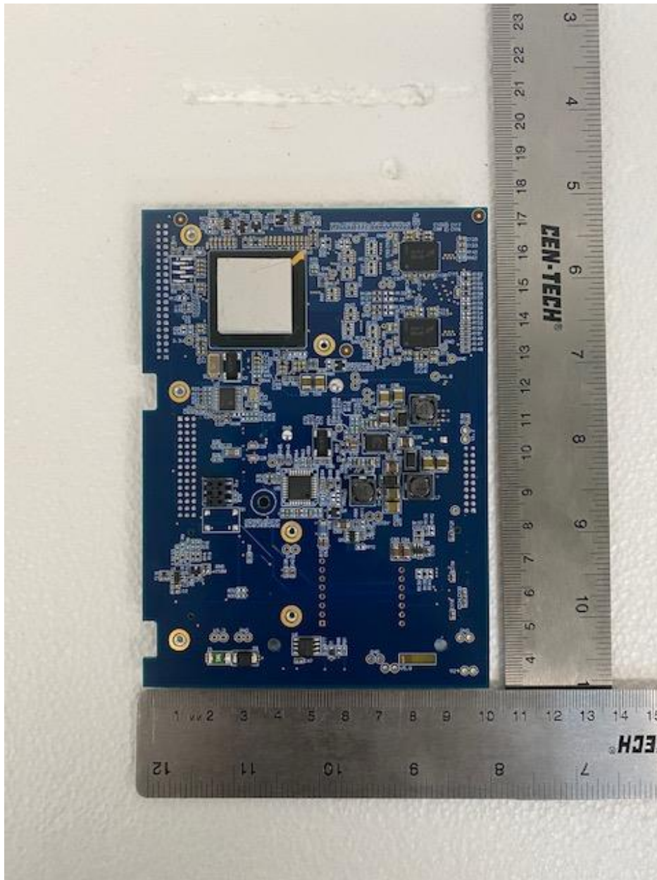
Figure 3. Processor PCB – Bottom
