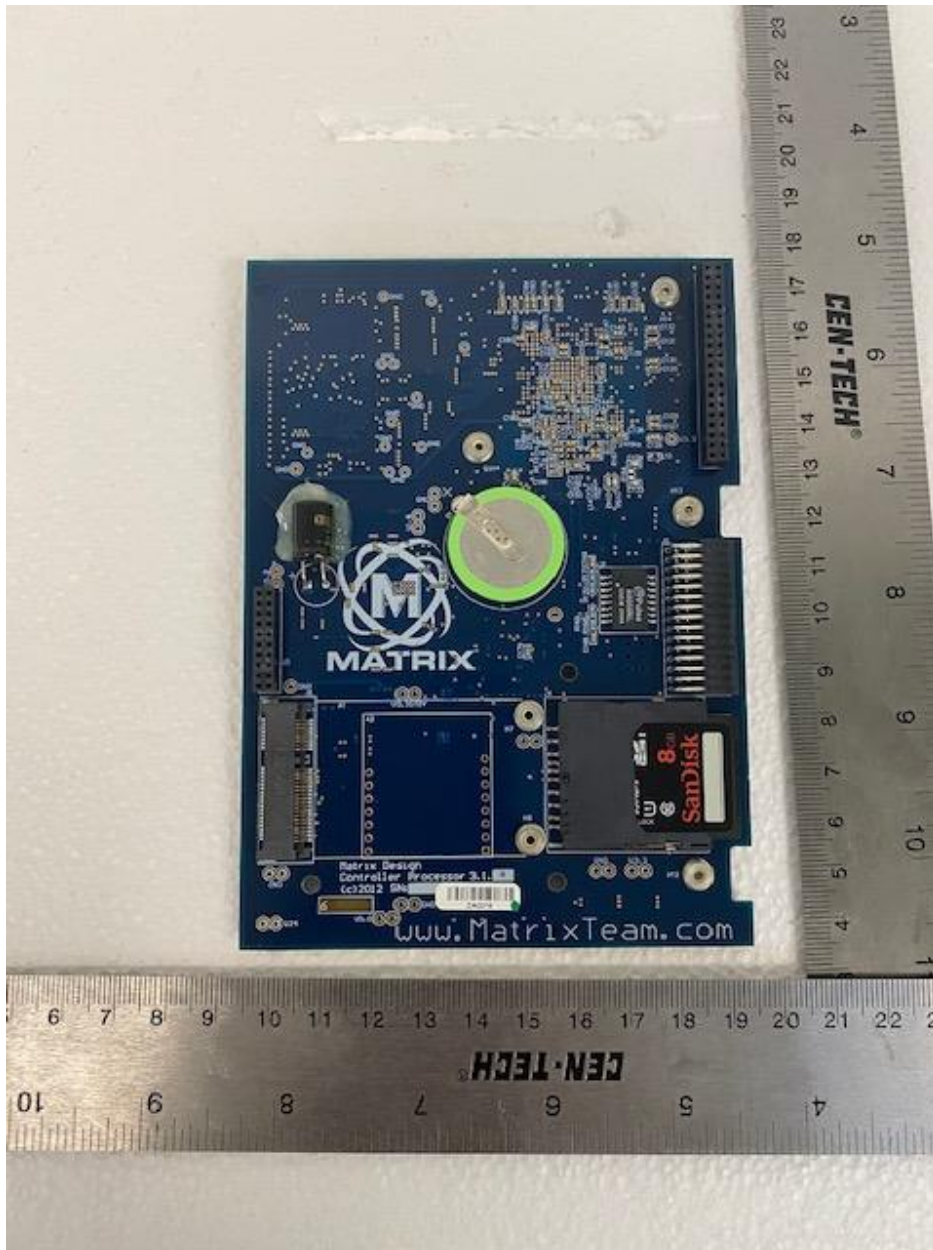
Figure 2. Processor PCB – Top
