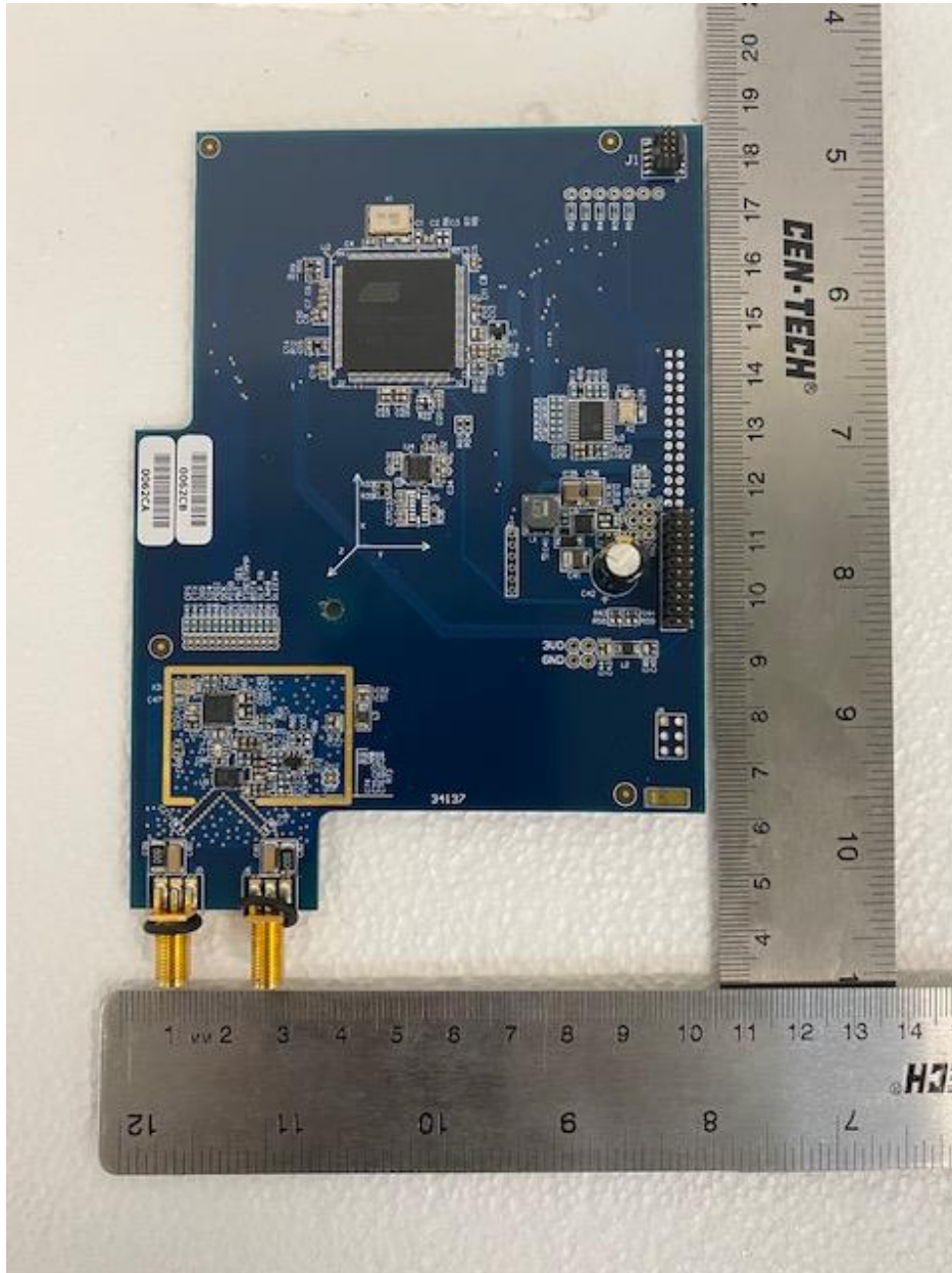
Figure 6. Wireless PCB – Top
