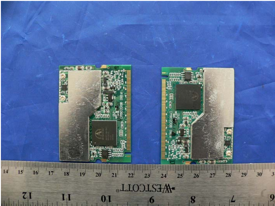
EUT – RF Board 2.4 & 5 GHz Band with RF Shielding (Component Side View)
