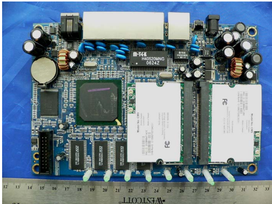
EUT – Main Board Assembly (Component Side View1)
