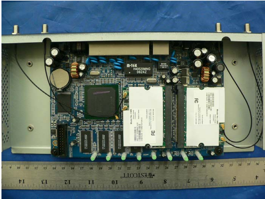
EUT – Chassis View Top Cover Removed
