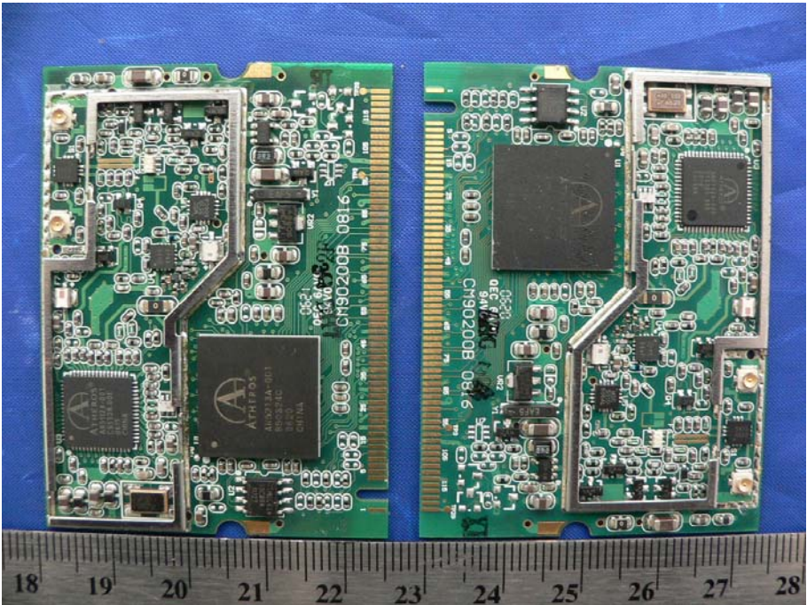
EUT – RF Board 2.4 & 5 GHz Band without RF Shielding (Component Side View)
