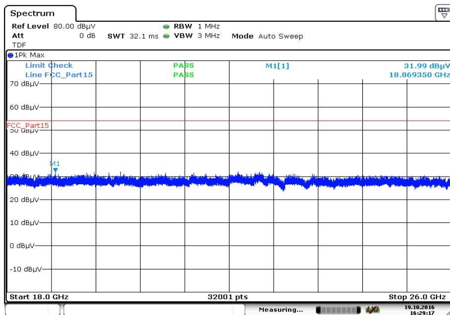
Plot 8: 18 GHz to 26 GHz, TX mode, channel 19, vertical & horizontal polarization
