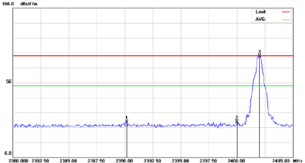
TEST PLOT OF BAND EDGE FOR LOW CHANNEL (3Mbps)
