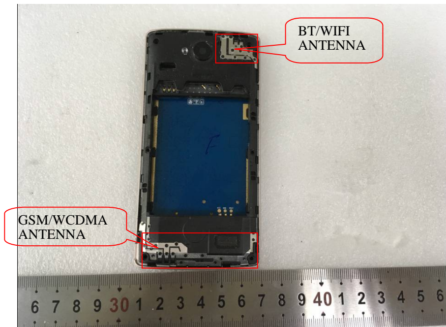
EUT – Ant View
