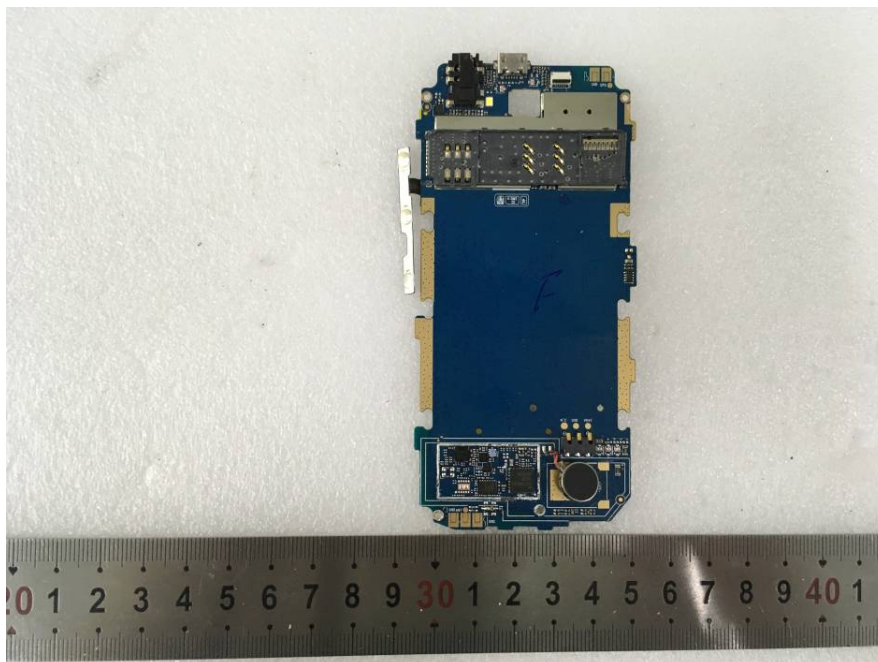
EUT –Main Board Top Shielded off View 1
