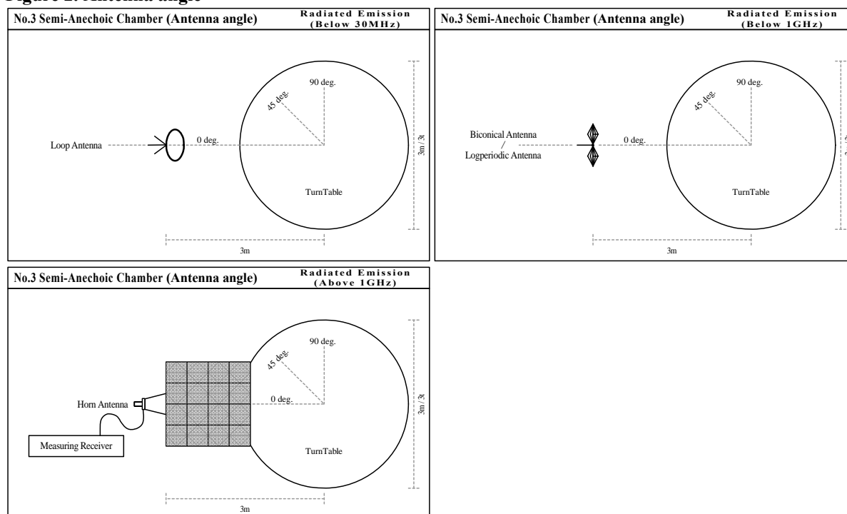
Figure 2. Antenna angle
