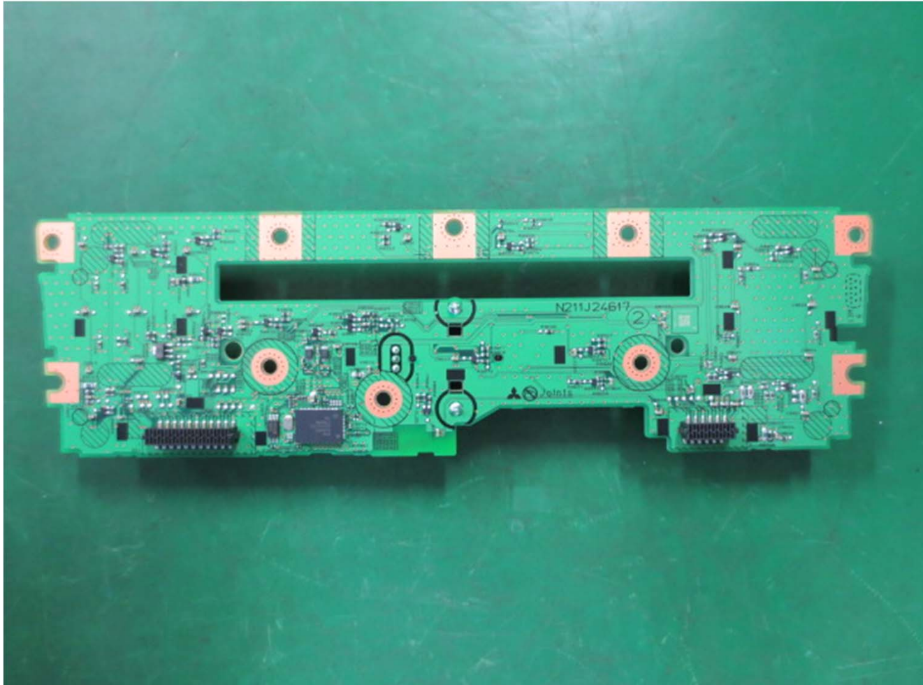
12. PCB-PANEL S-side
