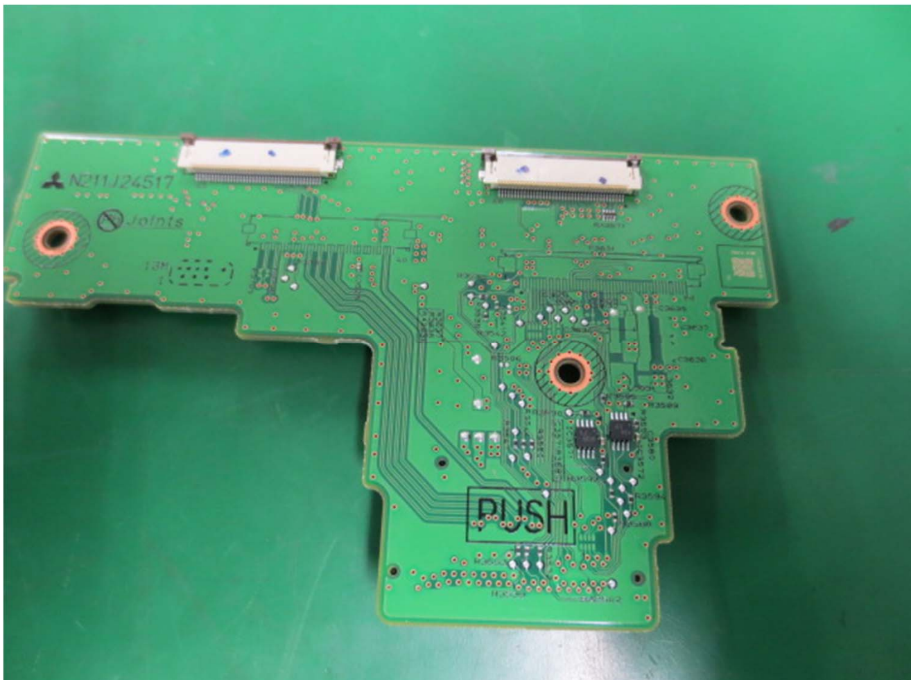
8. PCB-IF (PCB-NAVI-B) S-side
