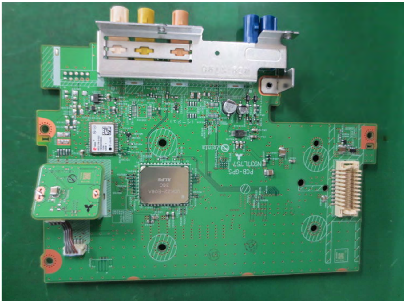
5. PCB-GPS (PCB-NAVI-B) C-side
