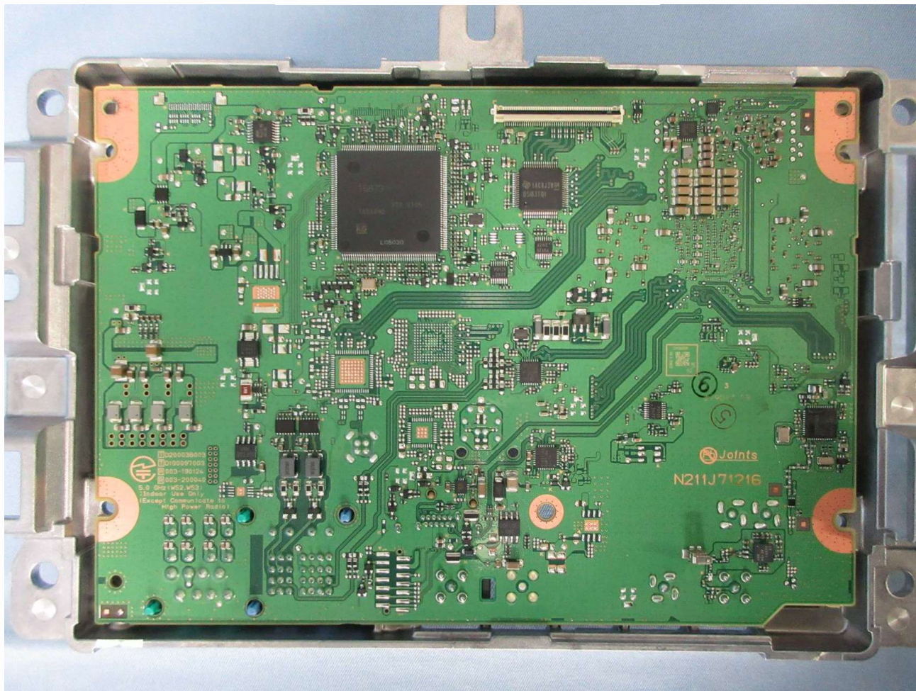
PCB-MAIN S-side
