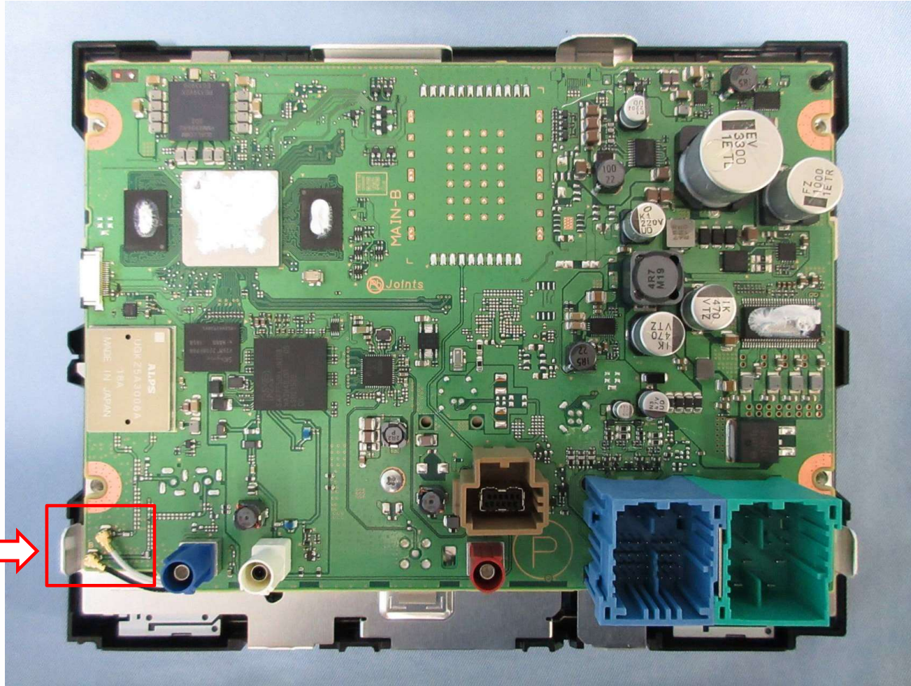
PCB-MAIN C-side
