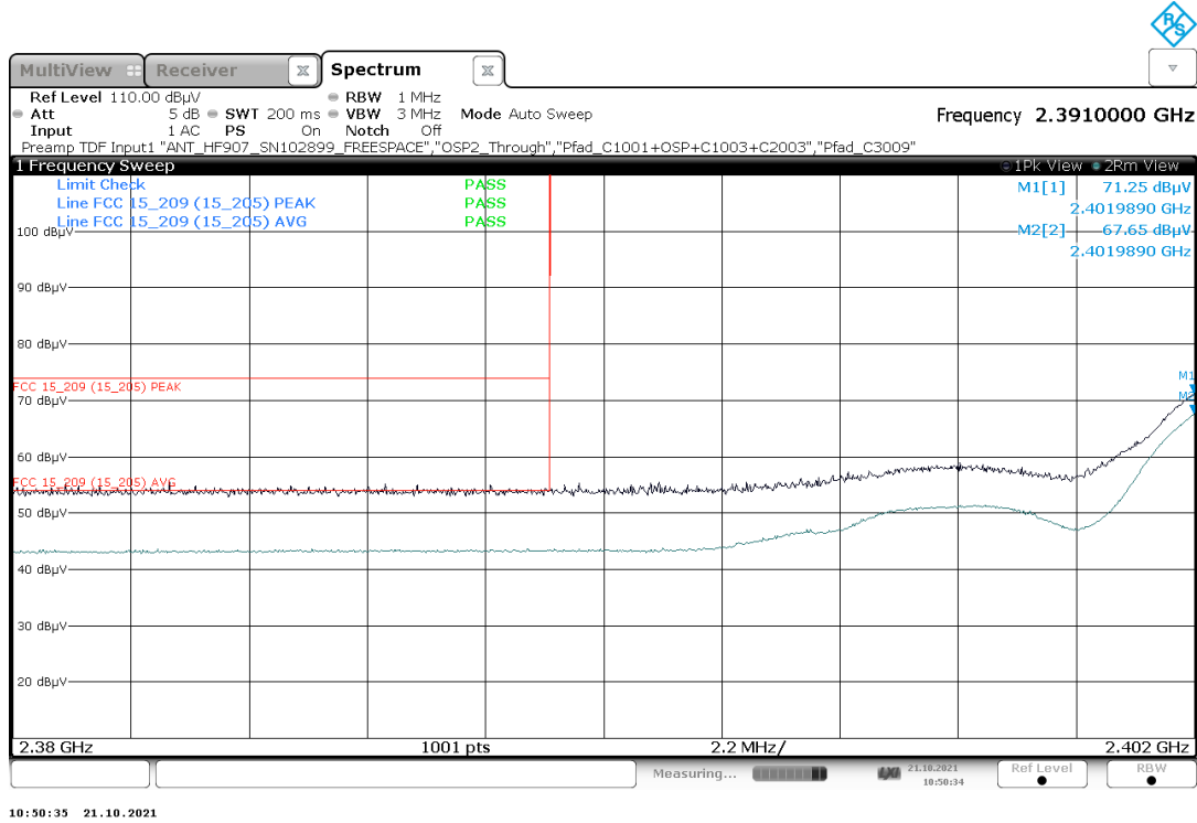
Plot 45: Mode 1, BEC, low channel 1
