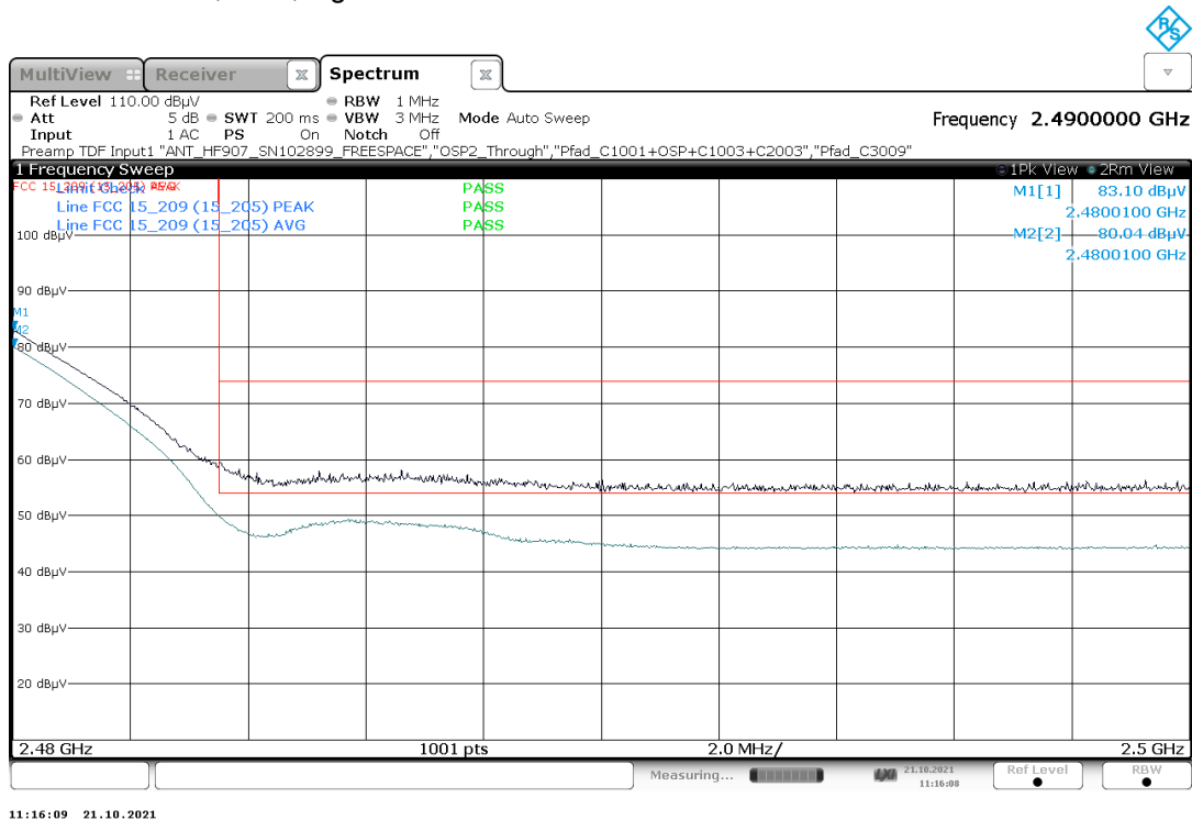
Plot 46: Mode 1, BEC, high channel 13
