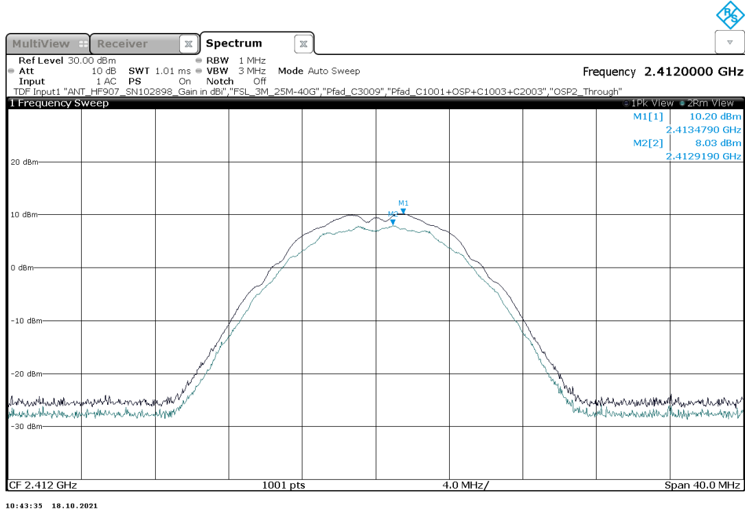
Plot 11: Test Mode 1, DBPSK, 1 Mbit/s, Peak EIRP, low channel 1, 2412 MHz
