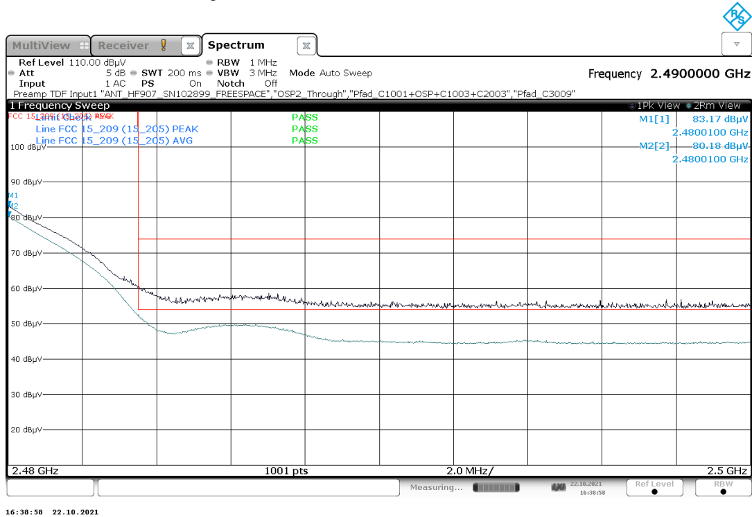
Plot 24: Mode 1, BEC, high channel 13
