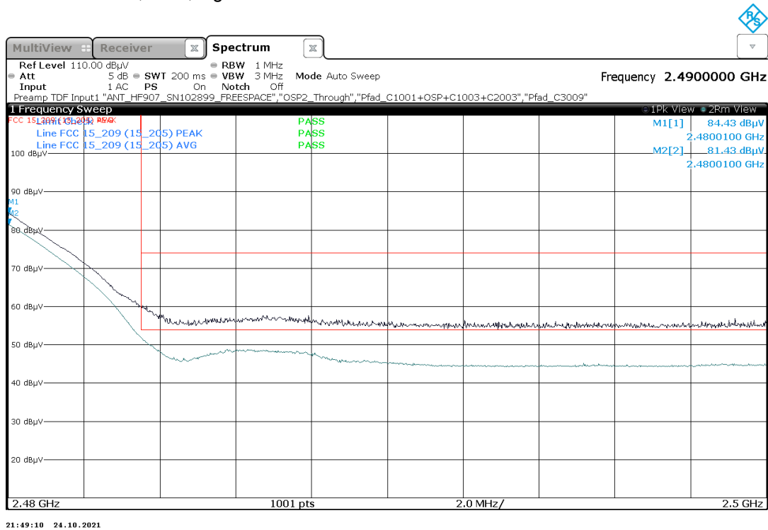
Plot 14: Mode 1, BEC, high channel 13
