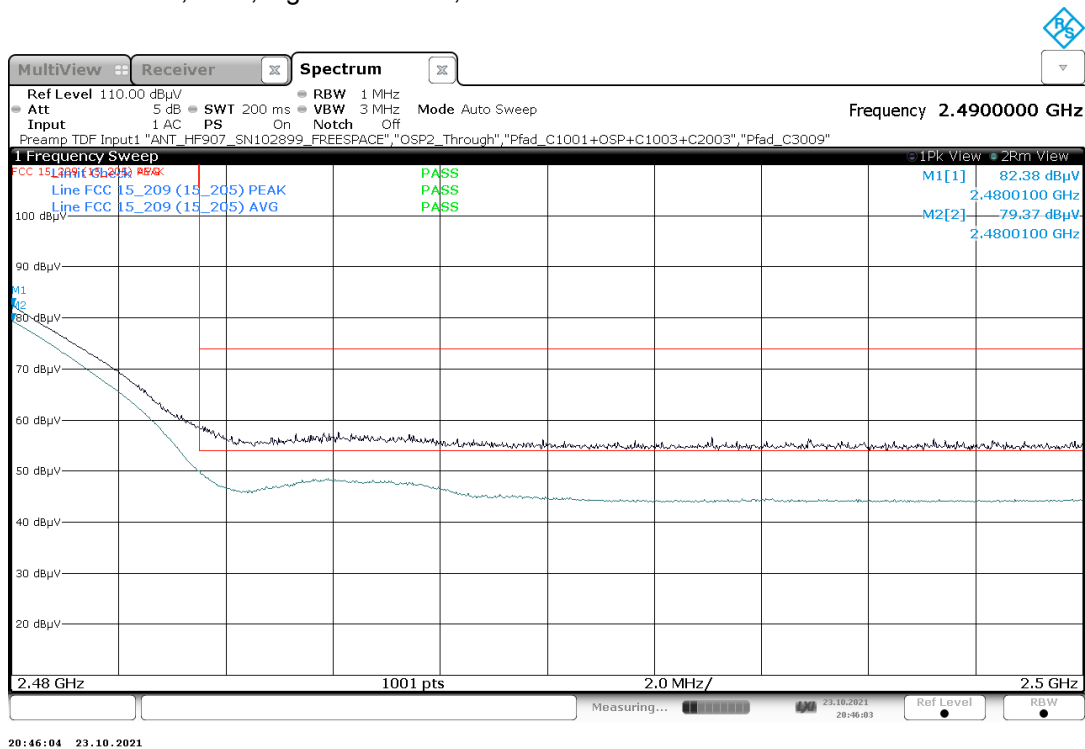
Plot 2: Mode 1, BEC, high channel 13, 2472 MHz
