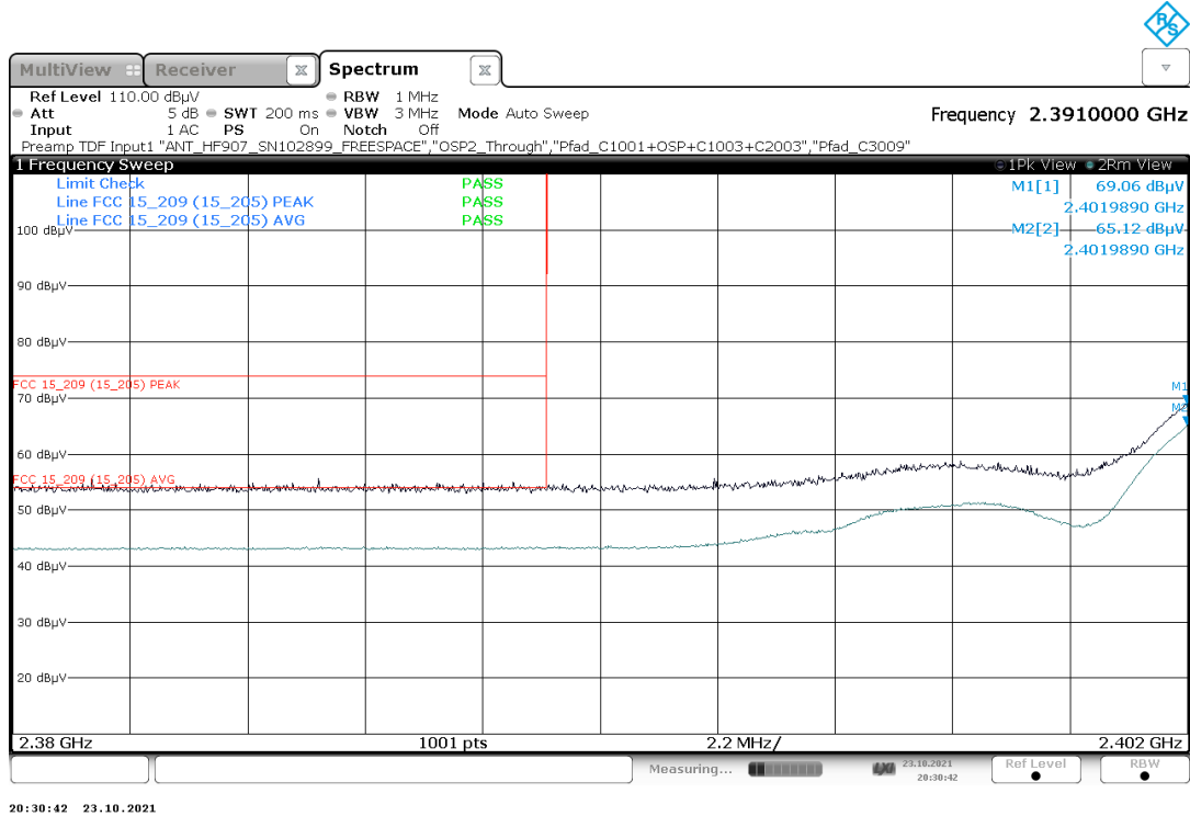
Plot 1: Mode 1, BEC, low channel 1, 2412 MHz
