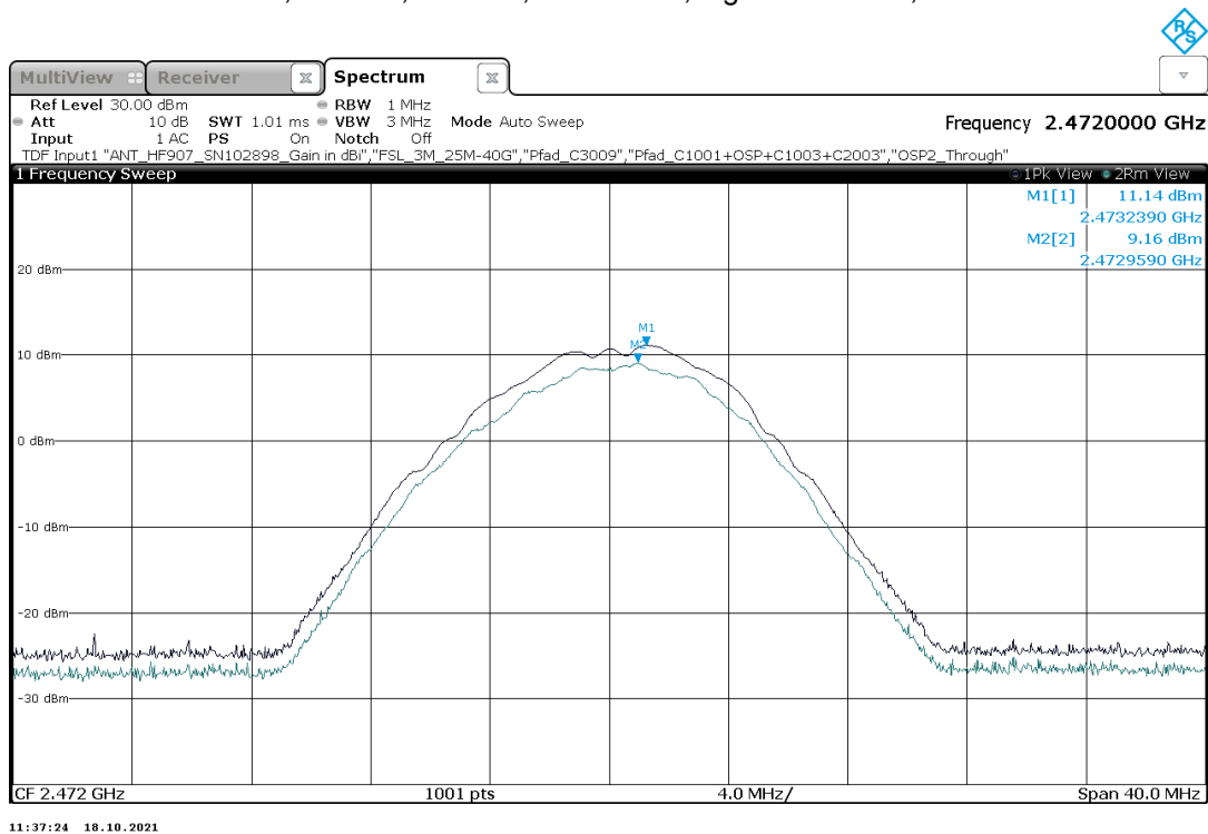
Plot 12: Test Mode 1, DBPSK, 1 Mbit/s, Peak EIRP, high channel 13, 2472 MHz
