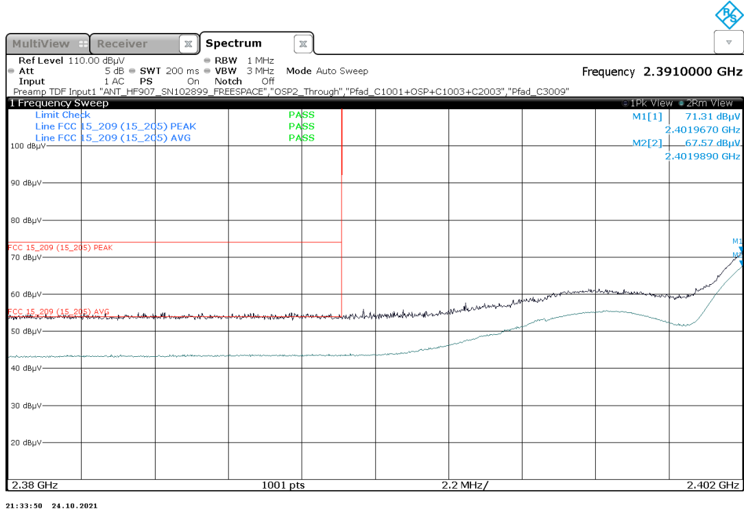
Plot 13: Mode 1, BEC, low channel 1
