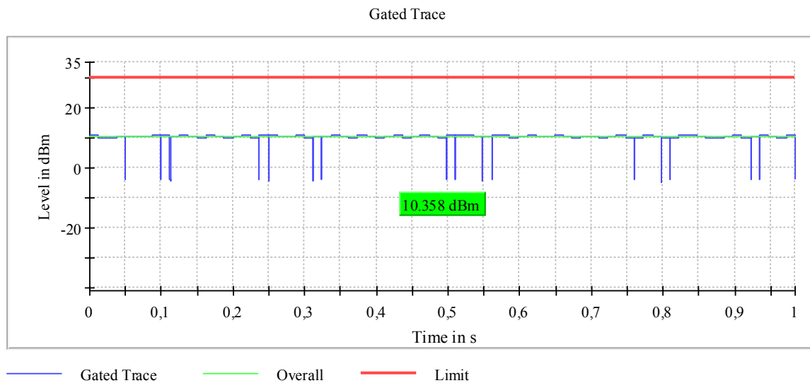
Plot 35: Mode 1, AVGPM-G Gated Average Power Measurement, high channel
