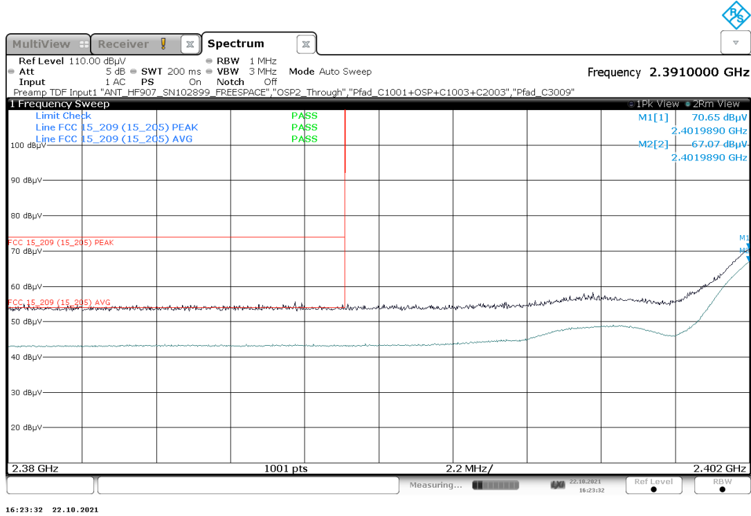
Plot 23: Mode 1, BEC, low channel 1
