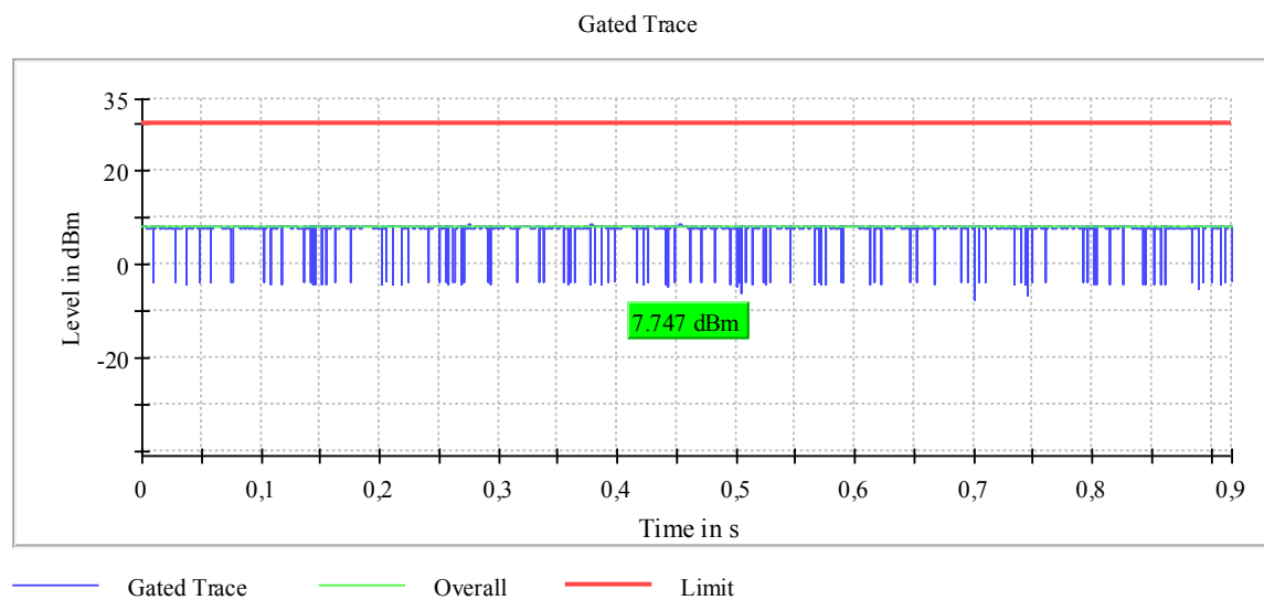
Plot 40: Mode 3, AVGPM-G Gated Average Power Measurement, mid channel
