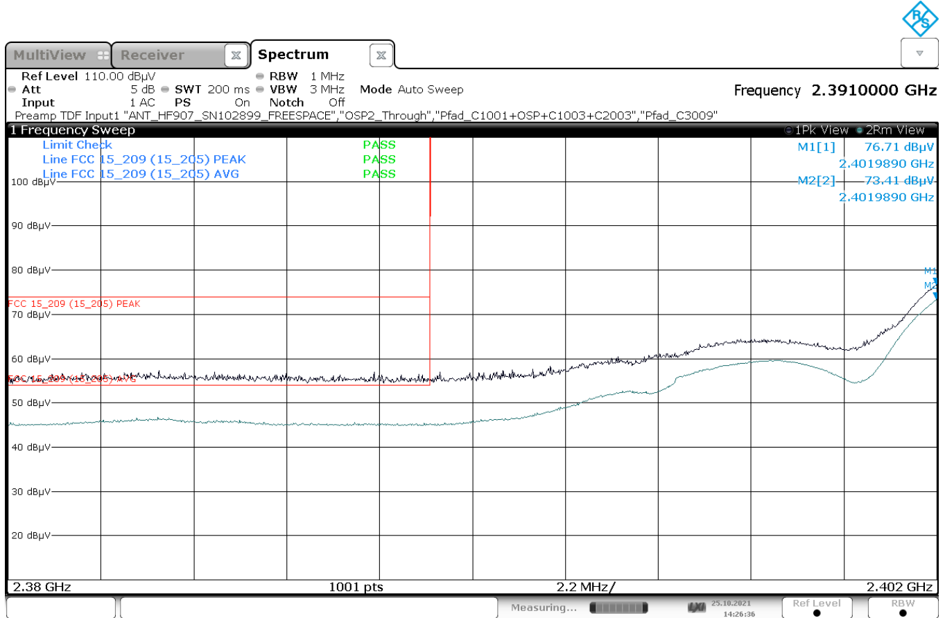
Plot 12: Mode 1, BEC, low channel 1
