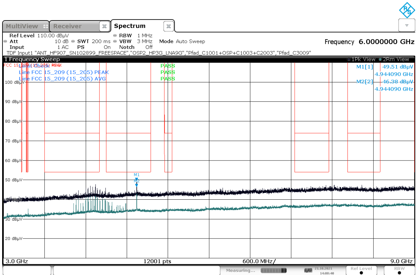
Plot 52: Mode 1, RSE 3 GHz – 9 GHz, high channel, horizontal / vertical polarisation
