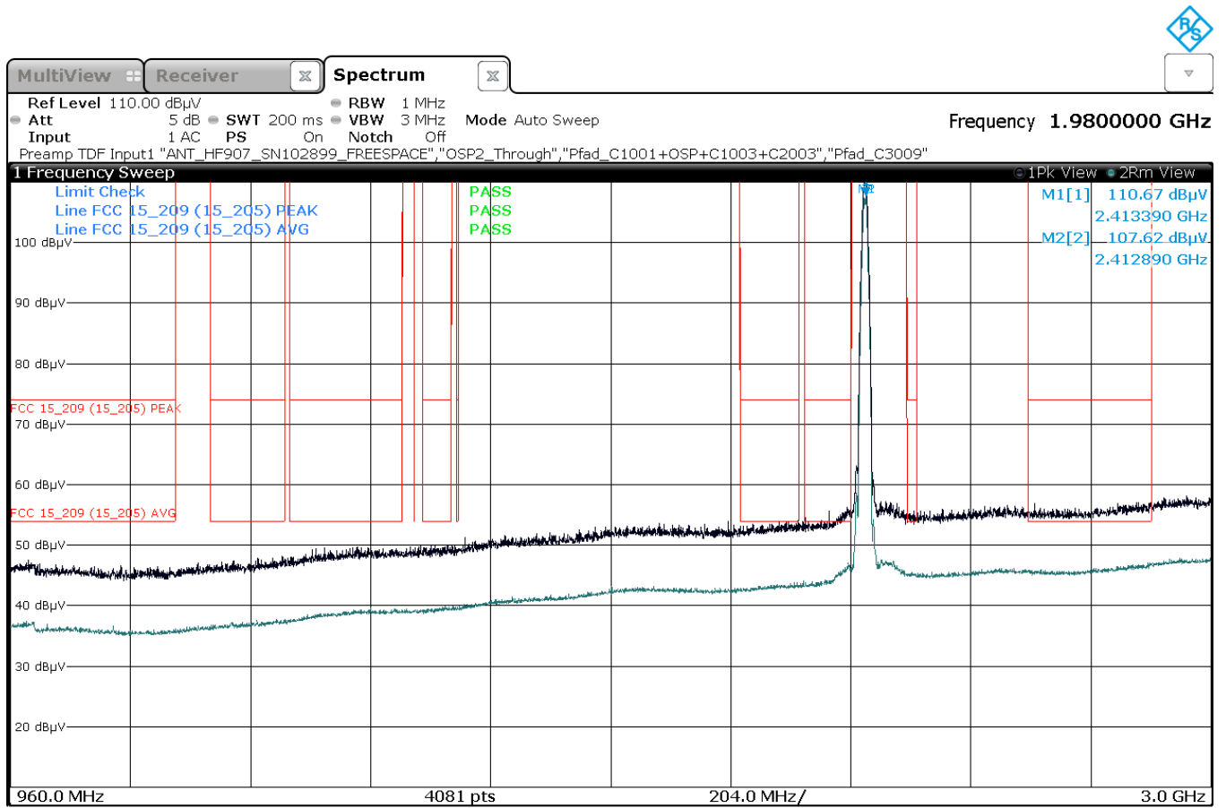
Plot 28: Mode 1, RSE 1 GHz – 3 GHz, low channel, horizontal / vertical polarisation
