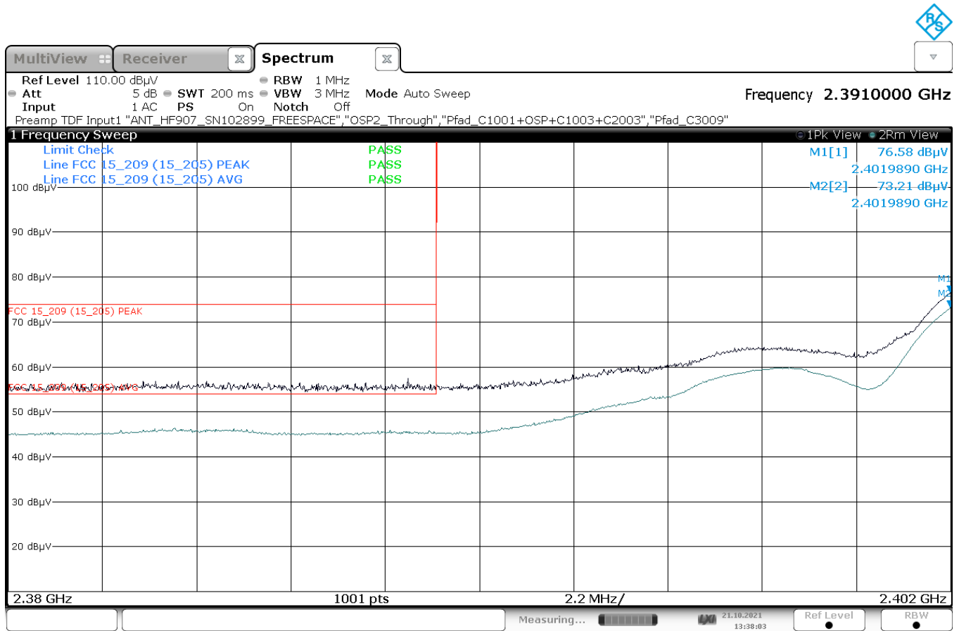
Plot 43: Mode 1, BEC, low channel 1
