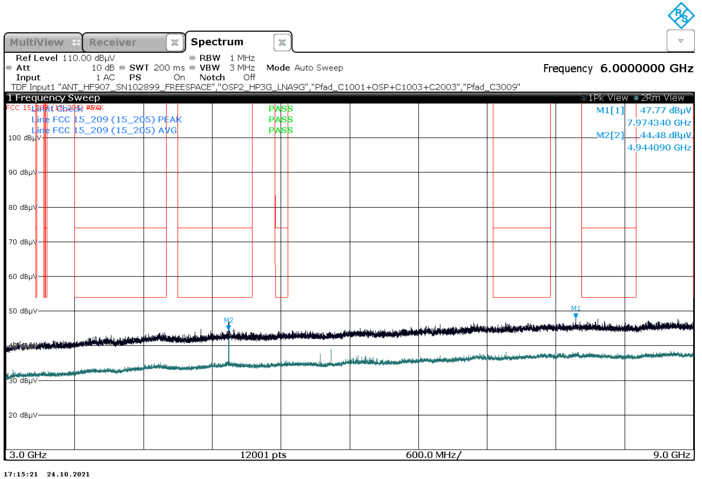
Plot 31: Mode 1, RSE 3 GHz – 9 GHz, high channel, horizontal / vertical polarisation
