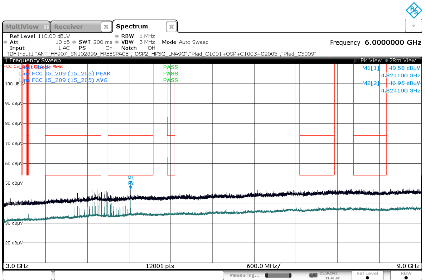
Plot 51: Mode 1, RSE 3 GHz – 9 GHz, low channel, horizontal / vertical polarisation
