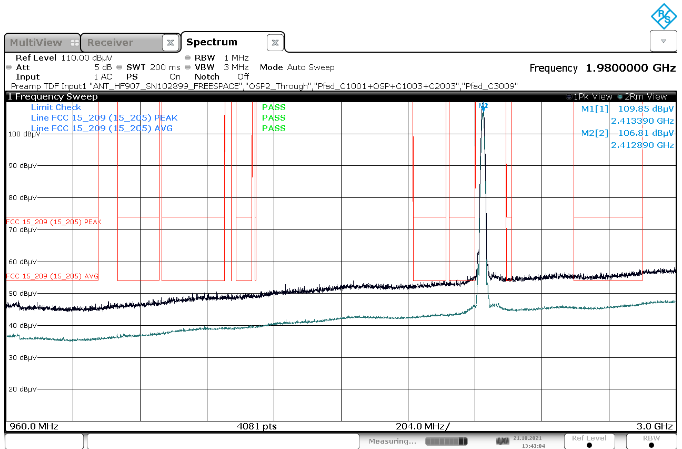
Plot 49: Mode 1, RSE 1 GHz – 3 GHz, low channel, horizontal / vertical polarisation
