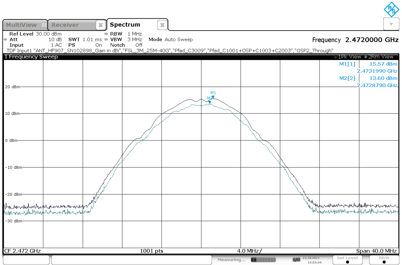
Plot 42: Test Mode 1, DBPSK, 1 Mbit/s, Peak EIRP, high channel 13, 2472 MHz
