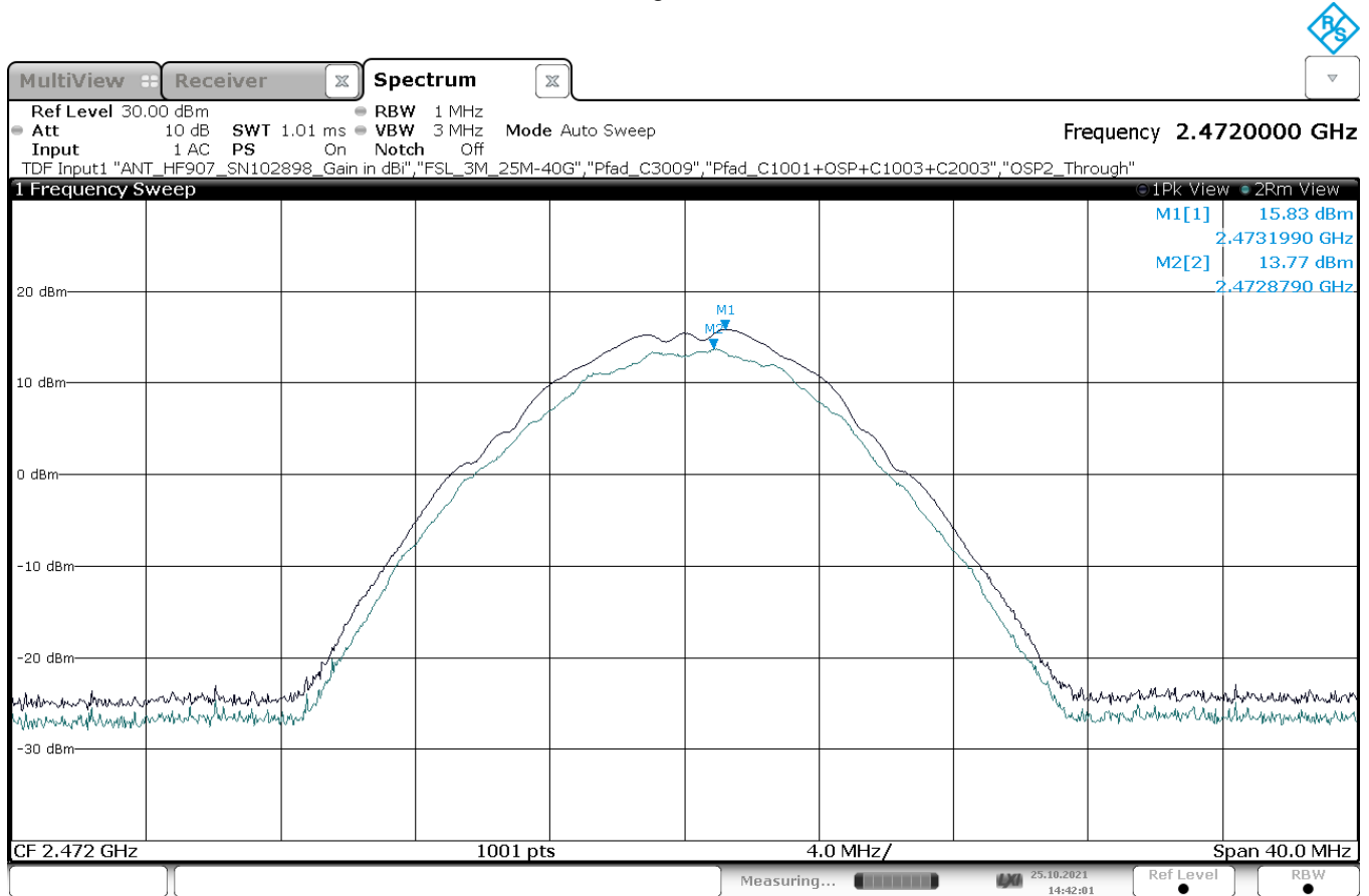
Plot 11: Test Mode 1, DBPSK, 1 Mbit/s, Peak EIRP, high channel 13, 2472 MHz
