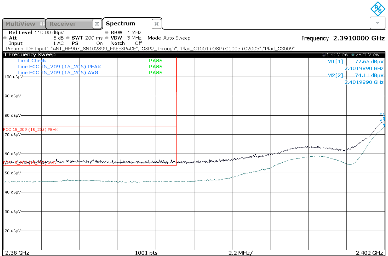
Plot 22: Mode 1, BEC, low channel 1
