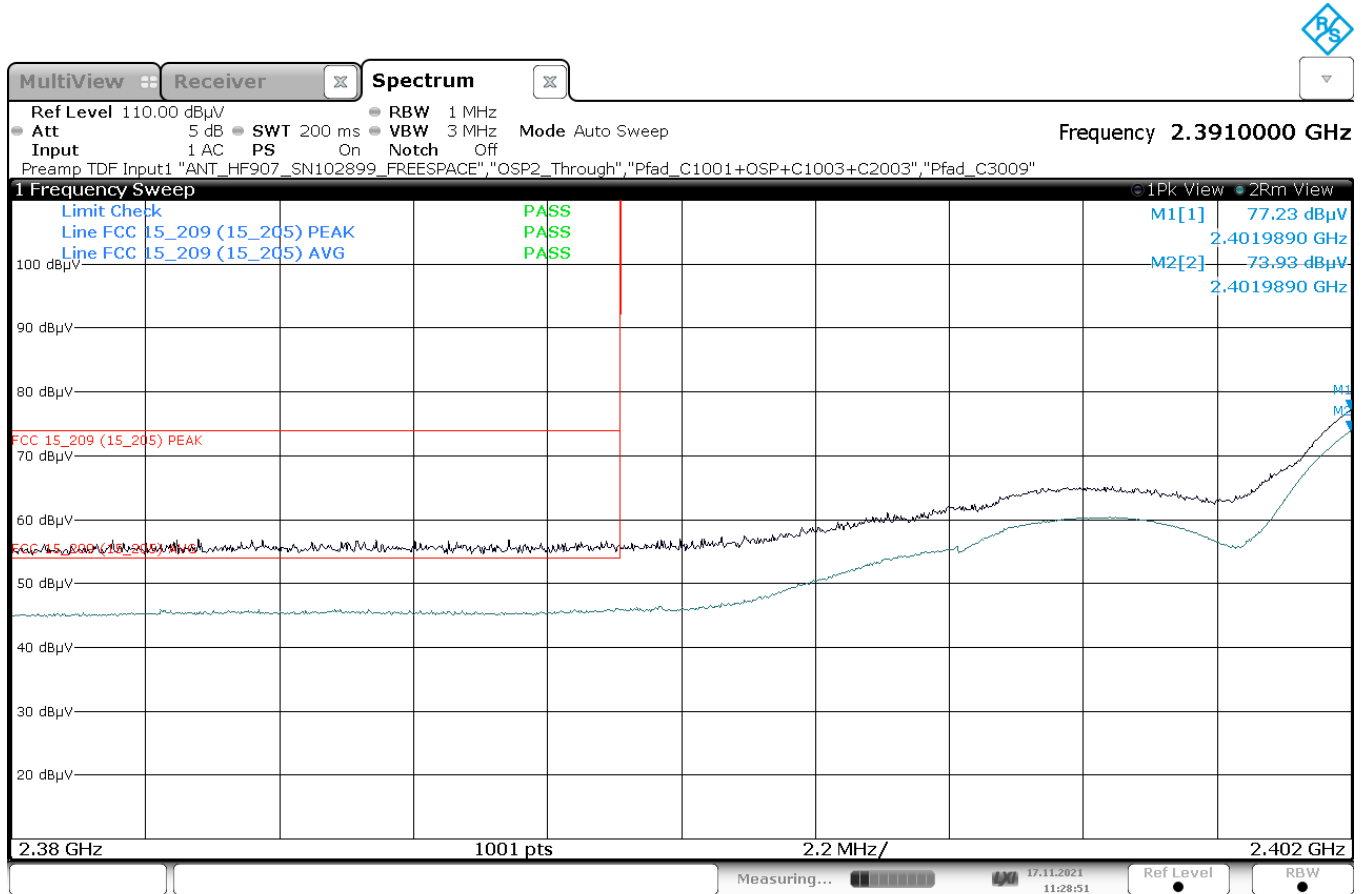
Plot 53: Mode 1, BEC, low channel 1
