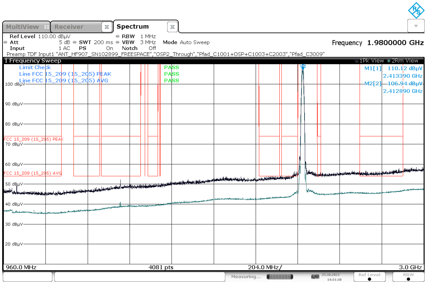
Plot 18: Mode 1, RSE 1 GHz – 3 GHz, low channel, horizontal / vertical polarisation
