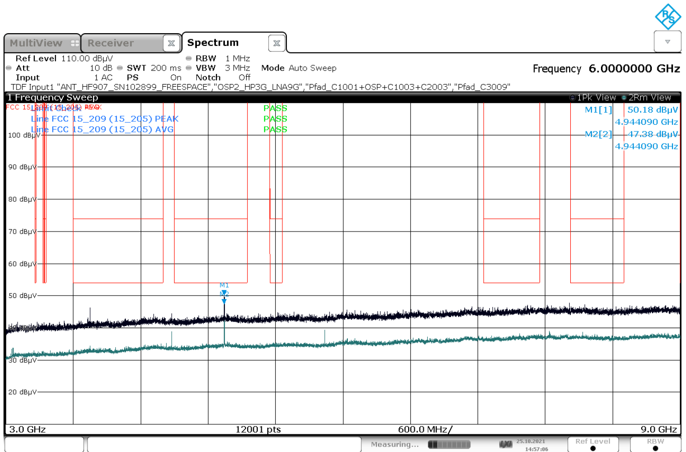
Plot 21: Mode 1, RSE 3 GHz – 9 GHz, high channel, horizontal / vertical polarisation
