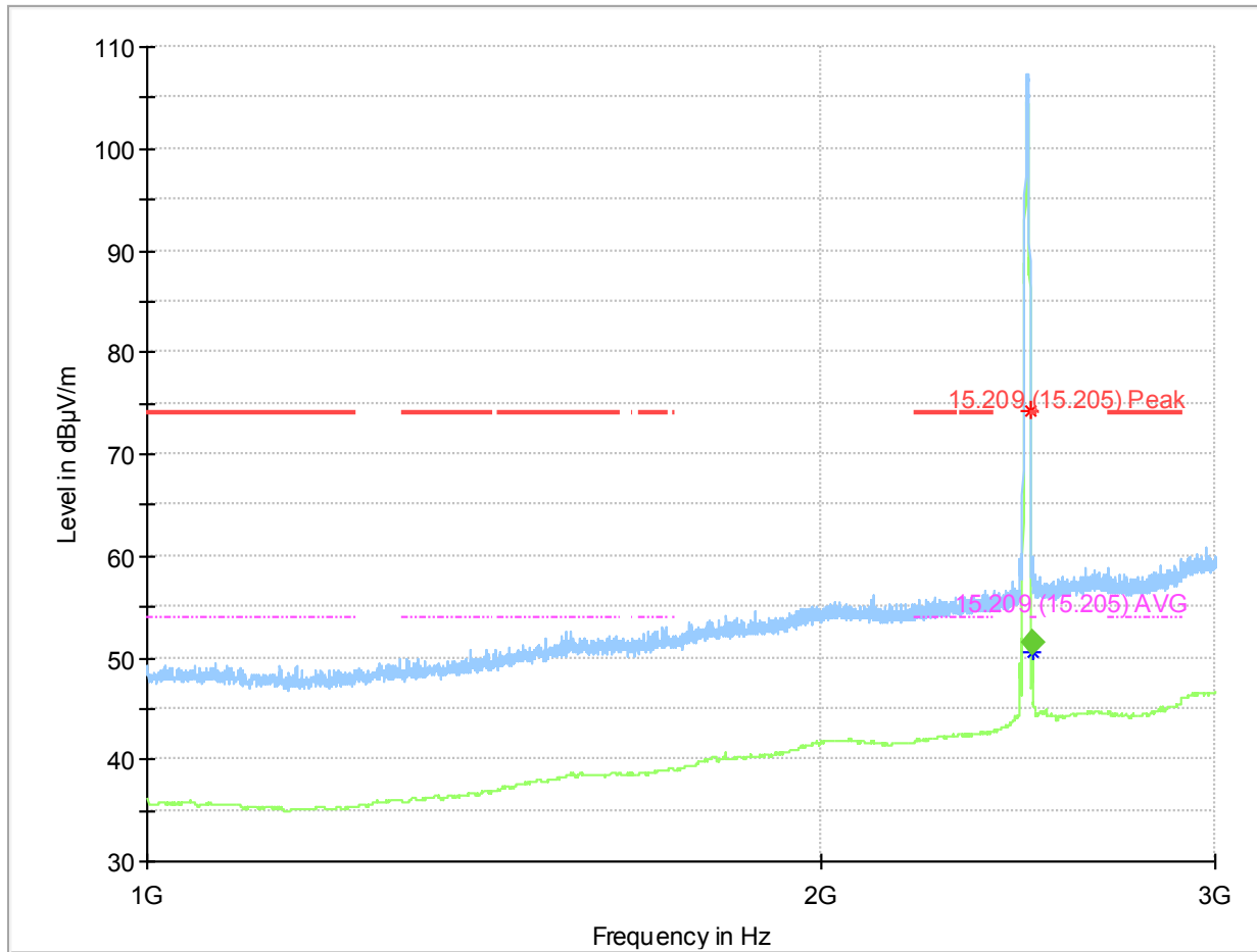
Plot 29: Mode 1, RSE 1 GHz – 3 GHz, high channel, horizontal / vertical polarisation
