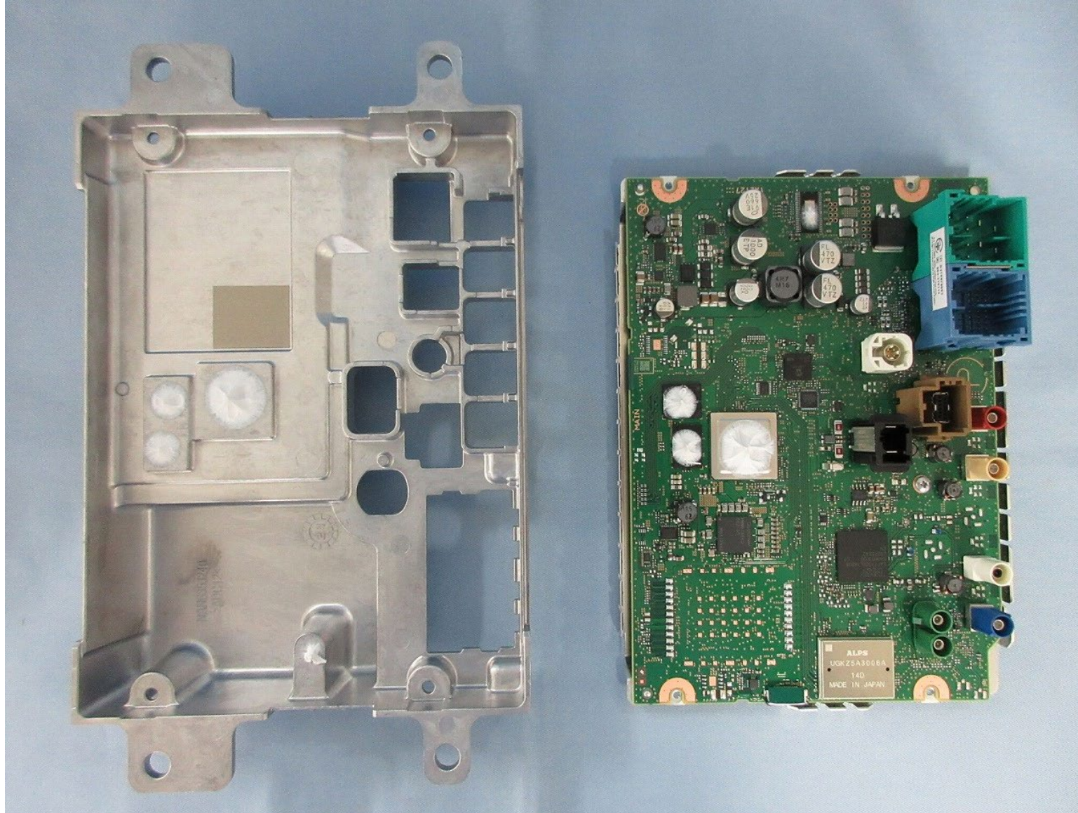
PCB-MAIN C-side
