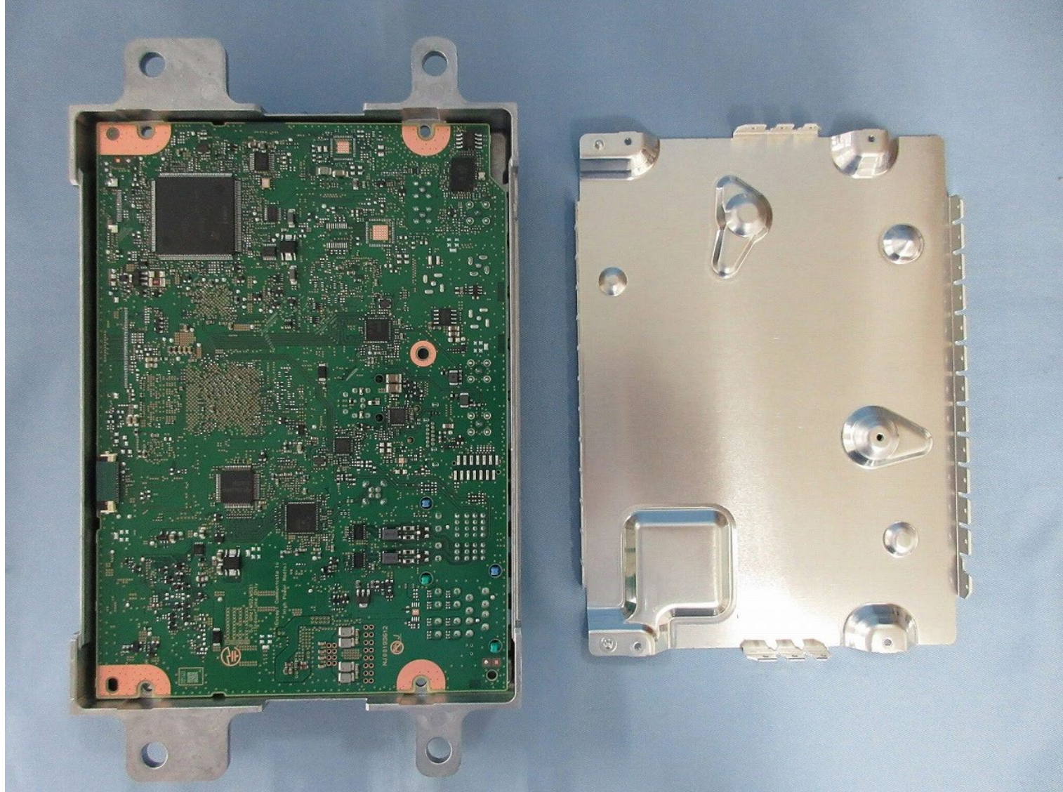
PCB-MAIN S-side
