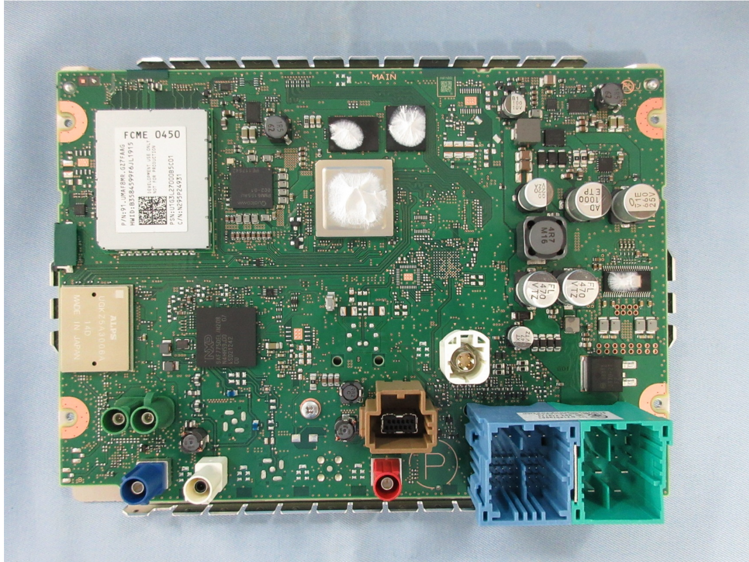
PCB-MAIN C-side
