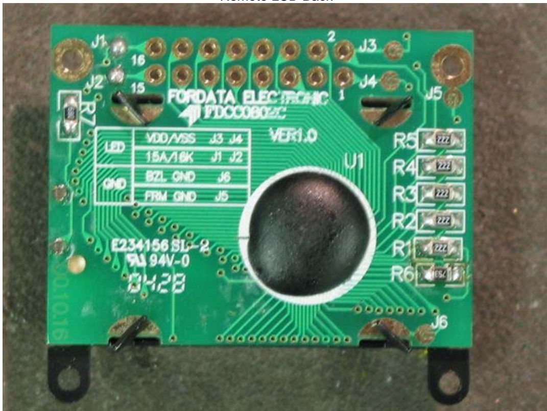
Remote LCD Back
