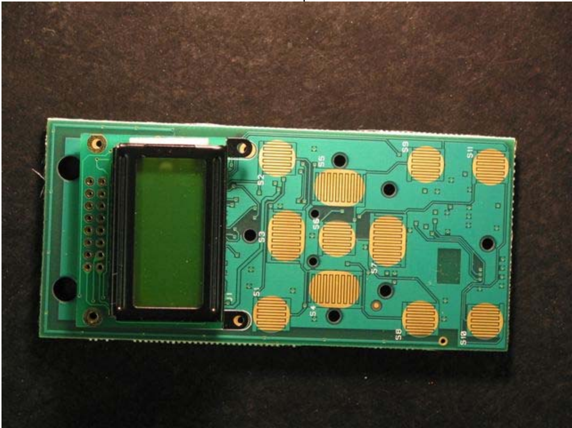
Remote PCB Top with LCD
