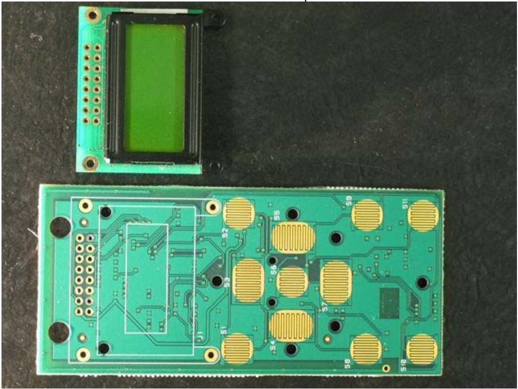
Remote PCB Bottom
