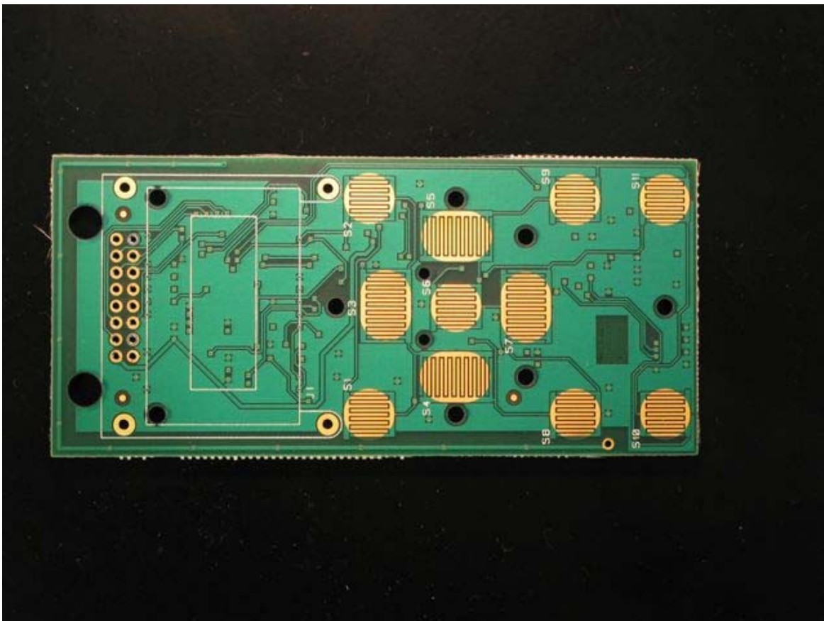
Remote PCB Top No LCD
