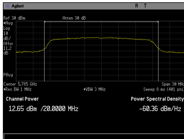
Plot 6. Maximum Conducted Output Power, BW 20M, Ch 5785M, 80211n, MSC24, P3230, CH0
