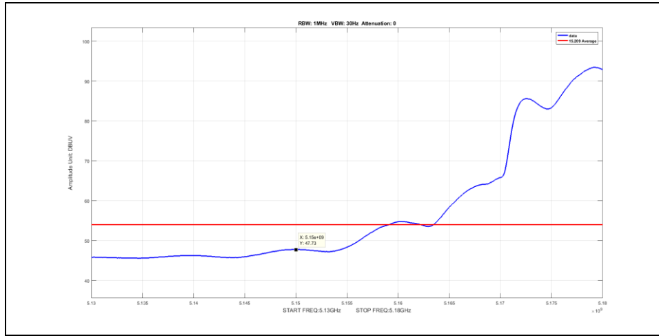
Plot 67. Average Band Edge Spurious, BW 20M, Ch. 5180M, 80211a, MCS0, P3230
