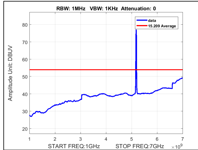
Plot 43. Average Spurious Emission, 1-7 GHz, BW 20M, Ch. 5180M, 80211ac, MCS24, P3230
