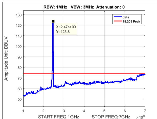
Plot 88. Radiated Spurious Emissions, High Channel, 802.11n 20 MHz, 1 GHz – 7 GHz, Peak
