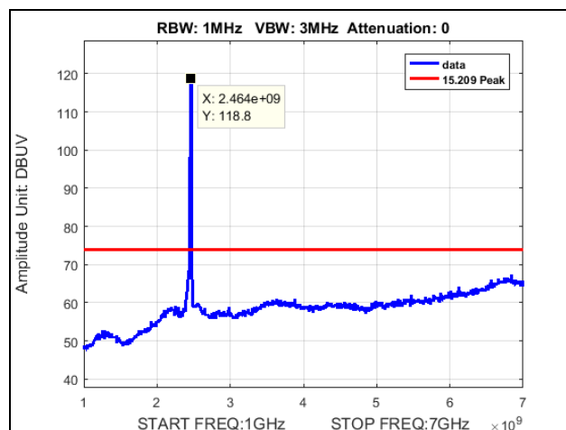
Plot 76. Radiated Spurious Emissions, High Channel, 802.11b 20 MHz, 1 GHz – 7 GHz, Peak
