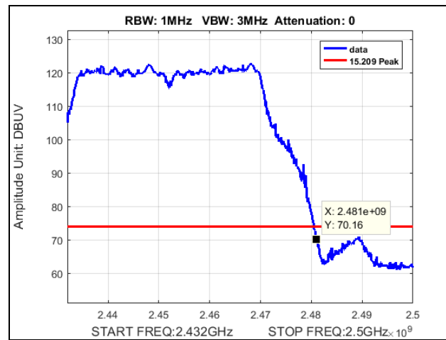
Plot 110. Radiated Restricted Band Edge, High Channel, 802.11n 40 MHz, Peak
