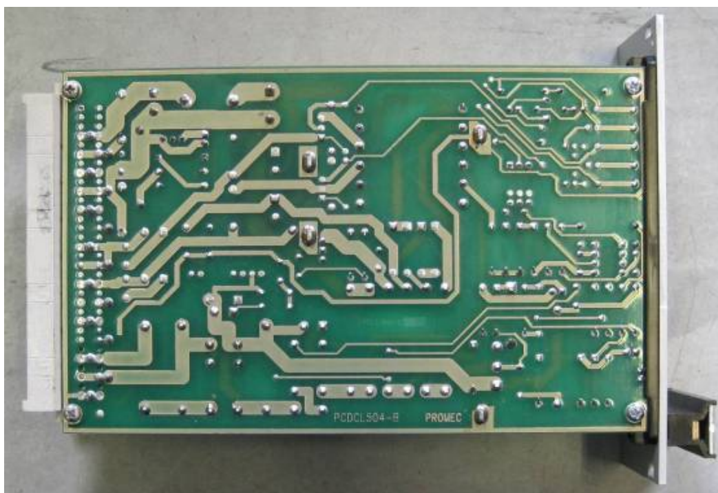
Fig. 10: Battery Charger STD 482 (Bottom Side)
