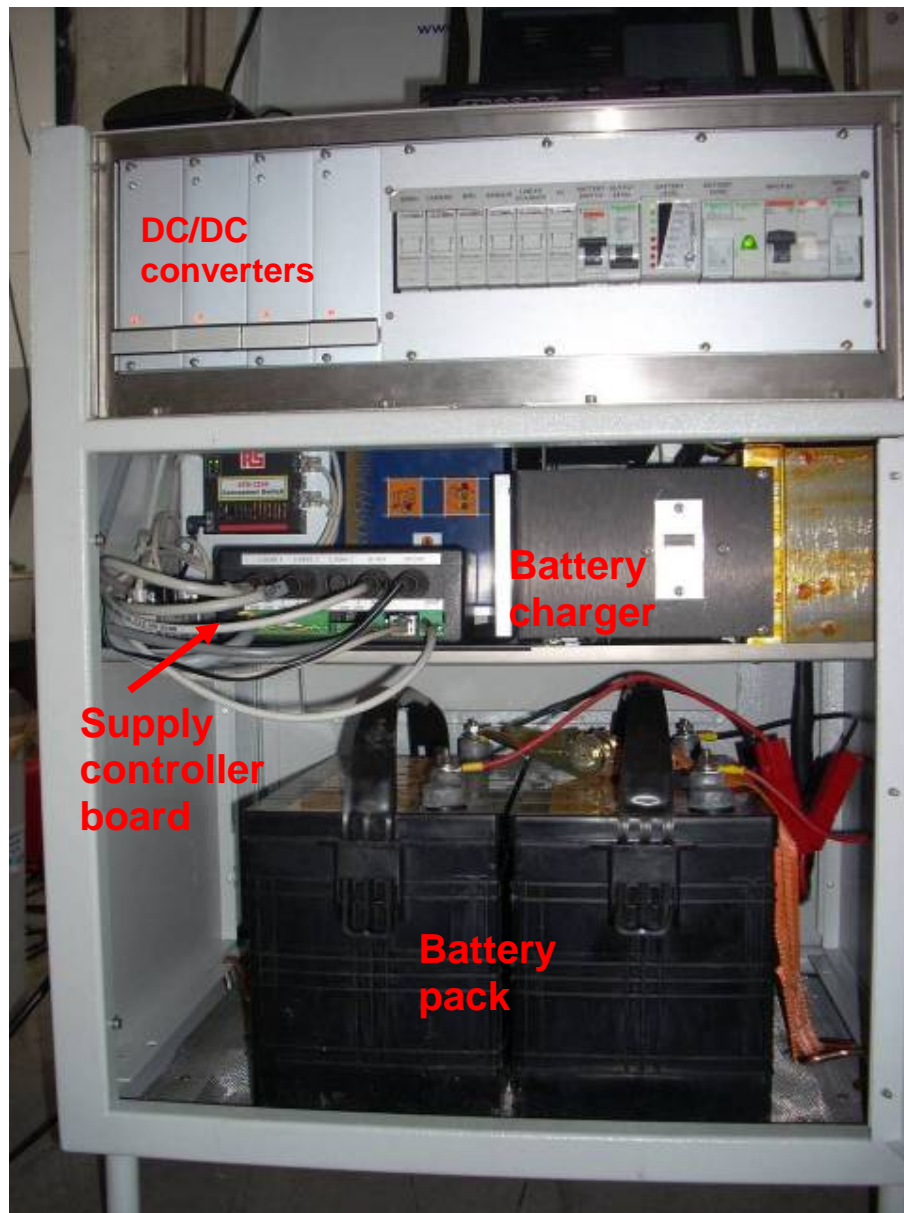
Fig. 3: Supply Unit Front part
