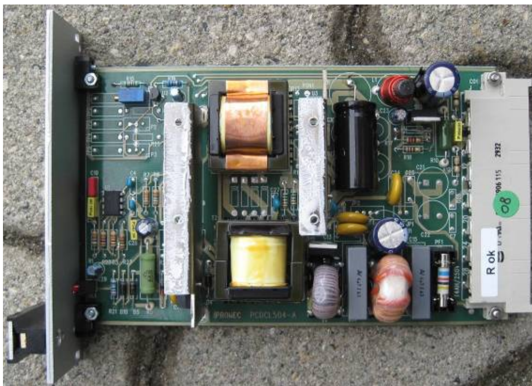
Fig. 9: Battery Charger STD 482 (Top Side)
