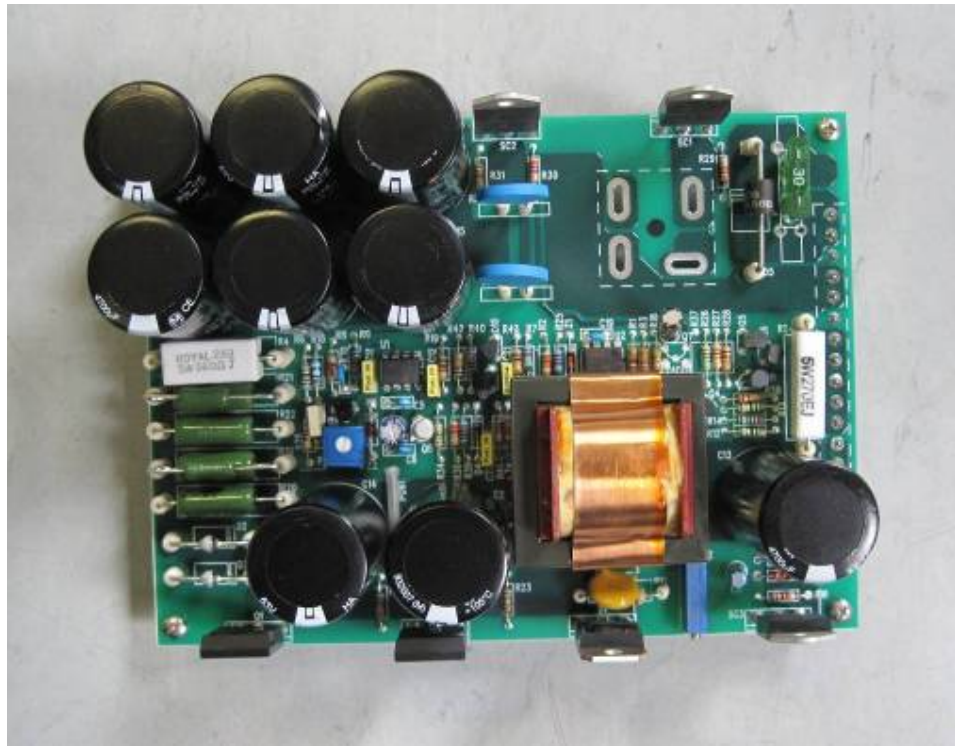
Fig. 11: DC/DC converters (top side)
