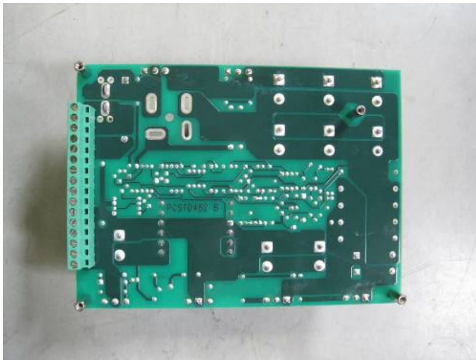
Fig. 12: DC/DC converters (bottom side)
