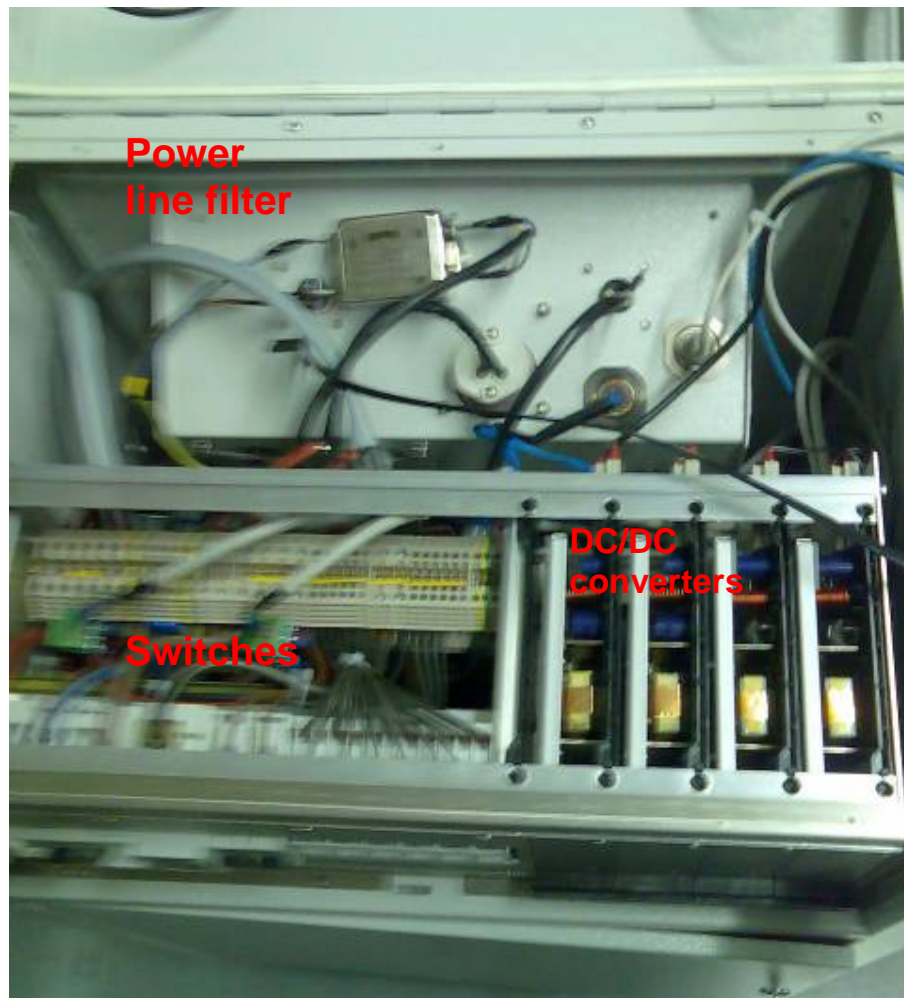
Fig. 2: Supply Unit Top View (PC housing)
