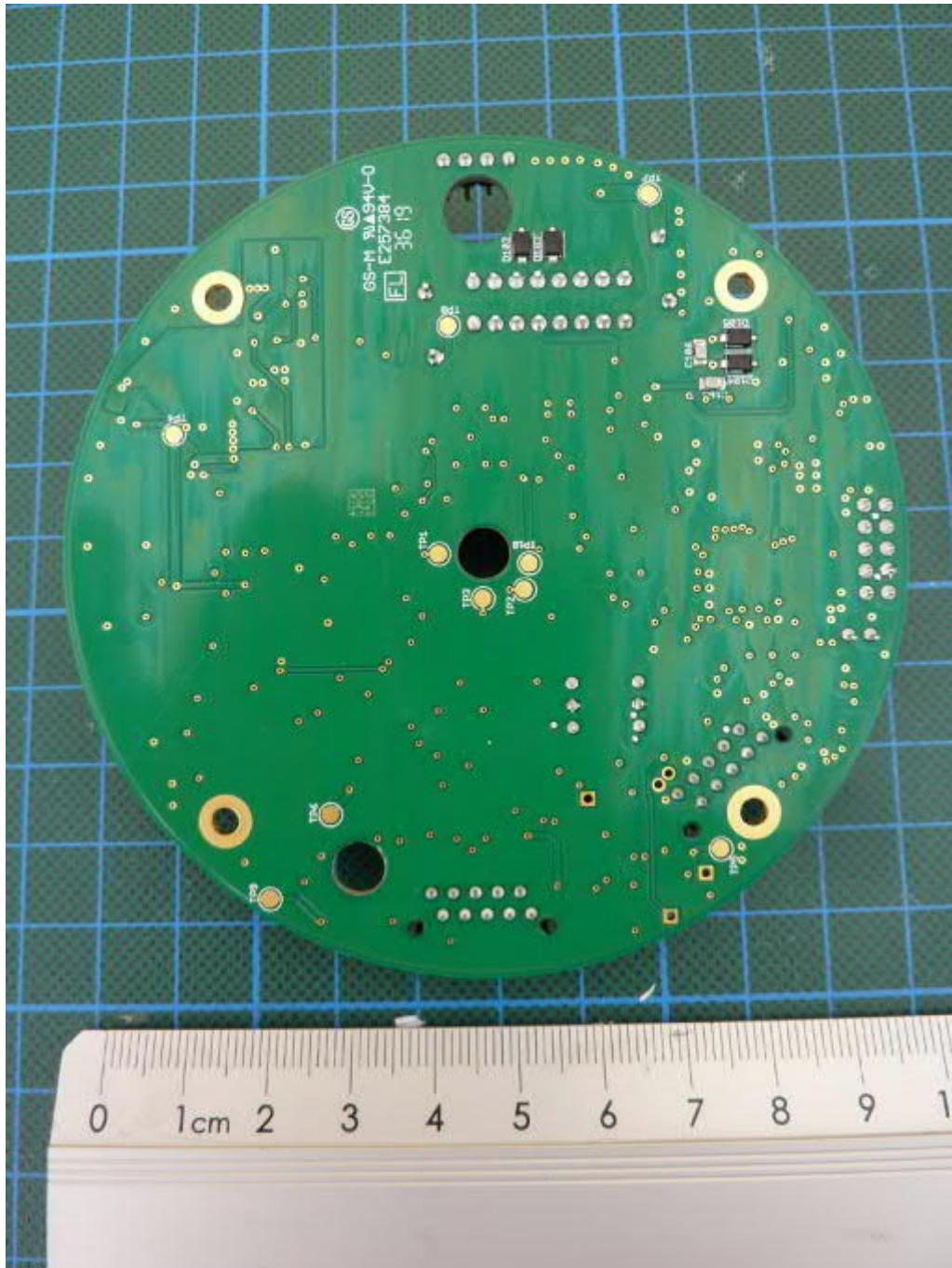
WS600-UMB, main PCB, bottom view
