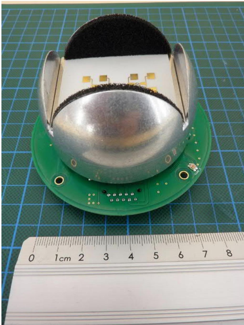
WS600-UMB, radar part, total view
