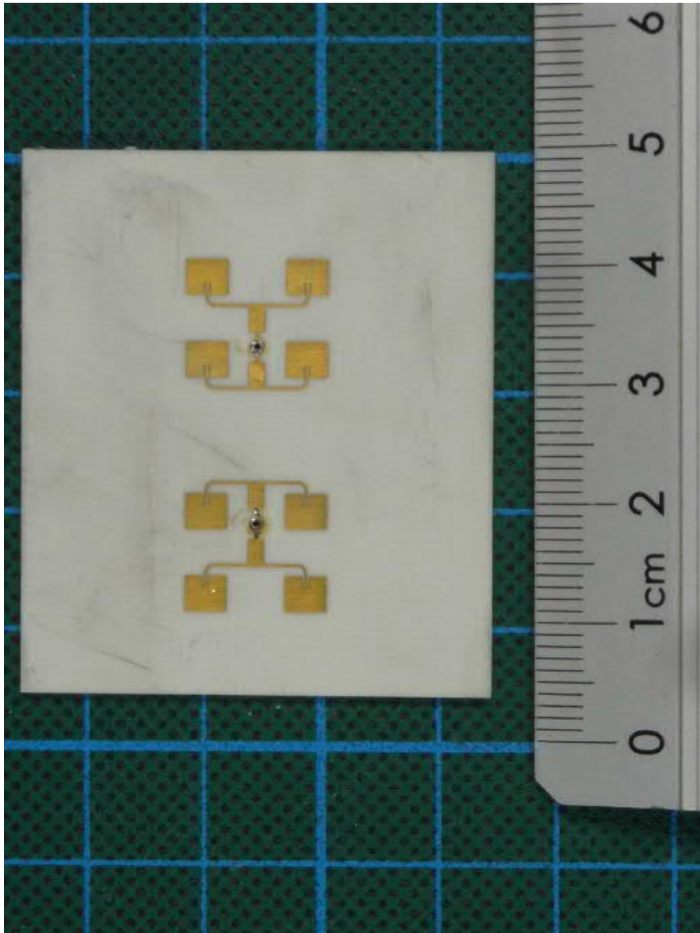
WS600-UMB, radar module, antenna PCB, top view
