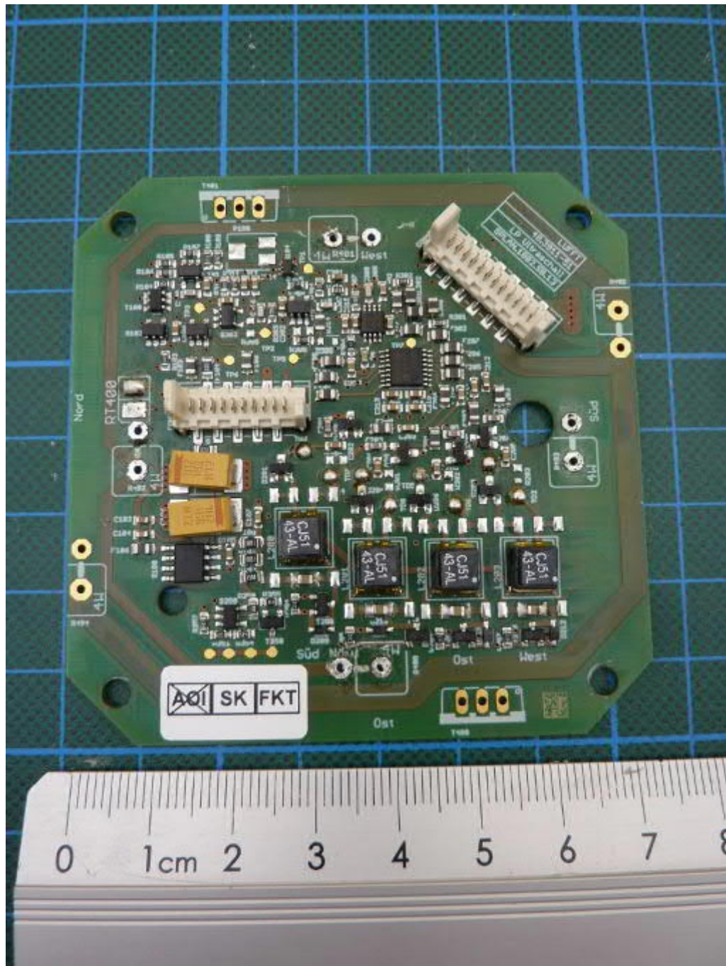
WS600-UMB, ultra sonic PCB, top view
