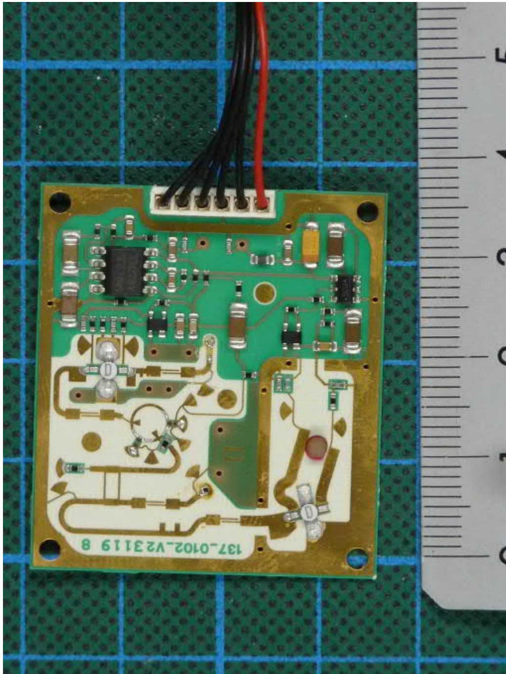
WS600-UMB, radar module, PCB, top view
