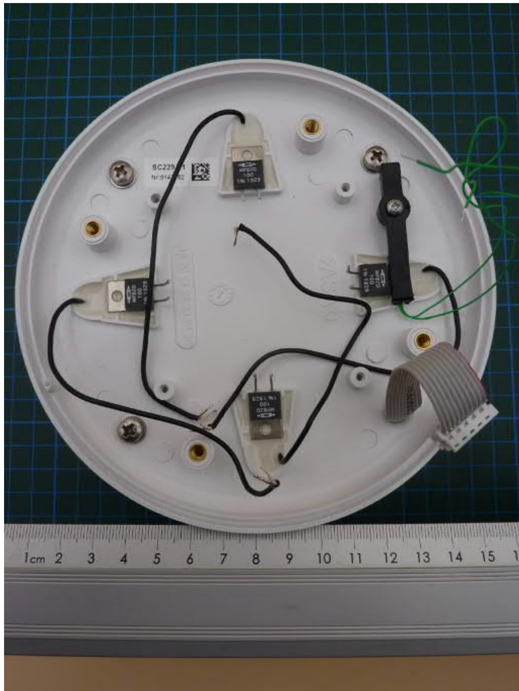
WS600-UMB, housing, ultra sonic PCB removed
