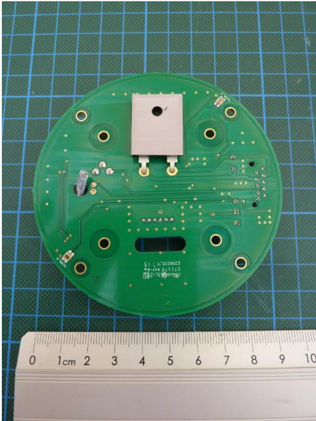
WS600-UMB, radar carrier PCB, bottom view
