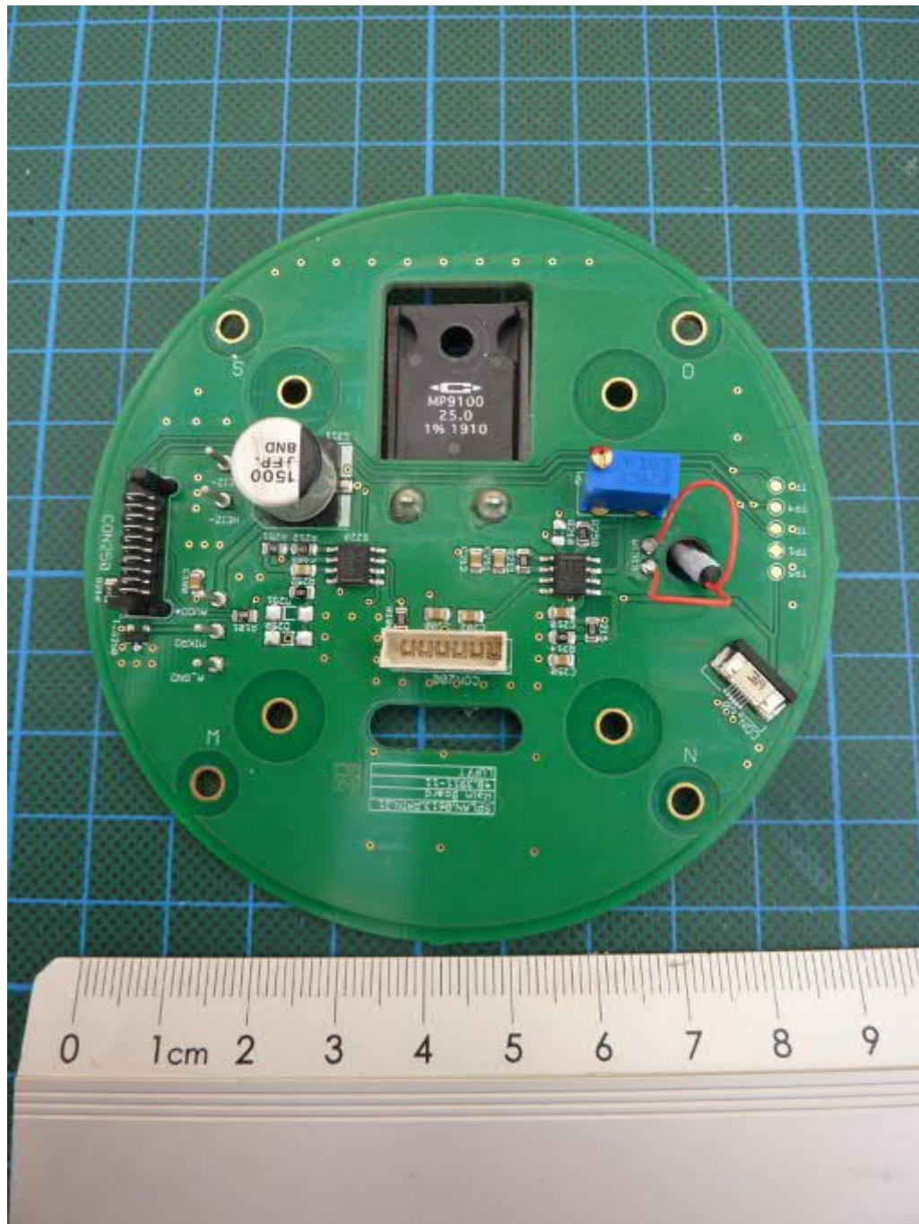
WS600-UMB, radar carrier PCB, top view
