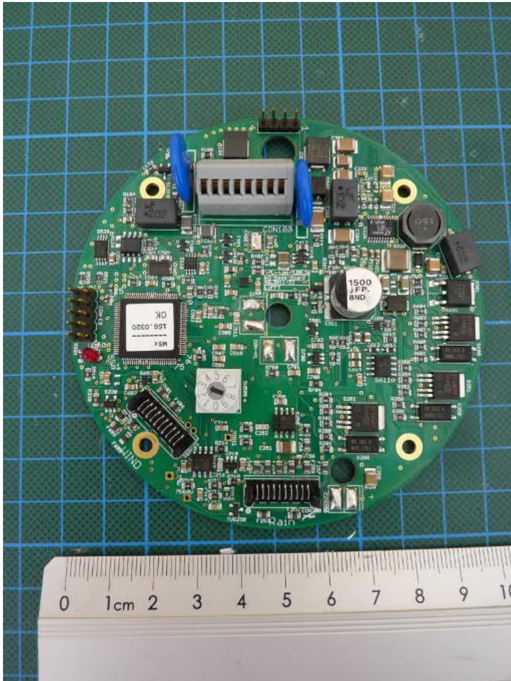
WS600-UMB, main PCB, top view
