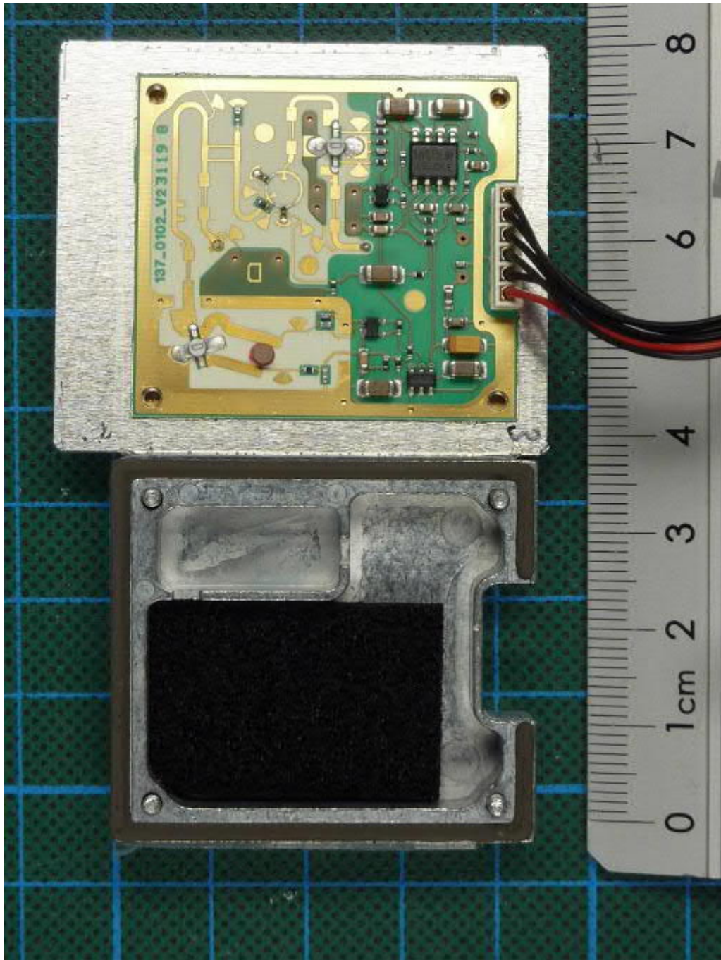
WS600-UMB, radar module, internal view
