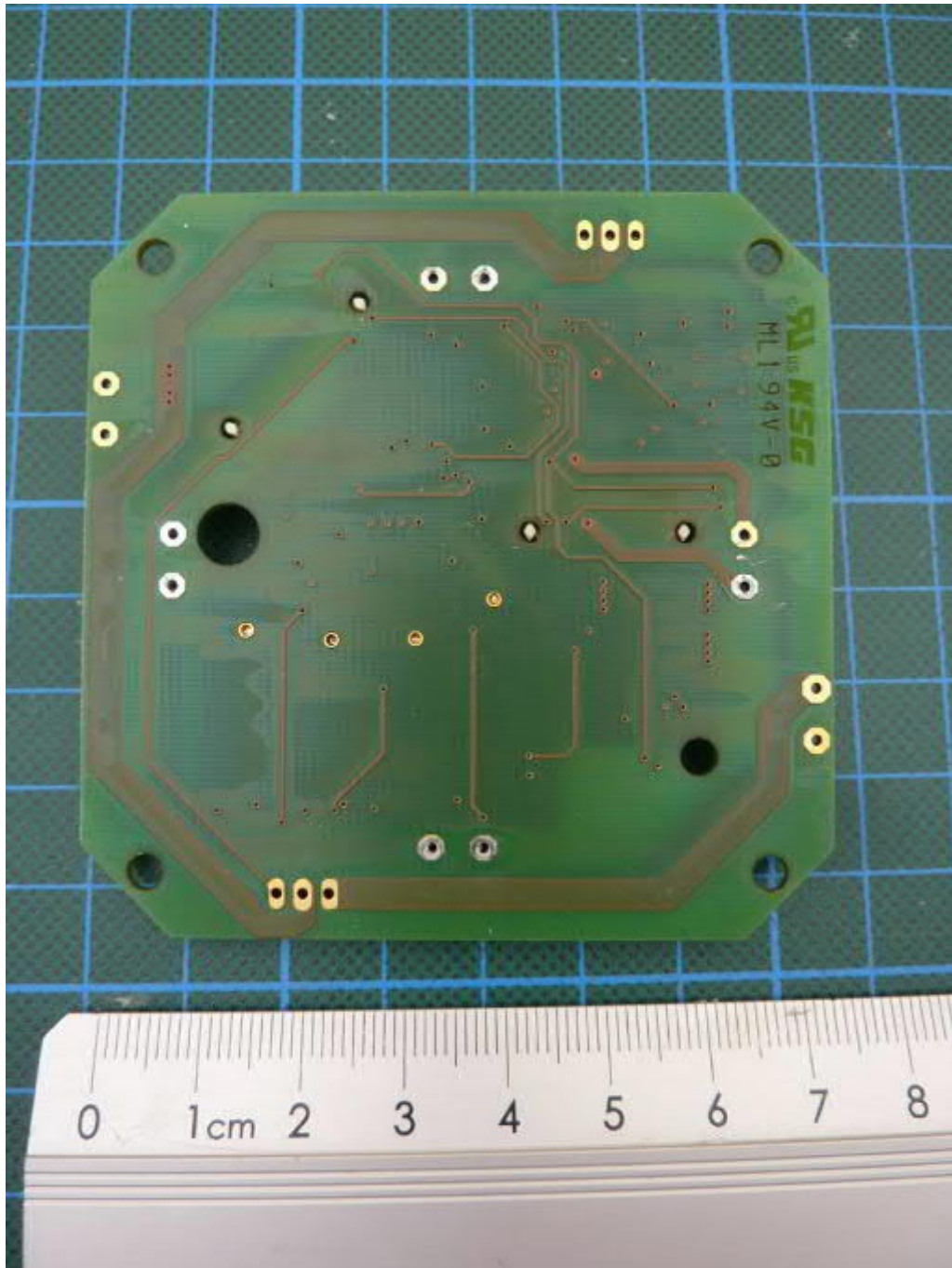
WS600-UMB, ultra sonic PCB, bottom view
