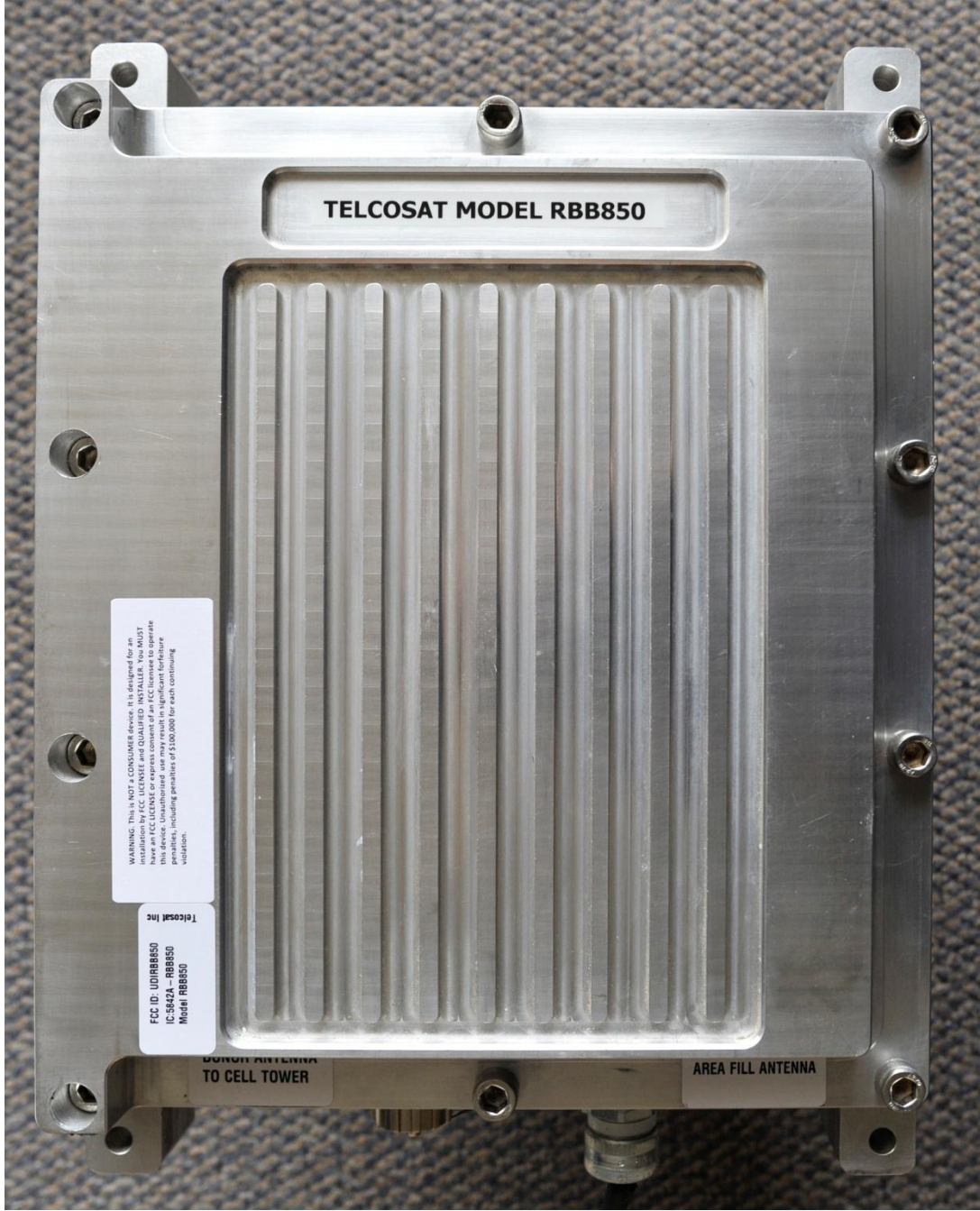
FRONT OF REPEATER WITH COVER PLATE ATTACHED
