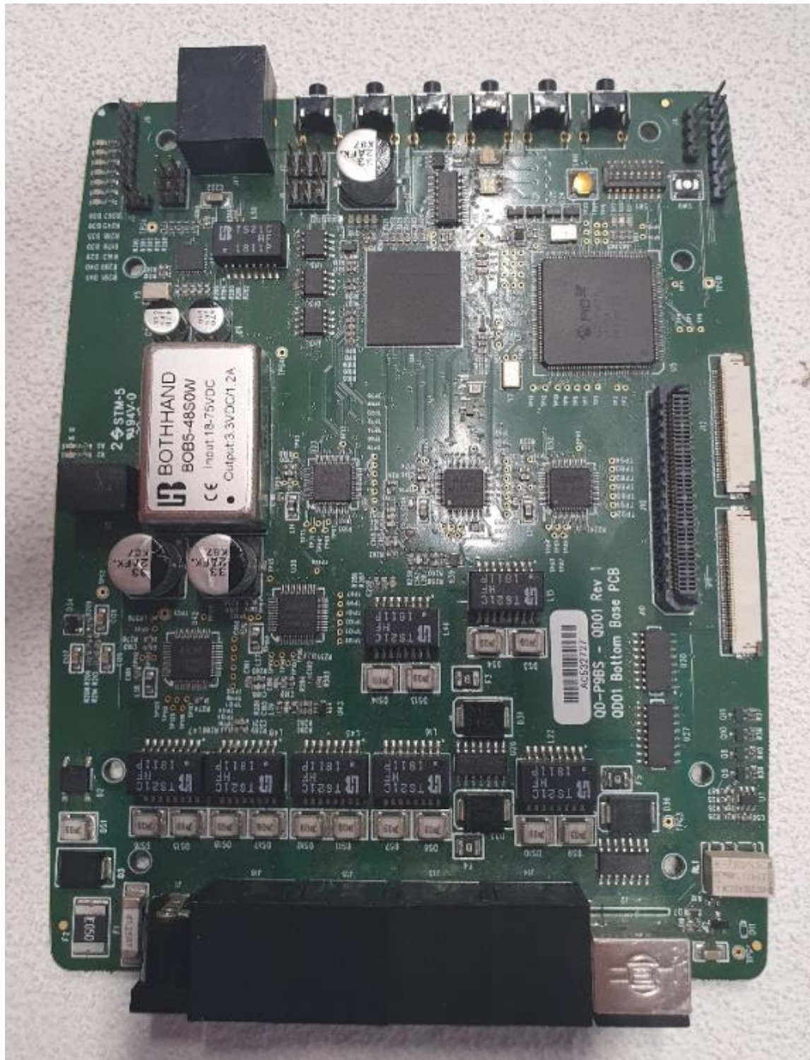
QD01 Main control board
