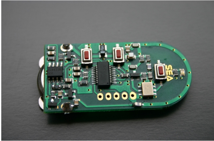
Internal component side
