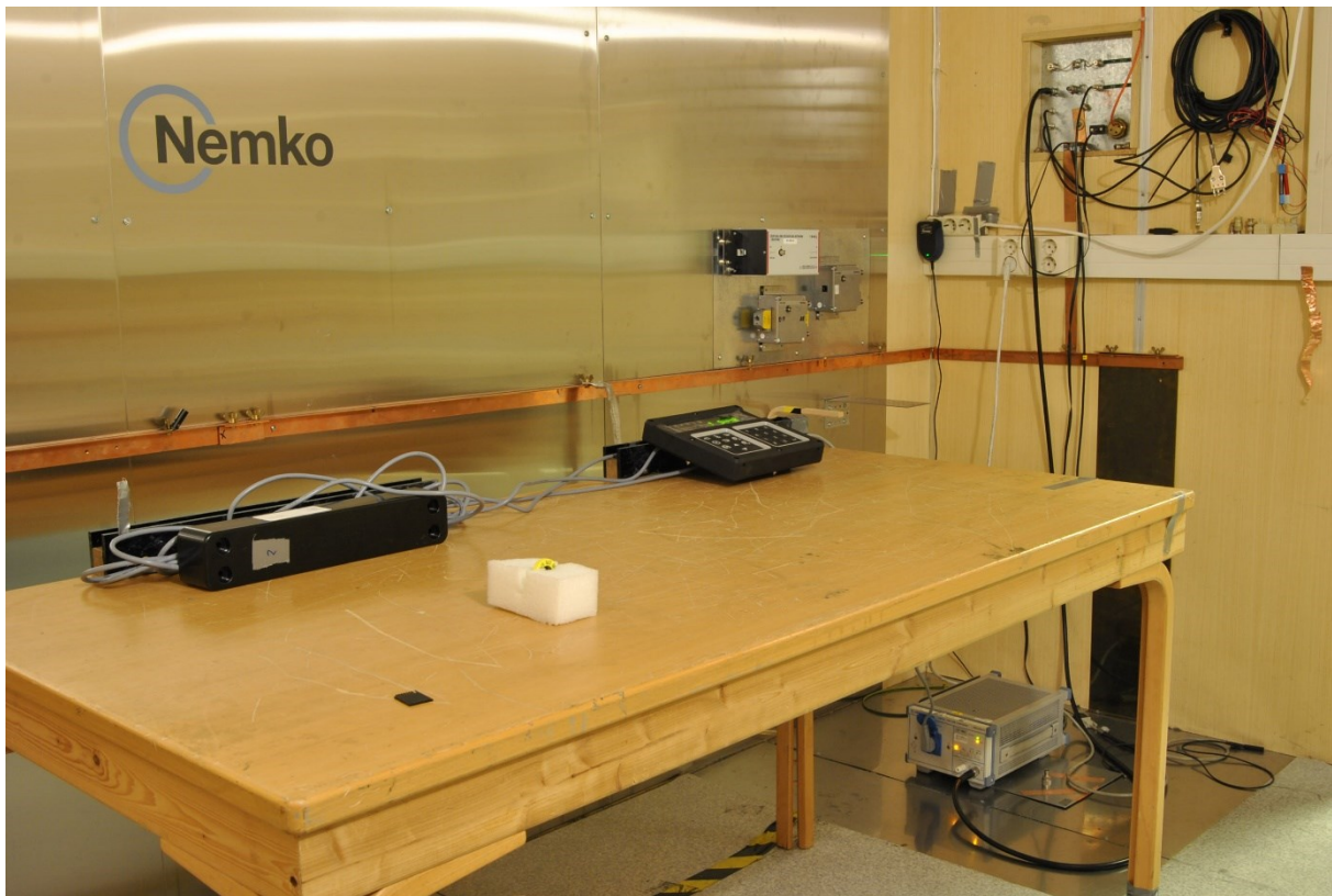
Conducted Emissions
