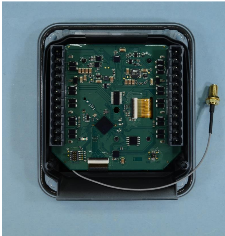
EUT for Conducted Emissions, "Back"
