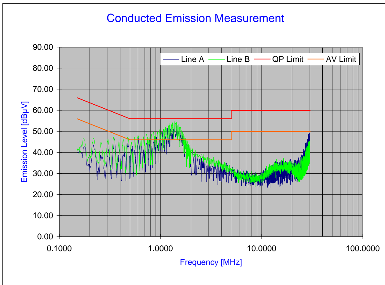
Plot 6-18. Line Conducted Plot with 802.11g
