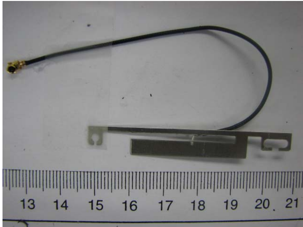
WiFi Antenna
