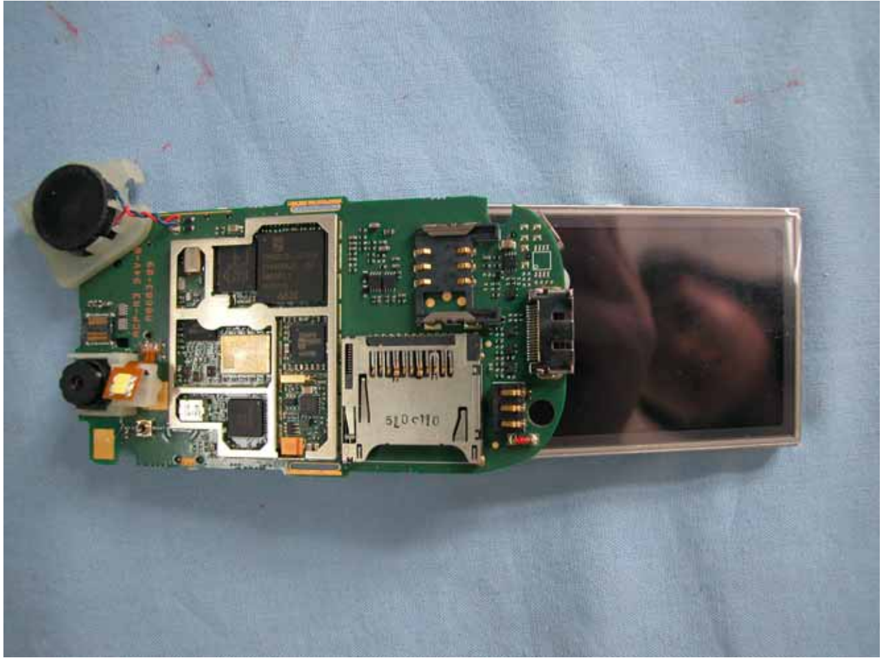
Pic 9 PW-1010 Internal Photo
