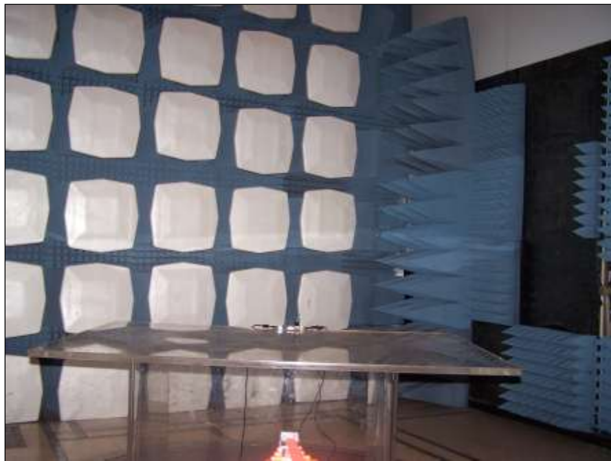
Photograph 4. Radiated Emissions, Monopole, Type II, Test Setup, Below 1 GHz
