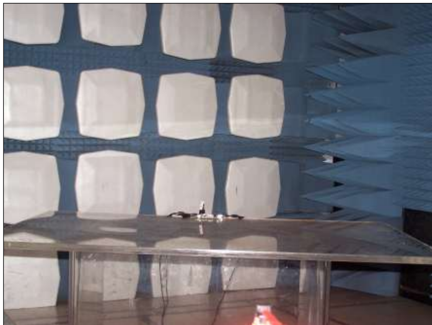
Photograph 2. Radiated Emissions, Monopole, Type I, Test Setup, Below 1 GHz
