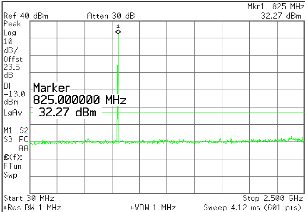
Figure 7-1: Out of Band emission at antenna terminals – GSM CH Low
