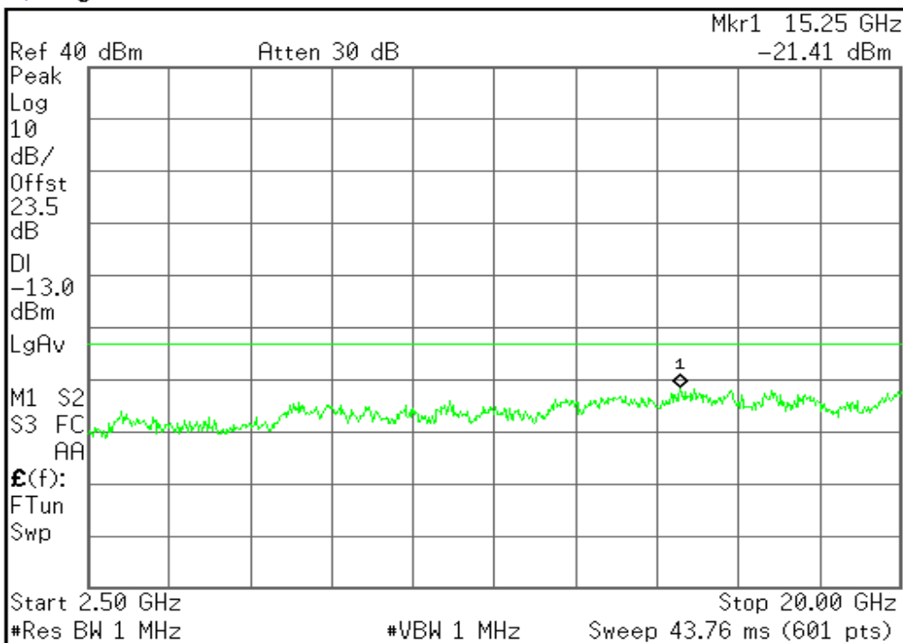
Figure 7-2: Out of Band emission at antenna terminals – GSM CH Low
