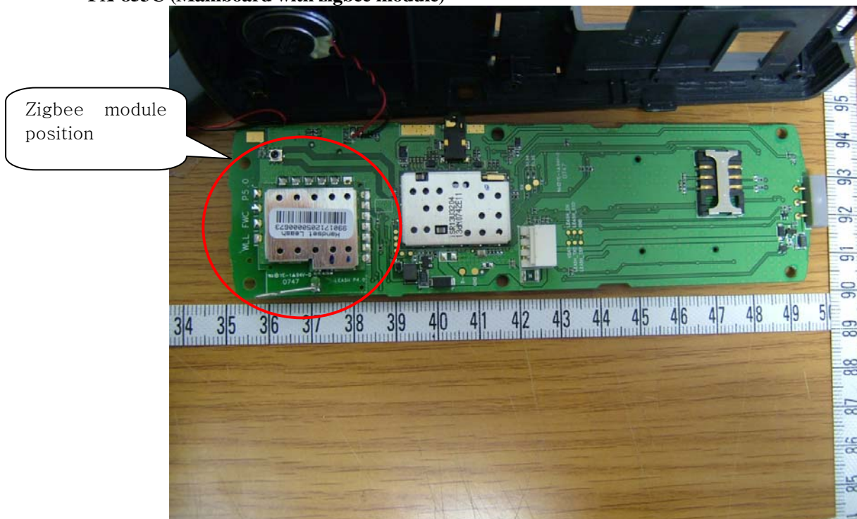
FX-853C (Mainboard with zigbee module)
