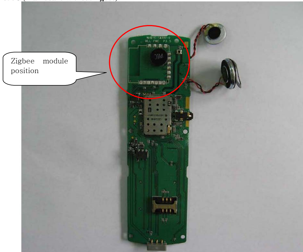
FX-853C (Mainboard with zigbee module)
