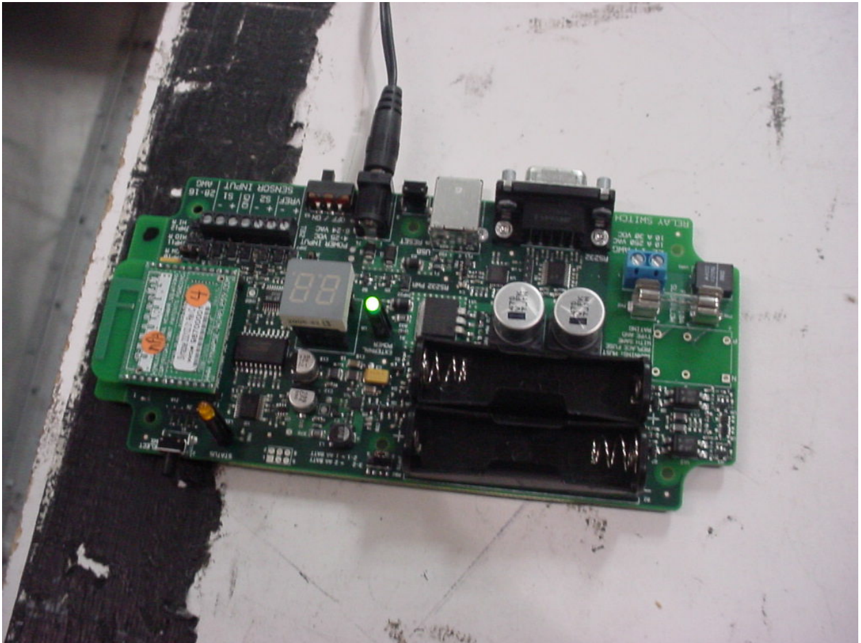
Figure 3: Test Setup – AC Power Line Conducted Emissions
