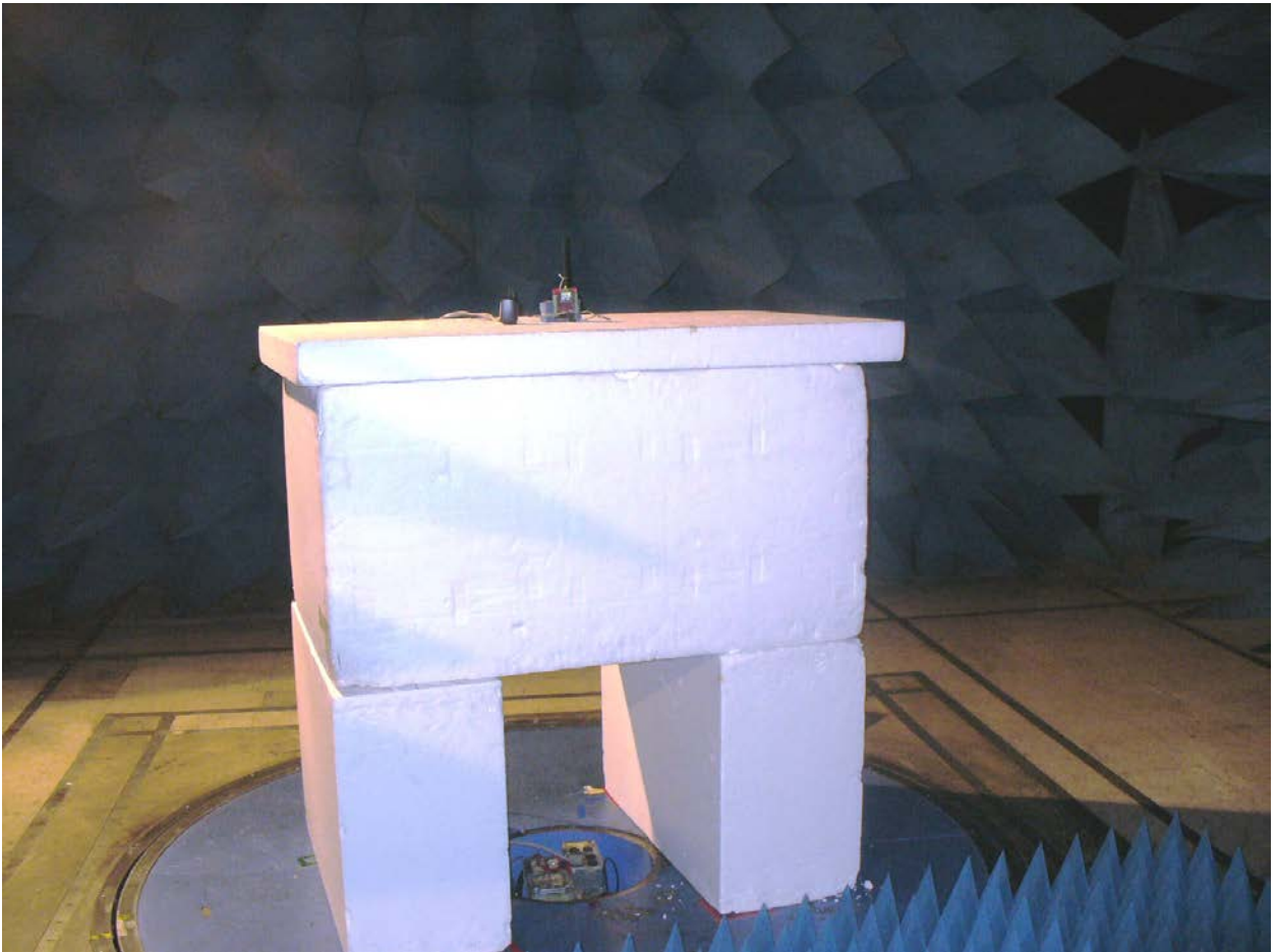
Figure 5: Radiated Emissions – Front View (EUT Standing)
