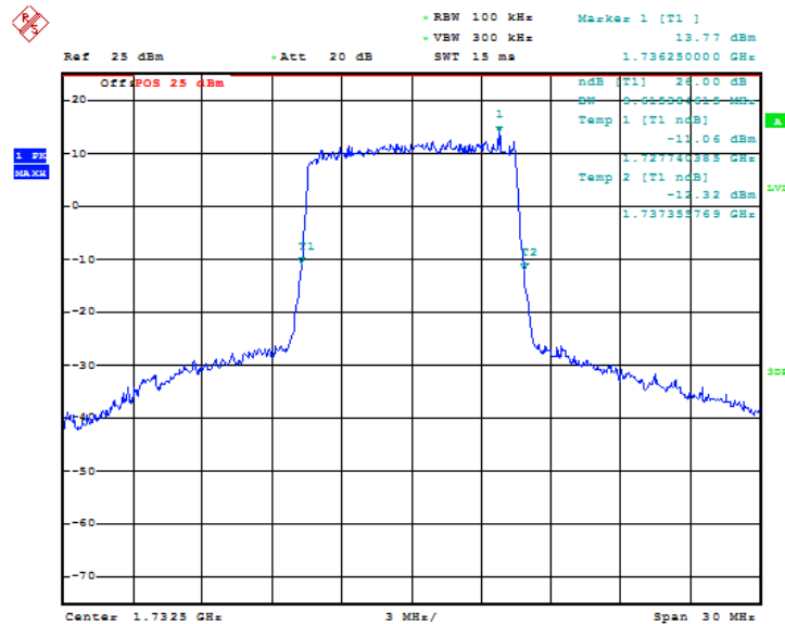
Fig.75 LTE band 4, 10MHz Bandwidth, QPSK (-26dBc BW)
