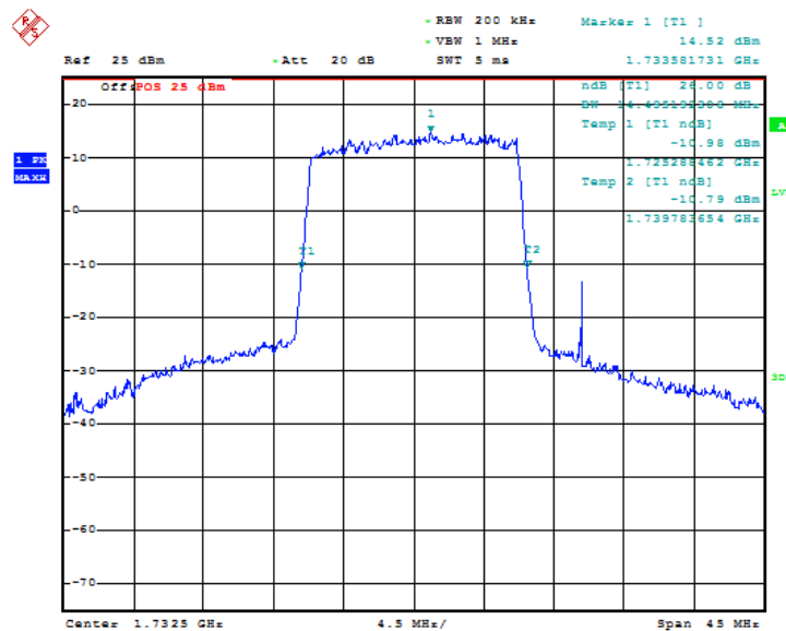
Fig.77 LTE band 4, 15MHz Bandwidth, QPSK (-26dBc BW)
