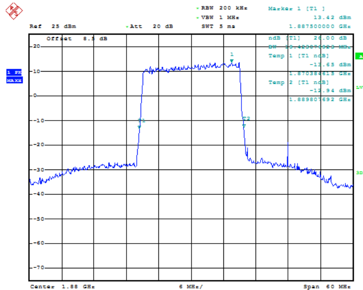
Fig.67 LTE band 2, 20MHz Bandwidth, QPSK (-26dBc BW)
