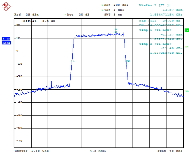
Fig.65 LTE band 2, 15MHz Bandwidth, QPSK (-26dBc BW)
