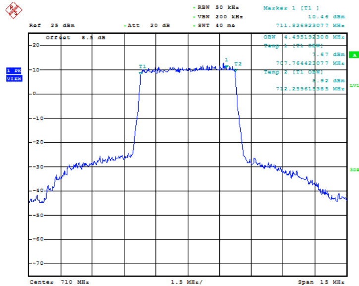
Fig.53 LTE band 17, 5MHz Bandwidth, QPSK (99% BW)
