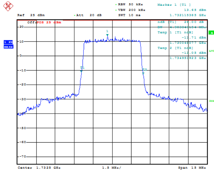
Fig.73 LTE band 4, 5MHz Bandwidth, QPSK (-26dBc BW)
