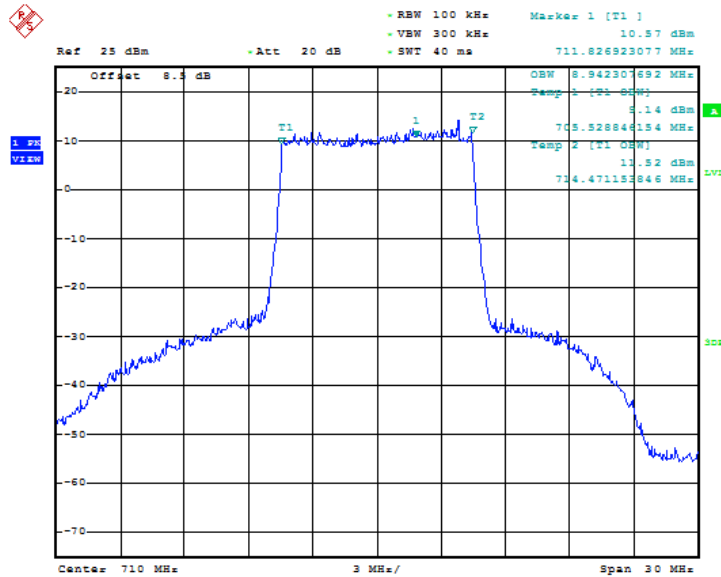
Fig.55 LTE band 17, 10MHz Bandwidth, QPSK (99% BW)
