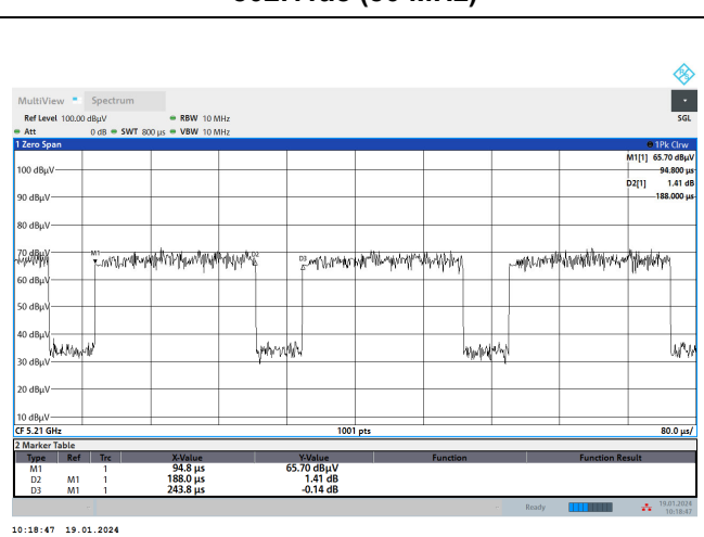
802.11ac (80 MHz)
